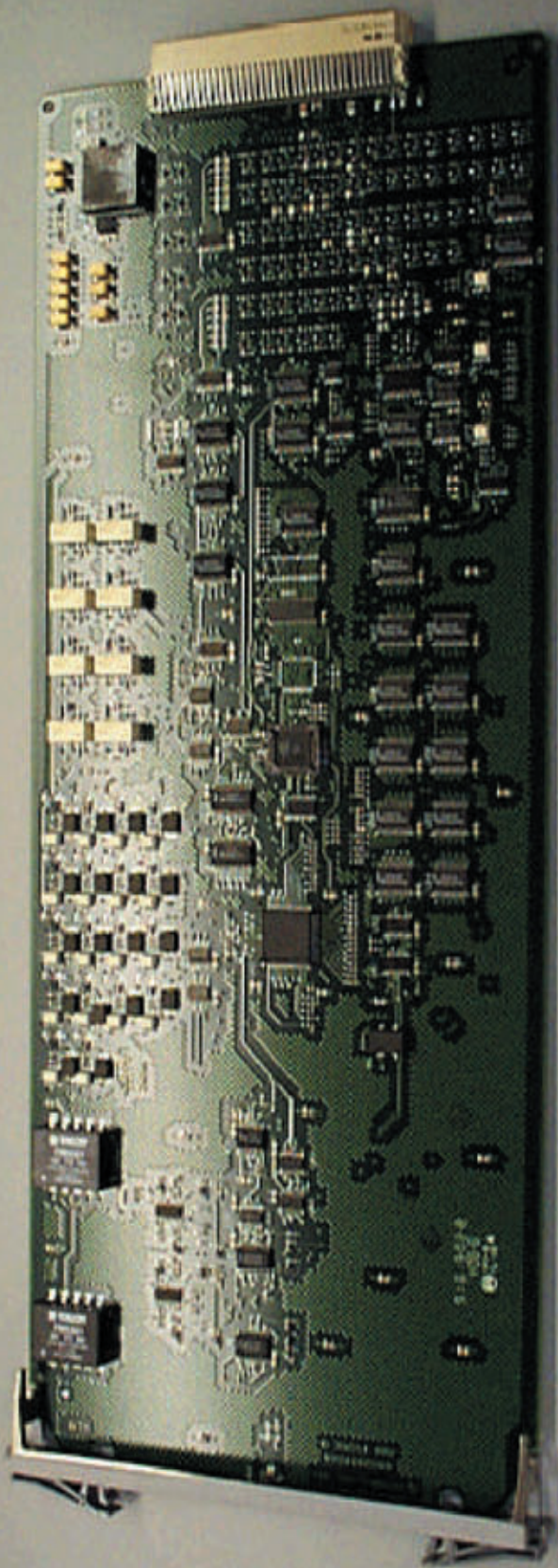
IHET6AP1 SC4812ET 1.9 GHz AMR Front
