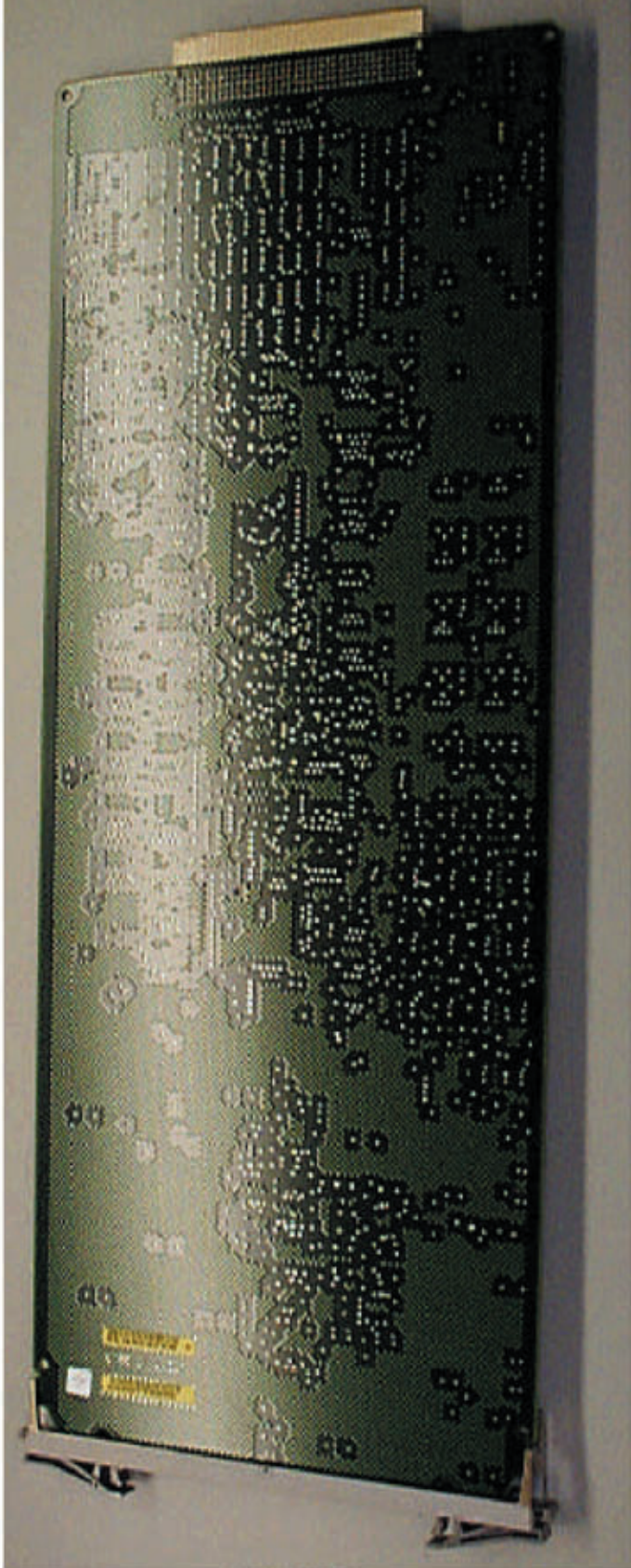
IHET6AP1 SC4812ET 1.9 GHz AMR Back
