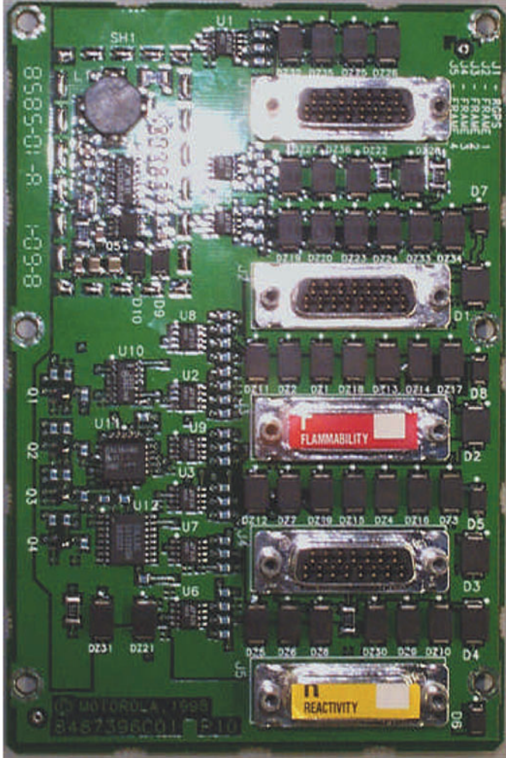
IHE6API SC4812ET 1.9 GHz RGD Front
