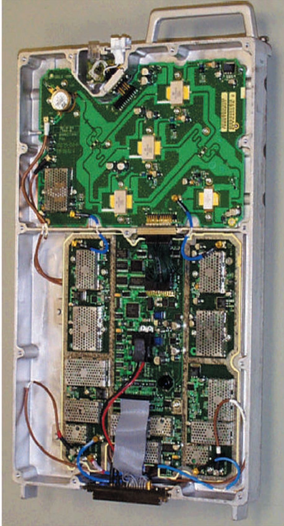
IHET6AP1 SC4812ET 1.9 GHz LPA without Cover
