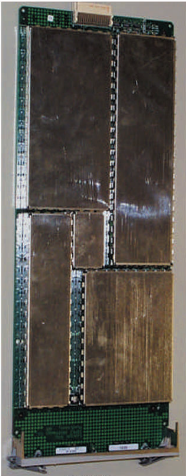
IHET6AP1 SC4812ET 1.9 GHz LFR Front
