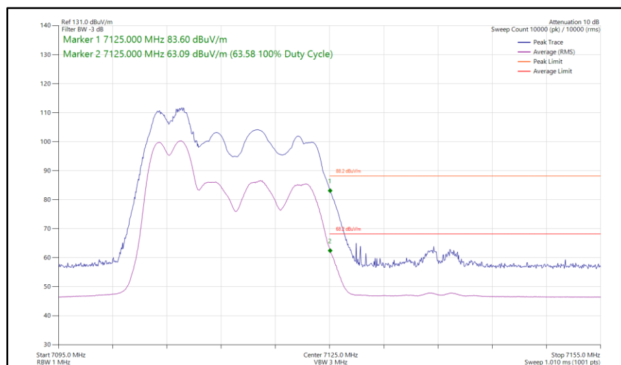
Figure 215 - 802.11ax HE20, RU 52-37, SDM, Core 0 - Core 1 - 7115 MHz Band Edge Frequency 7125 MHz
