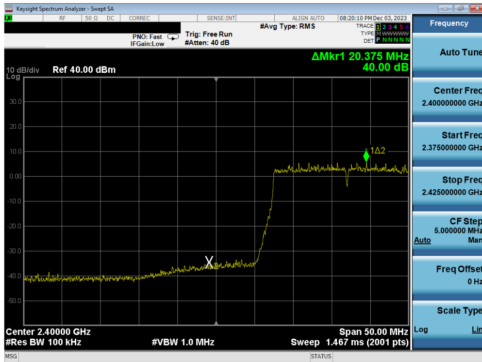
Plot 7-93. Band Edge Antenna WF2b (802.11ax OFDMA – RU242 – Ch. 2)
