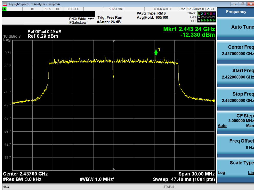
Plot 7-69. Power Spectral Density Plot Antenna WF7b (802.11ax OFDMA – RU242 – Ch. 6)
