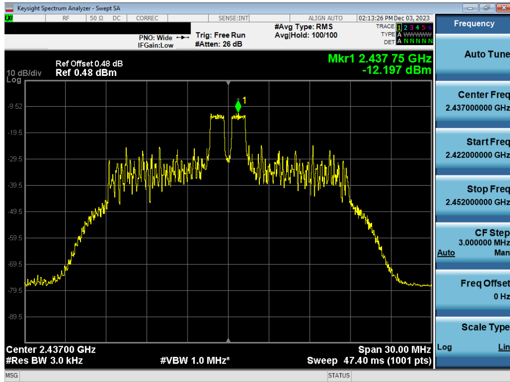
Plot 7-29. Power Spectral Density Plot Antenna WF7b (802.11ax OFDMA – RU26 Index 4 – Ch. 6)
