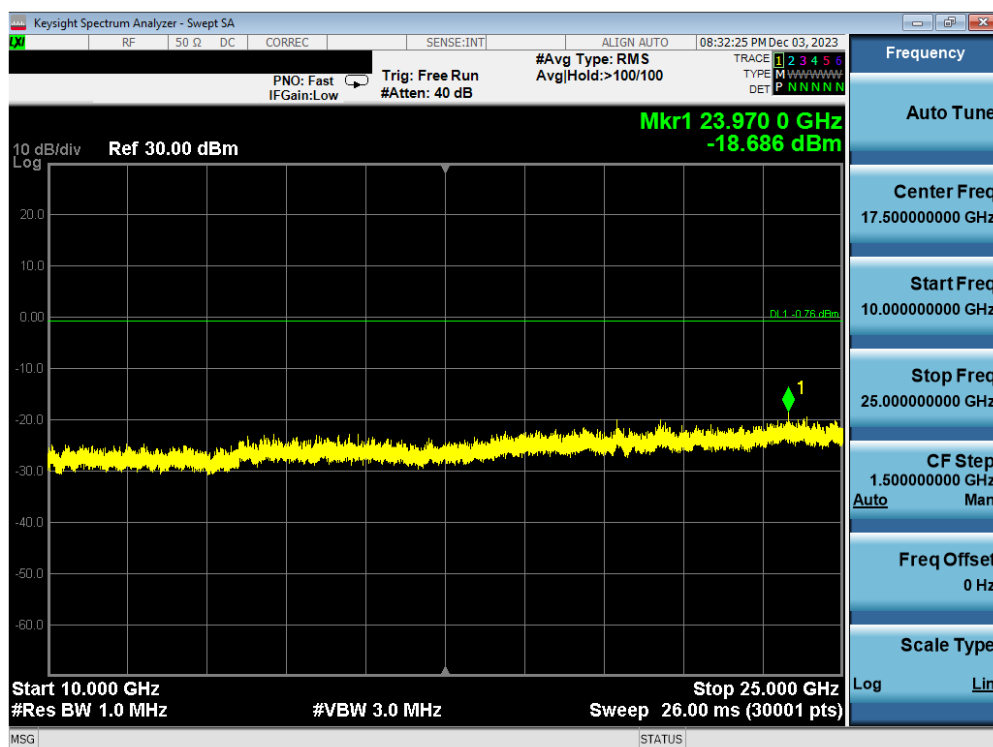
Plot 7-118. Conducted Spurious Plot Antenna WF2b (802.11ax OFDMA – RU26 – Ch. 1)
