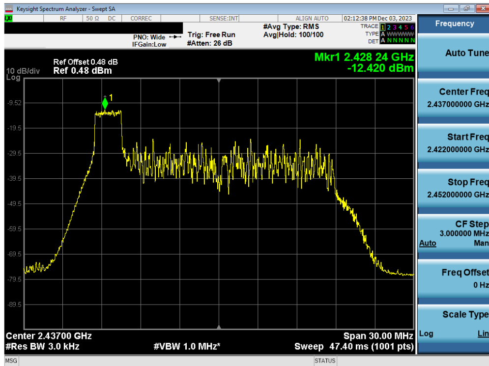
Plot 7-28. Power Spectral Density Plot Antenna WF7b (802.11ax OFDMA – RU26 Index 0 – Ch. 6)
