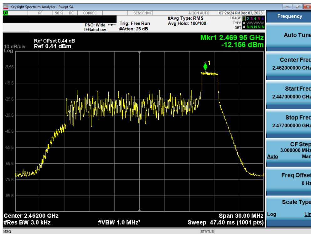
Plot 7-65. Power Spectral Density Plot Antenna WF7b (802.11ax OFDMA – RU26 Index 8 – Ch. 11)
