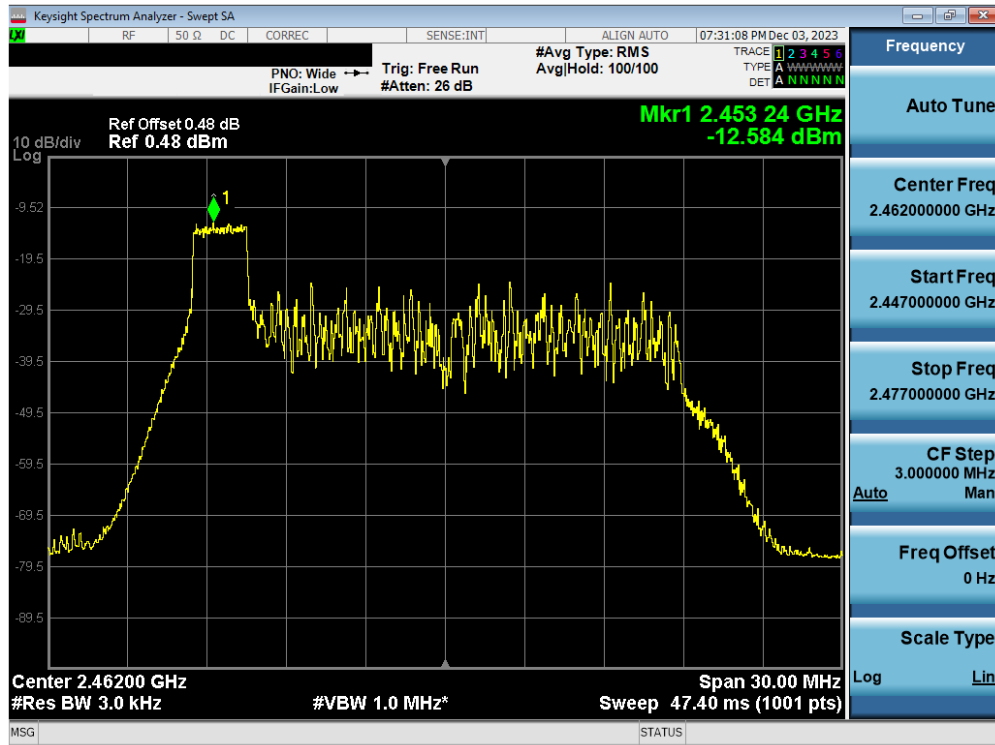
Plot 7-43. Power Spectral Density Plot Antenna WF2b (802.11ax OFDMA – RU26 Index 0 – Ch. 11)
