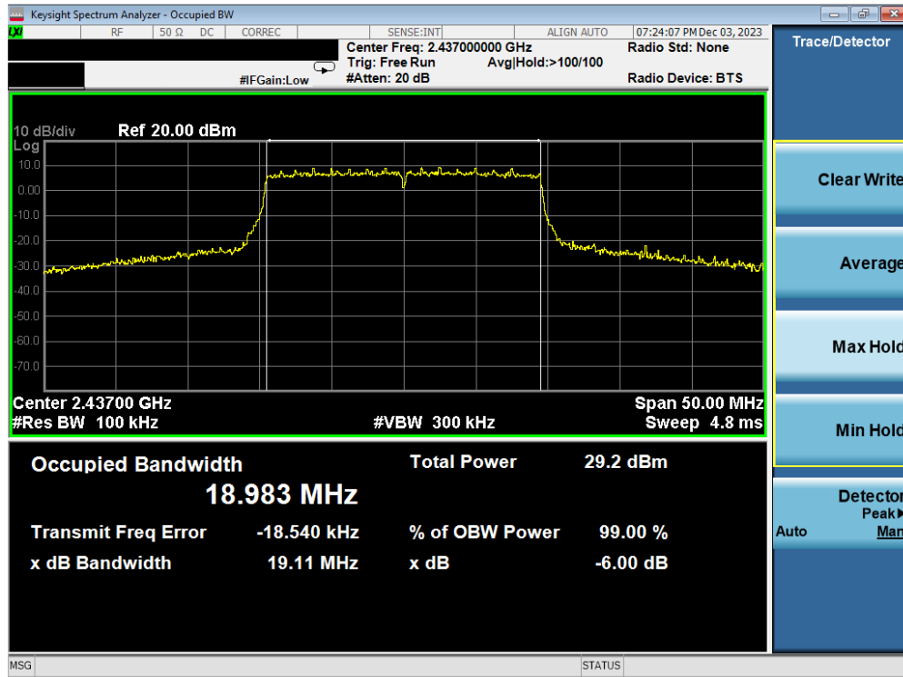
Plot 7-23. 6dB BW & 99% OBW Plot Antenna WF2b (802.11ax OFDMA – RU242 – Ch. 6)
