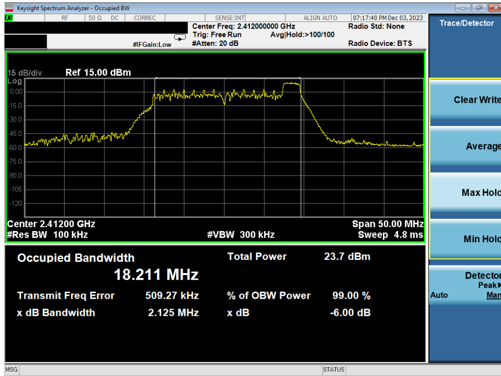
Plot 7-15. 6dB BW & 99% OBW Plot Antenna WF2b (802.11ax OFDMA – RU26 Index 8 – Ch. 1)
