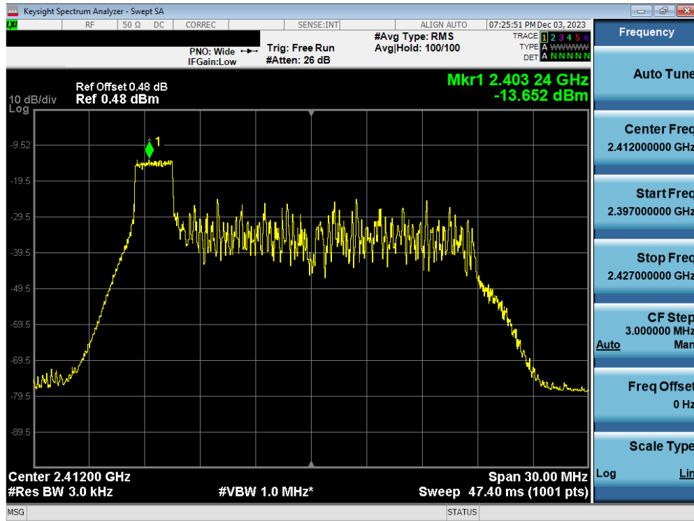
Plot 7-37. Power Spectral Density Plot Antenna WF2b (802.11ax OFDMA – RU26 Index 0 – Ch. 1)
