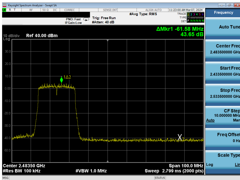
Plot 7-102. Band Edge Antenna WF2b (802.11ax OFDMA – RU242 – Ch. 10)
