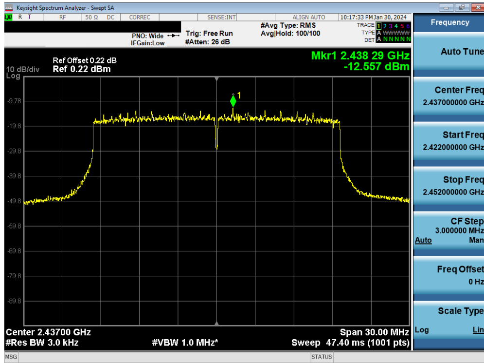
Plot 7-47. Power Spectral Density Plot Antenna WF2b (802.11ax OFDMA – RU242 – Ch. 6)
