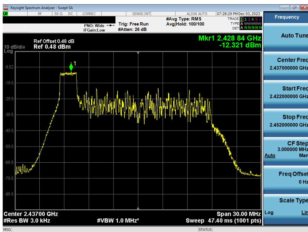
Plot 7-40. Power Spectral Density Plot Antenna WF2b (802.11ax OFDMA – RU26 Index 0 – Ch. 6)
