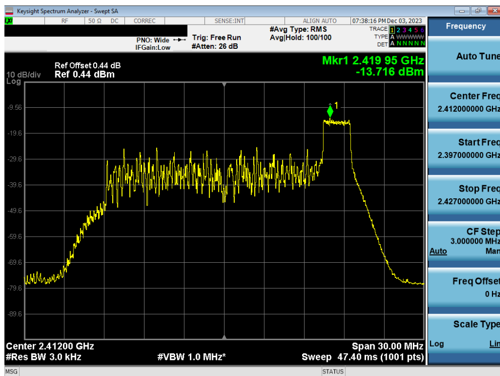
Plot 7-54. Power Spectral Density Plot Antenna WF2b (802.11ax OFDMA – RU26 Index 8 – Ch. 1)
