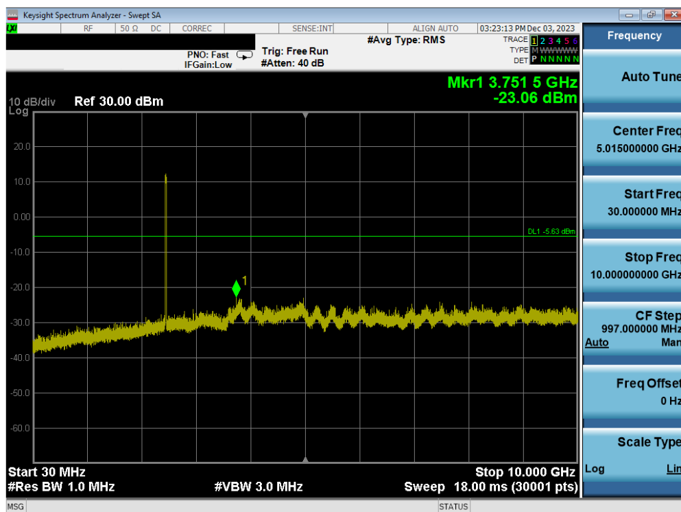
Plot 7-115. Conducted Spurious Plot Antenna WF7b (802.11ax OFDMA – RU242 – Ch. 11)
