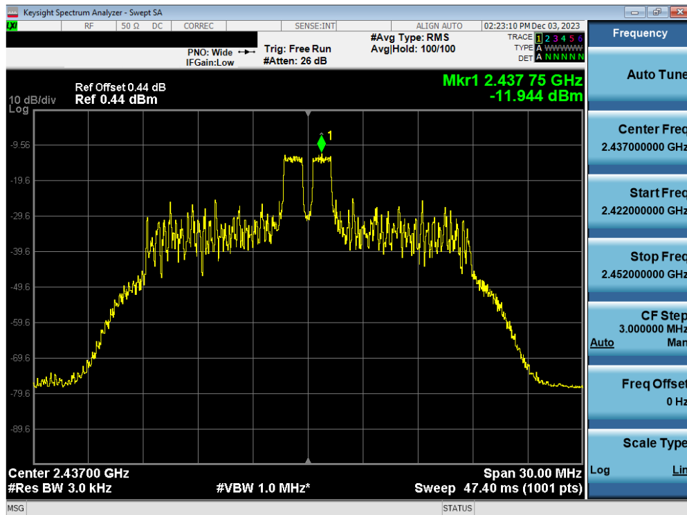
Plot 7-57. Power Spectral Density Plot Antenna WF7b (802.11ax OFDMA – RU26 Index 4 – Ch. 6)
