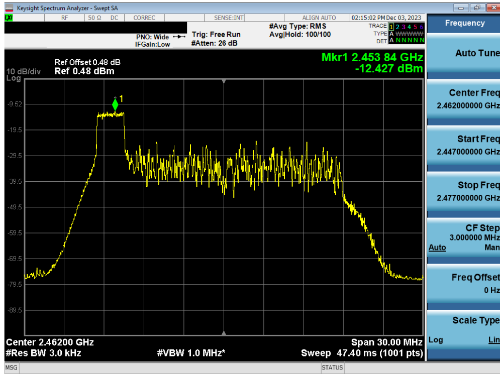
Plot 7-31. Power Spectral Density Plot Antenna WF7b (802.11ax OFDMA – RU26 Index 0 – Ch. 11)
