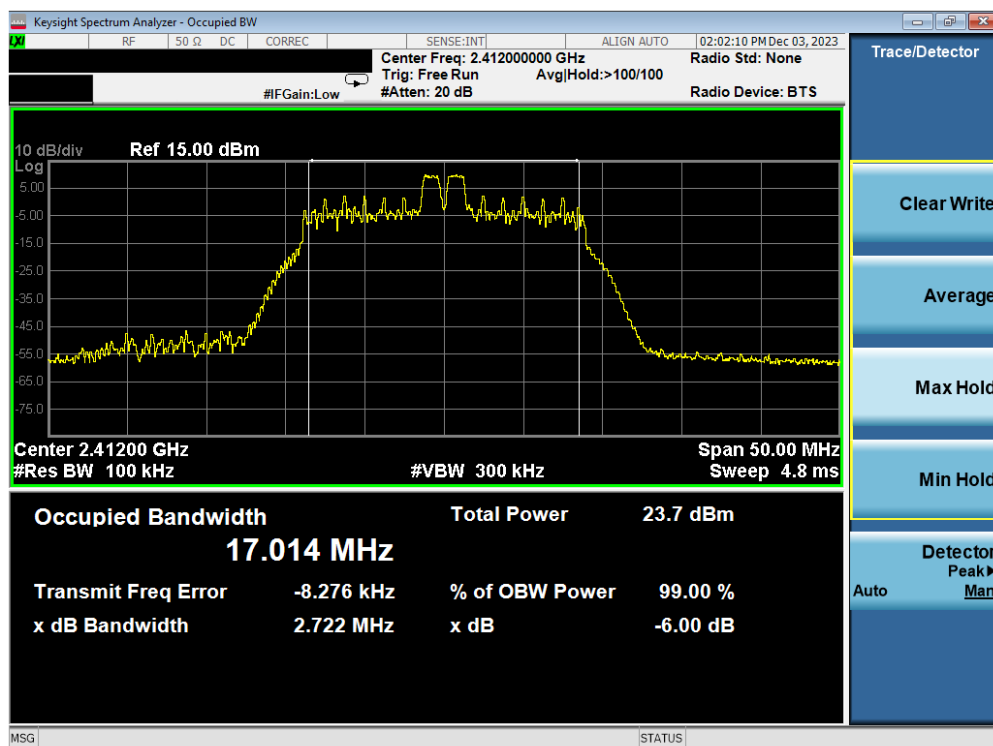
Plot 7-2. 6dB BW & 99% OBW Plot Antenna WF7b (802.11ax OFDMA – RU26 Index 4 – Ch. 1)
