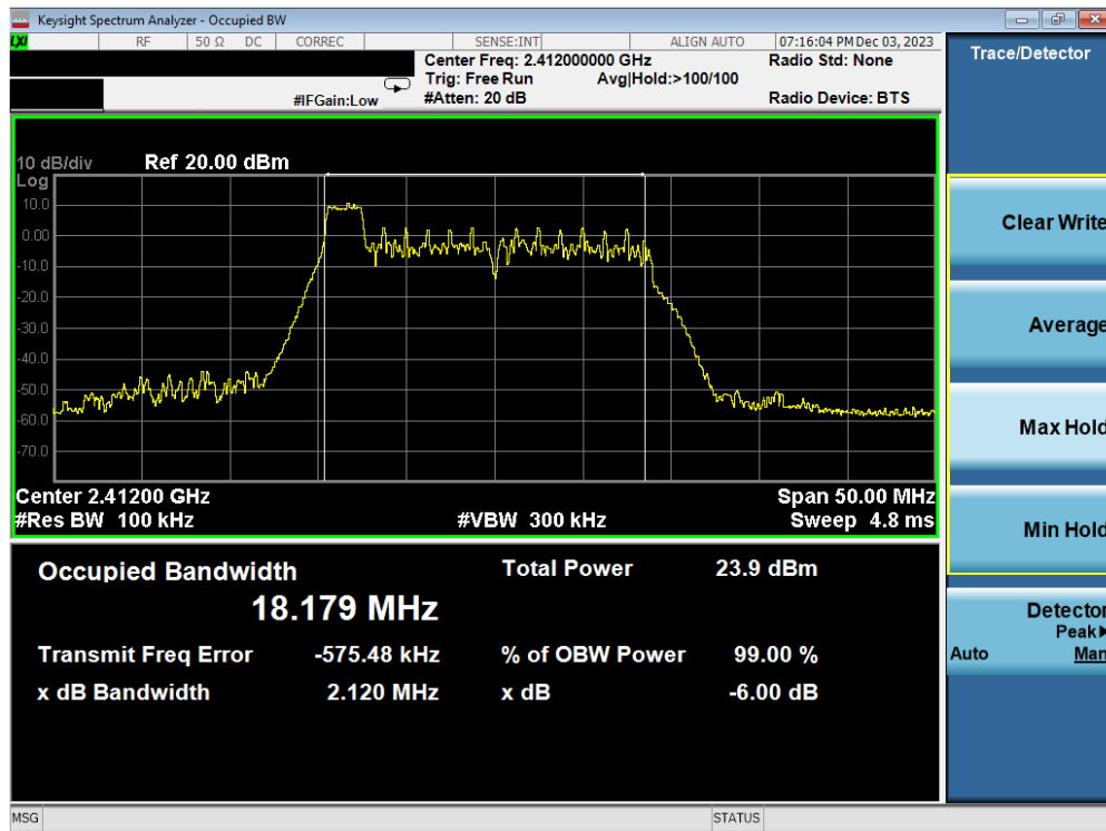
Plot 7-13. 6dB BW & 99% OBW Plot Antenna WF2b (802.11ax OFDMA – RU26 Index 0 – Ch. 1)
