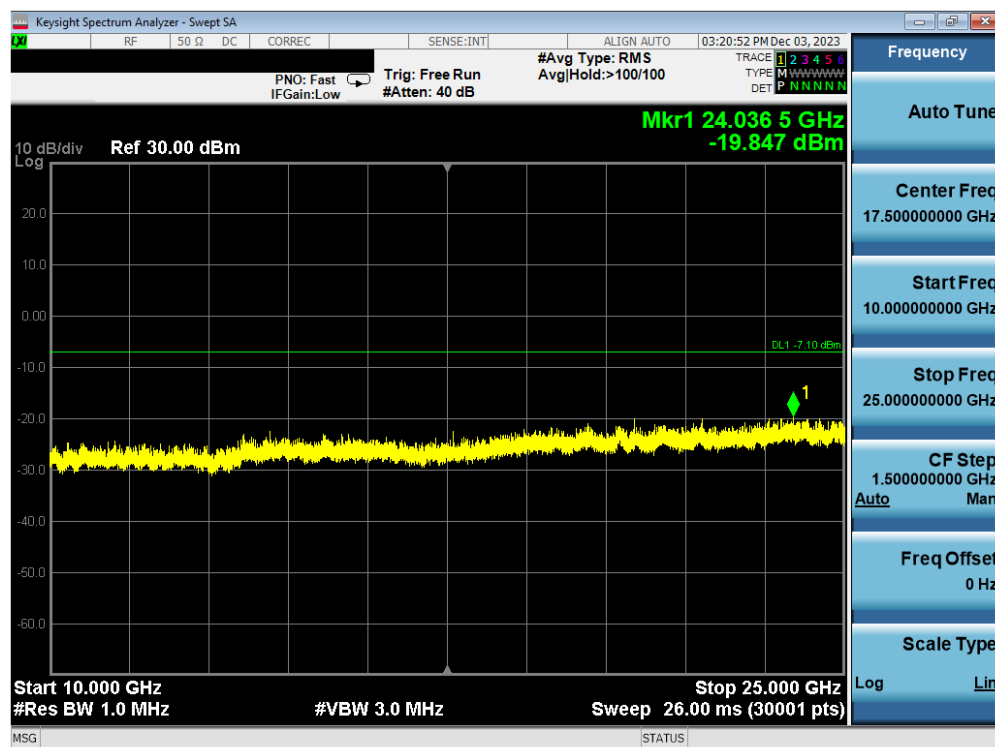
Plot 7-112. Conducted Spurious Plot Antenna WF7b (802.11ax OFDMA – RU242 – Ch. 1)
