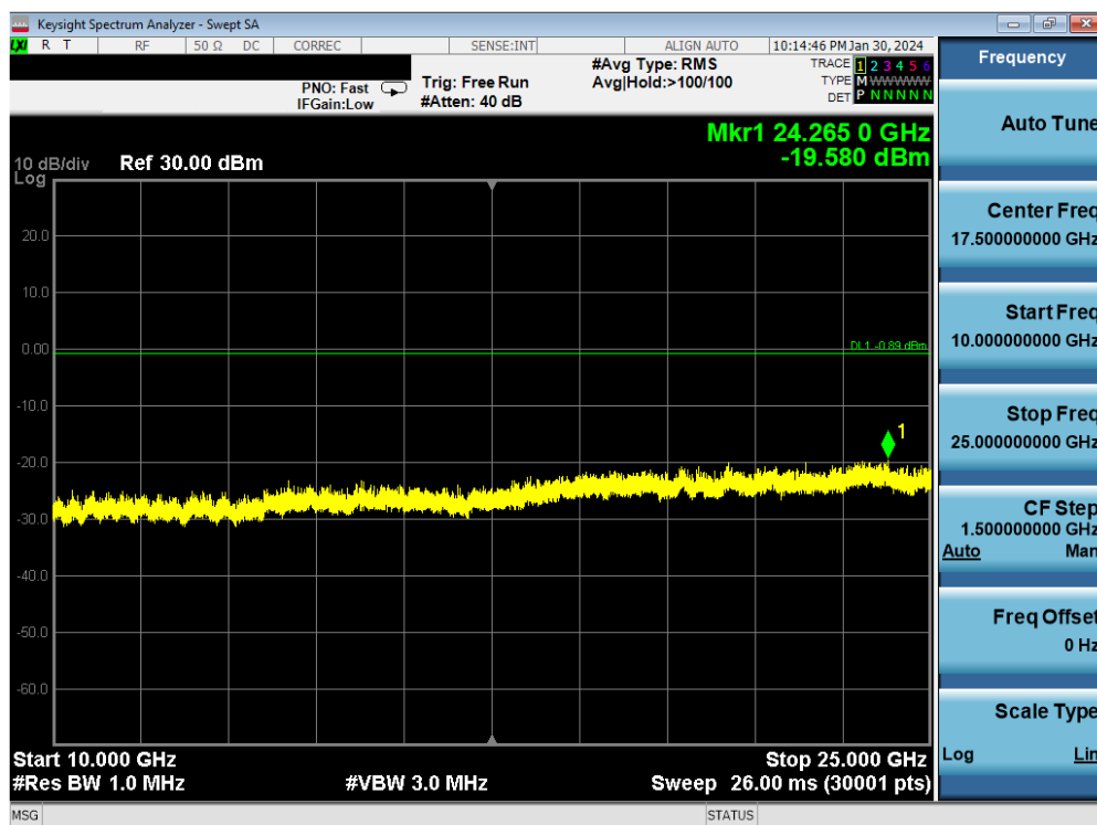
Plot 7-114. Conducted Spurious Plot Antenna WF7b (802.11ax OFDMA – RU242 – Ch. 6)
