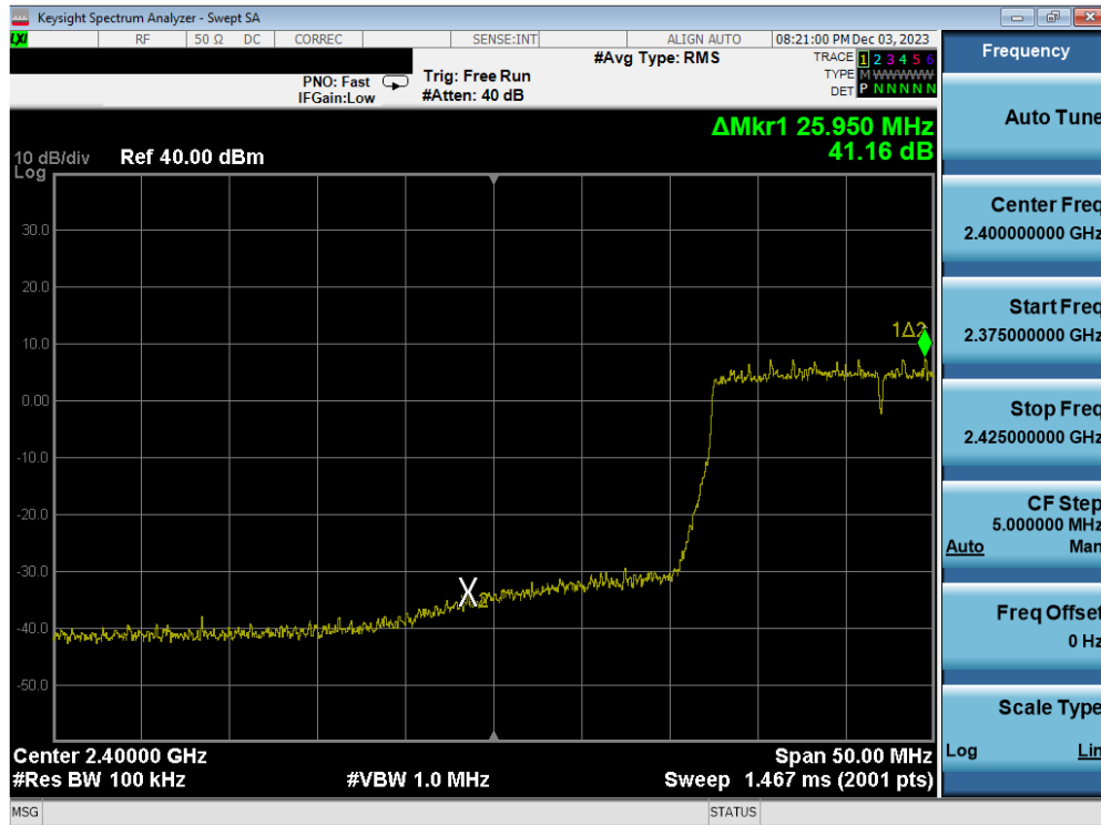
Plot 7-94. Band Edge Antenna WF2b (802.11ax OFDMA – RU242 – Ch. 3)
