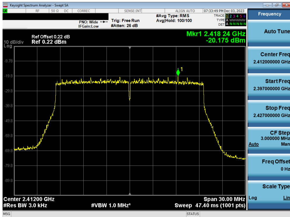
Plot 7-46. Power Spectral Density Plot Antenna WF2b (802.11ax OFDMA – RU242 – Ch. 1)
