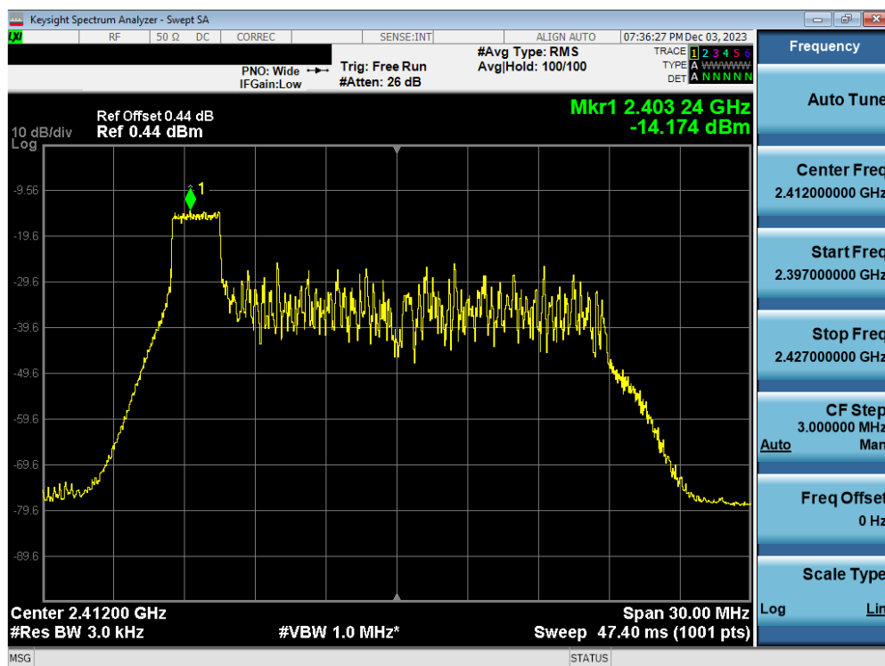
Plot 7-50. Power Spectral Density Plot Antenna WF2b (802.11ax OFDMA – RU26 Index 0 – Ch. 1)
