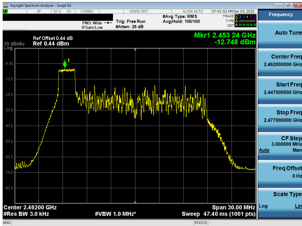
Plot 7-62. Power Spectral Density Plot Antenna WF2b (802.11ax OFDMA – RU26 Index 0 – Ch. 11)
