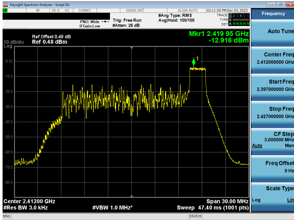
Plot 7-27. Power Spectral Density Plot Antenna WF7b (802.11ax OFDMA – RU26 Index 8 – Ch. 1)
