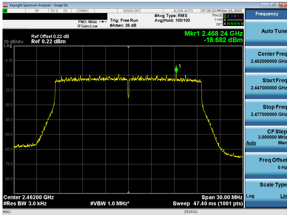
Plot 7-48. Power Spectral Density Plot Antenna WF2b (802.11ax OFDMA – RU242 – Ch. 11)
