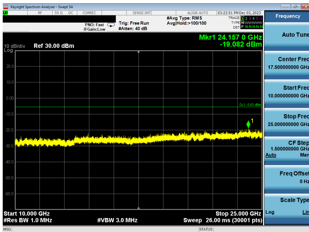
Plot 7-116. Conducted Spurious Plot Antenna WF7b (802.11ax OFDMA – RU242 – Ch. 11)
