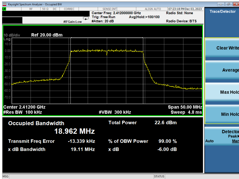
Plot 7-22. 6dB BW & 99% OBW Plot Antenna WF2b (802.11ax OFDMA – RU242 – Ch. 1)
