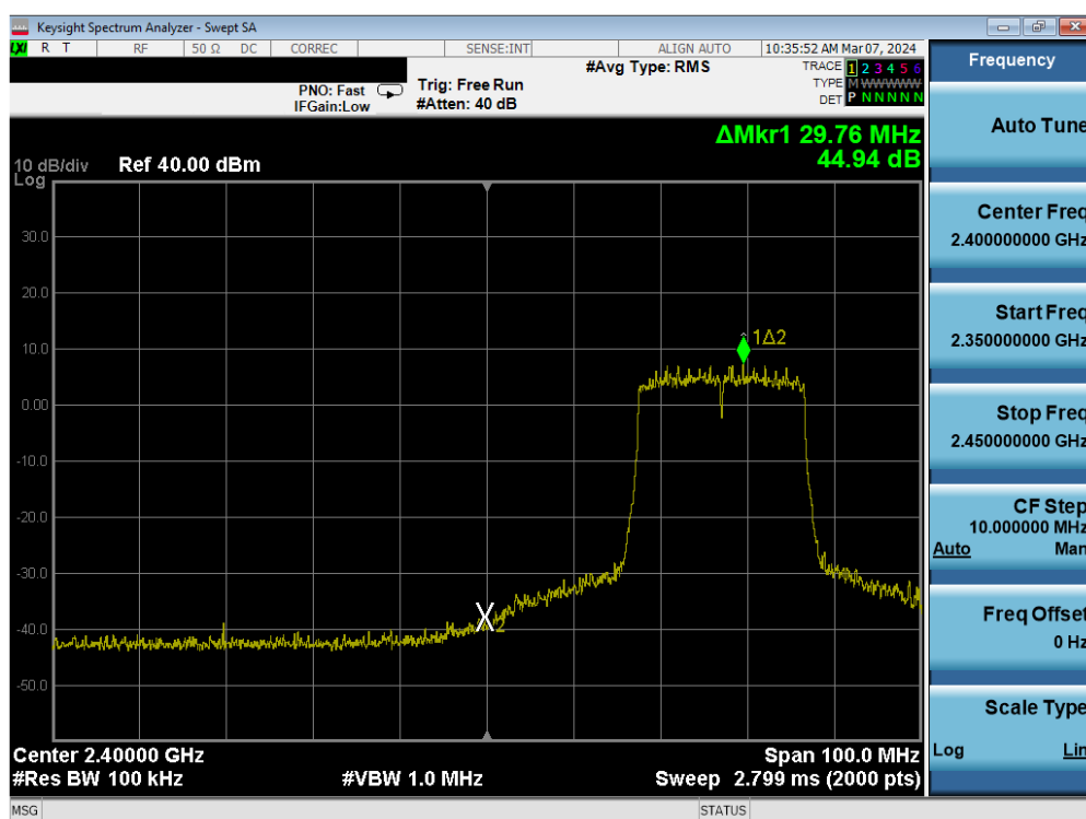
Plot 7-79. Band Edge Antenna WF7b (802.11ax OFDMA – RU242 – Ch. 4)
