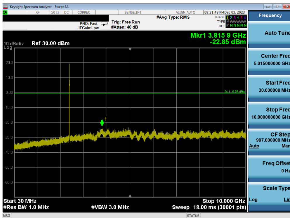
Plot 7-117. Conducted Spurious Plot Antenna WF2b (802.11ax OFDMA – RU26 – Ch. 1)
