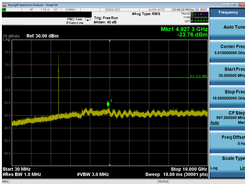
Plot 7-105. Conducted Spurious Plot Antenna WF7b (802.11ax OFDMA – RU26 – Ch. 1)
