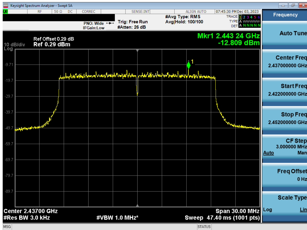
Plot 7-70. Power Spectral Density Plot Antenna WF2b (802.11ax OFDMA – RU242 – Ch. 6)
