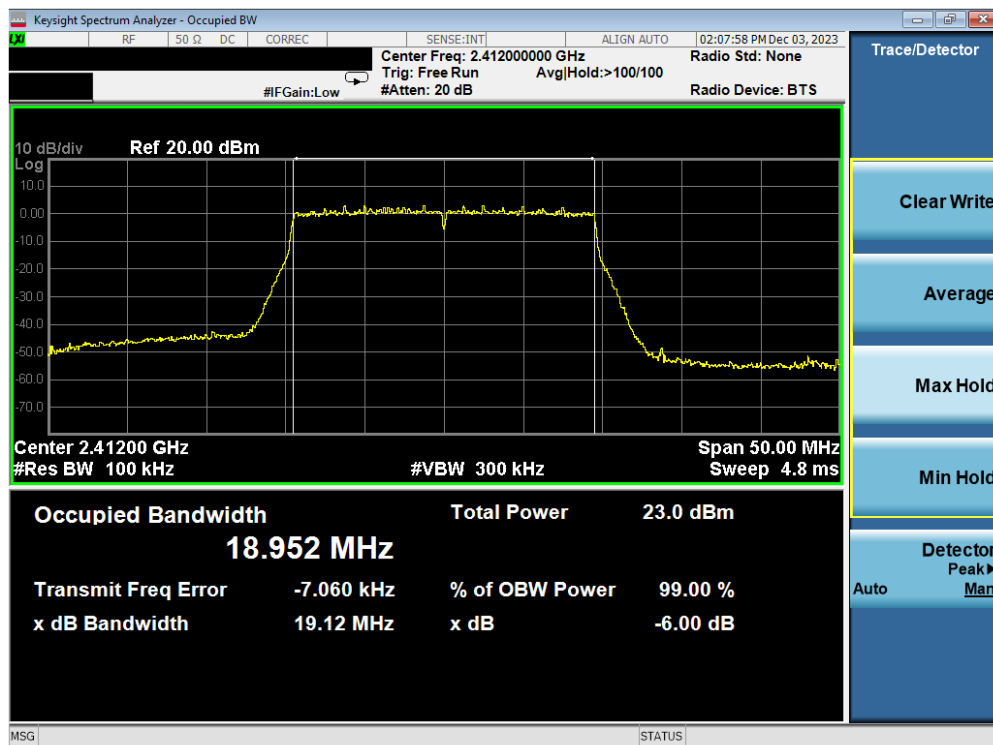
Plot 7-10. 6dB BW & 99% OBW Plot Antenna WF7b (802.11ax OFDMA – RU242 – Ch. 1)
