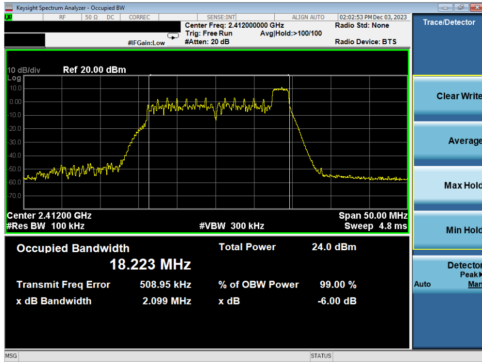
Plot 7-3. 6dB BW & 99% OBW Plot Antenna WF7b (802.11ax OFDMA – RU26 Index 8 – Ch. 1)
