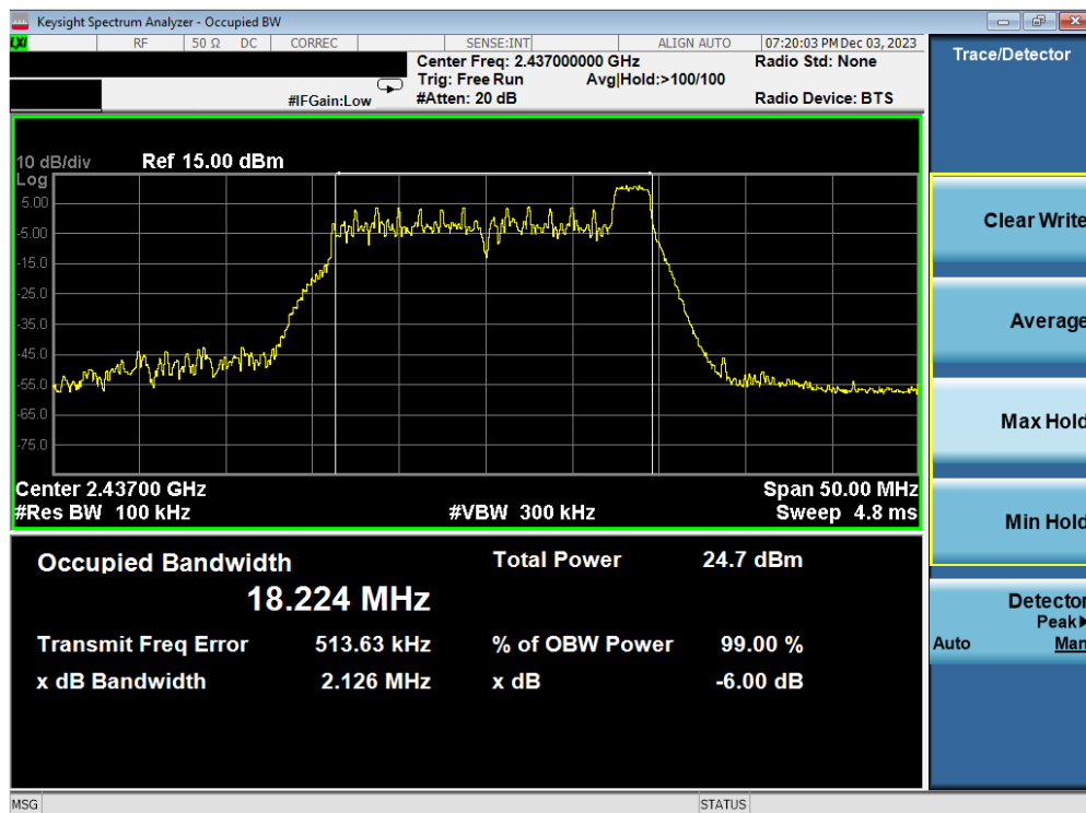
Plot 7-18. 6dB BW & 99% OBW Antenna WF2b (802.11ax OFDMA – RU26 Index 8 – Ch. 6)
