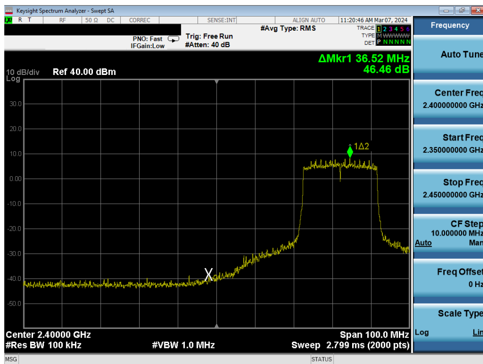
Plot 7-96. Band Edge Antenna WF2b (802.11ax OFDMA – RU242 – Ch. 5)
