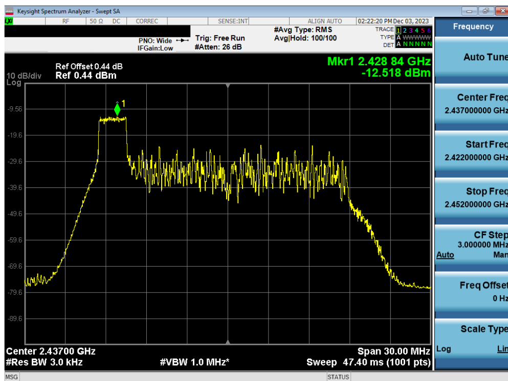
Plot 7-55. Power Spectral Density Plot Antenna WF7b (802.11ax OFDMA – RU26 Index 0 – Ch. 6)
