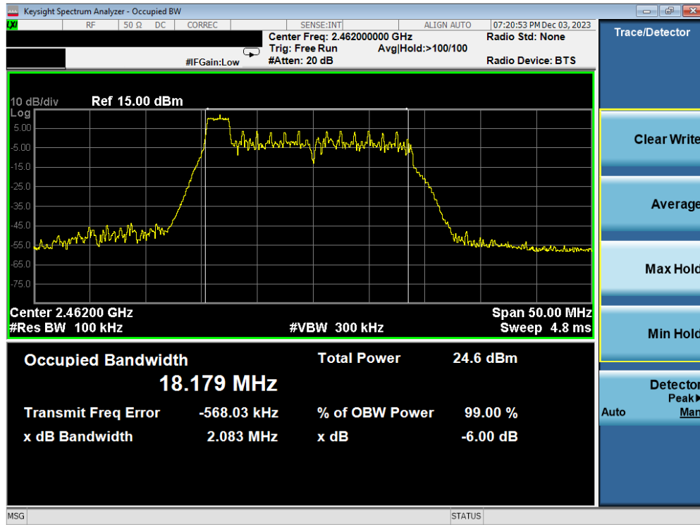
Plot 7-19. 6dB BW & 99% OBW Antenna WF2b (802.11ax OFDMA – RU26 Index 0 – Ch. 11)
