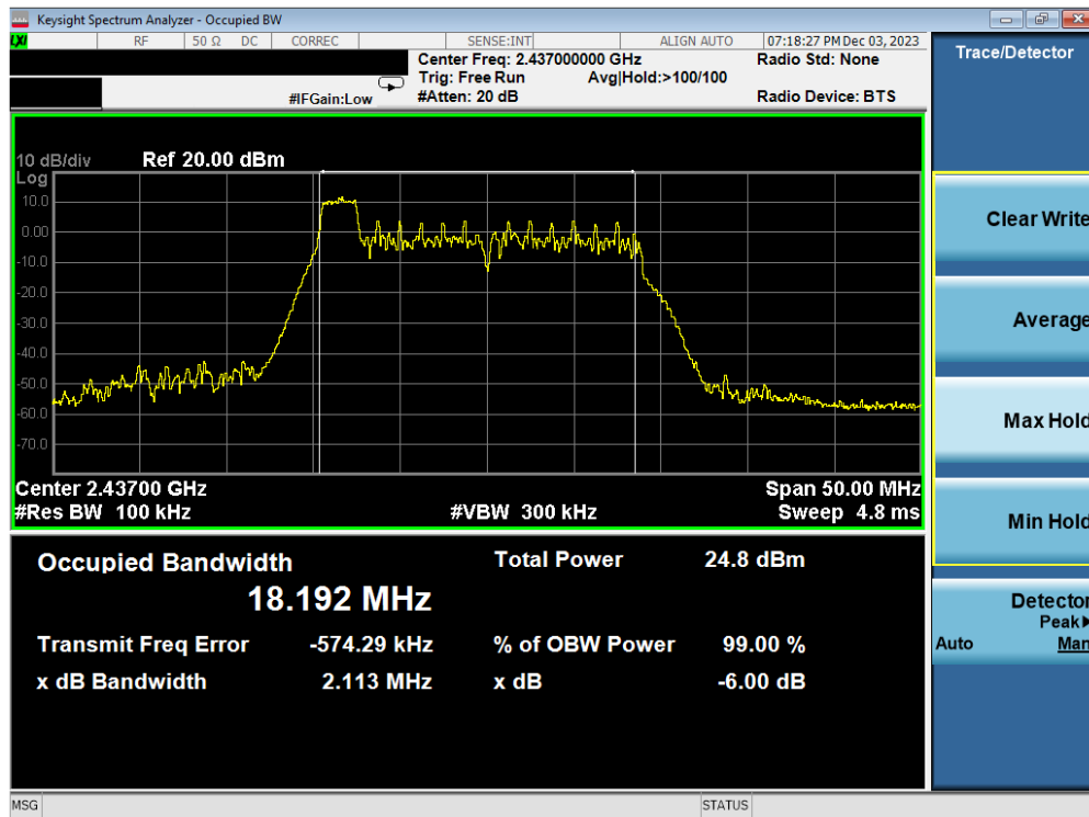
Plot 7-16. 6dB BW & 99% OBW Plot Antenna WF2b (802.11ax OFDMA – RU26 Index 0 – Ch. 6)
