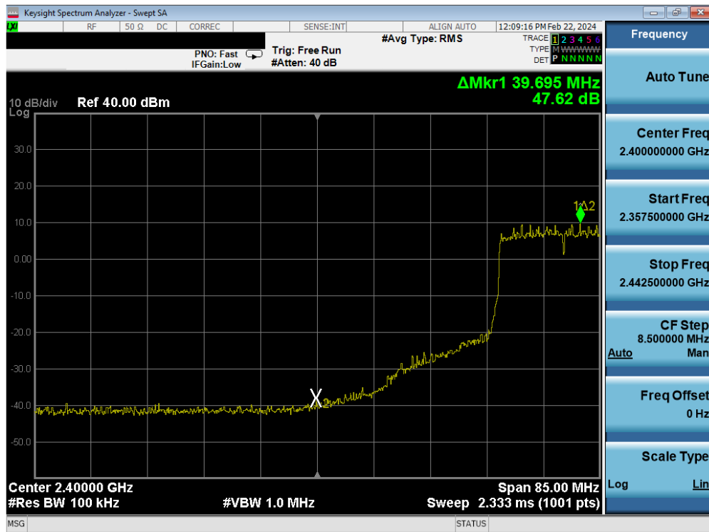
Plot 7-81. Band Edge Antenna WF7b (802.11ax OFDMA – RU242 – Ch. 6(low))
