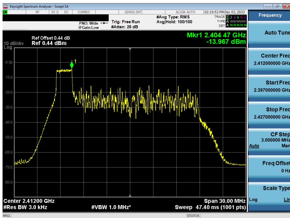
Plot 7-49. Power Spectral Density Plot Antenna WF7b (802.11ax OFDMA – RU26 Index 0 – Ch. 1)
