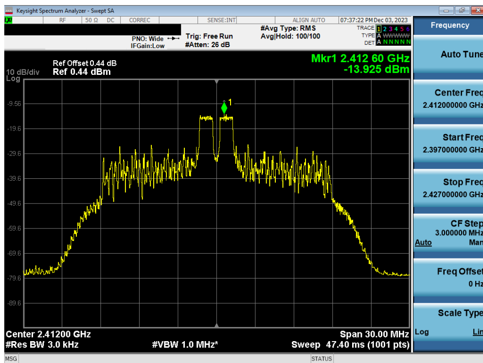
Plot 7-52. Power Spectral Density Plot Antenna WF2b (802.11ax OFDMA – RU26 Index 4 – Ch. 1)
