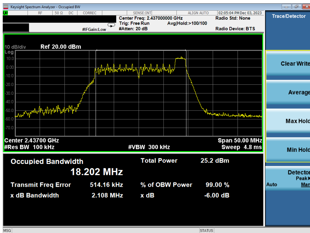
Plot 7-6. 6dB BW & 99% OBW Antenna WF7b (802.11ax OFDMA – RU26 Index 8 – Ch. 6)
