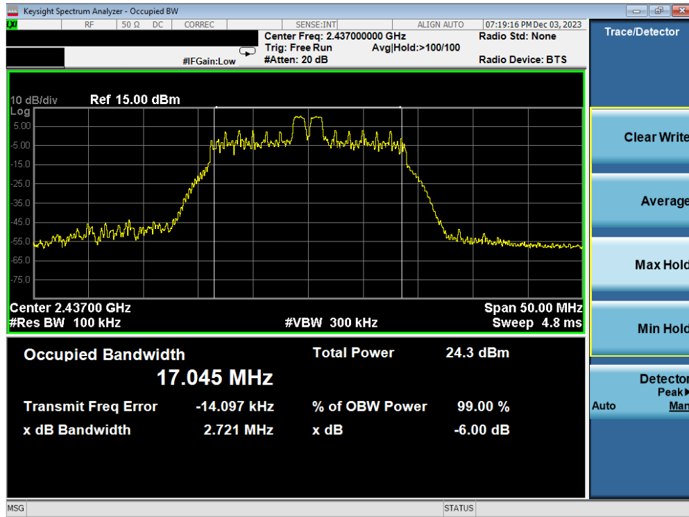
Plot 7-17. 6dB BW & 99% OBW Plot Antenna WF2b (802.11ax OFDMA – RU26 Index 4 – Ch. 6)
