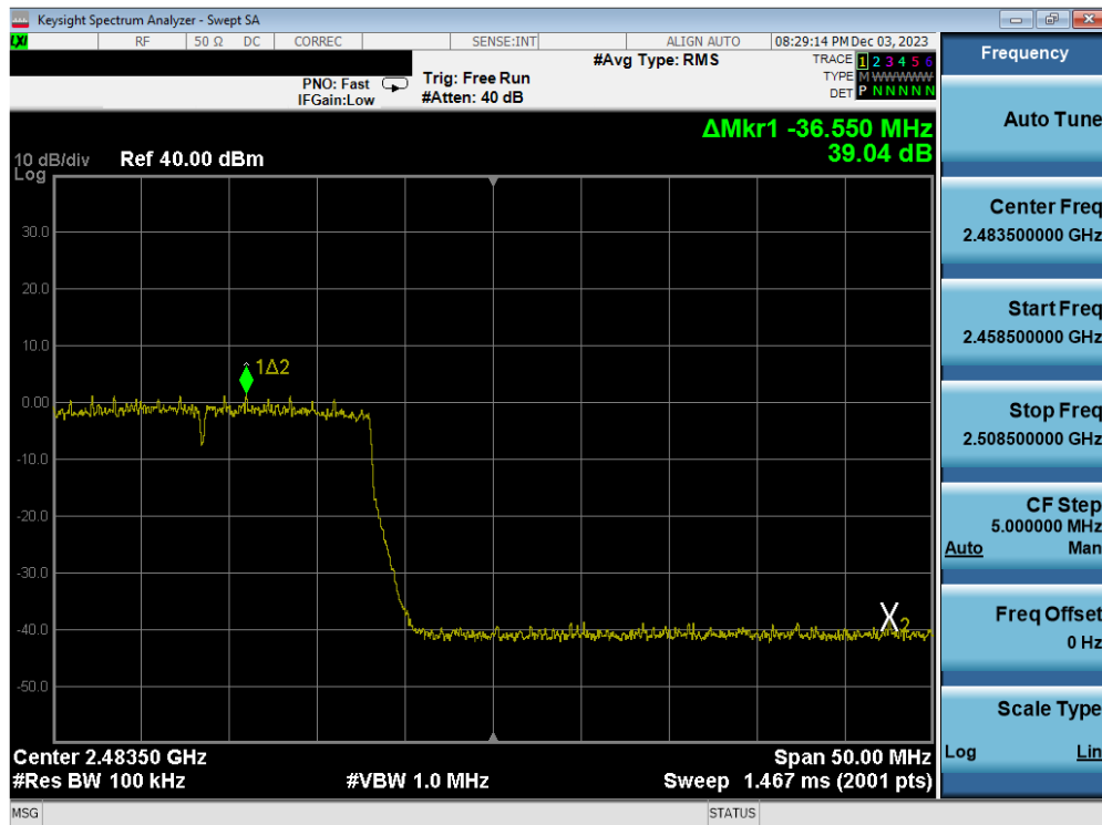
Plot 7-104. Band Edge Antenna WF2b (802.11ax OFDMA – RU242 – Ch. 12)
