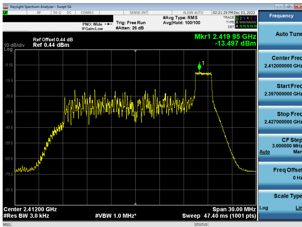
Plot 7-53. Power Spectral Density Plot Antenna WF7b (802.11ax OFDMA – RU26 Index 8 – Ch. 1)
