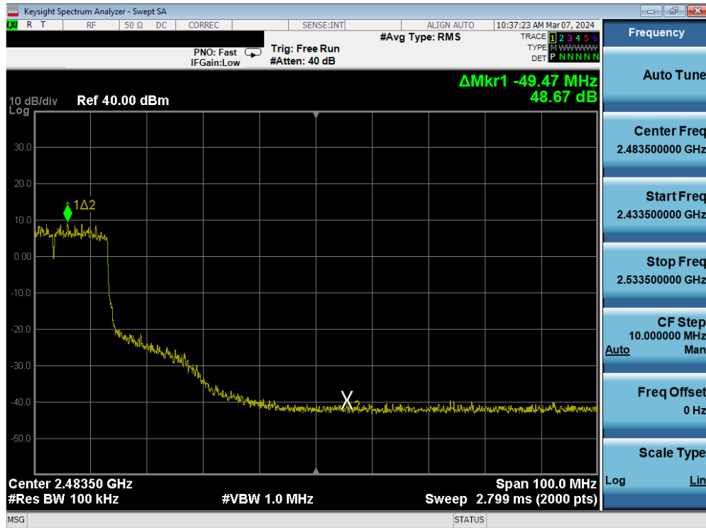
Plot 7-82. Band Edge Antenna WF7b (802.11ax OFDMA – RU242 – Ch. 6(high))
