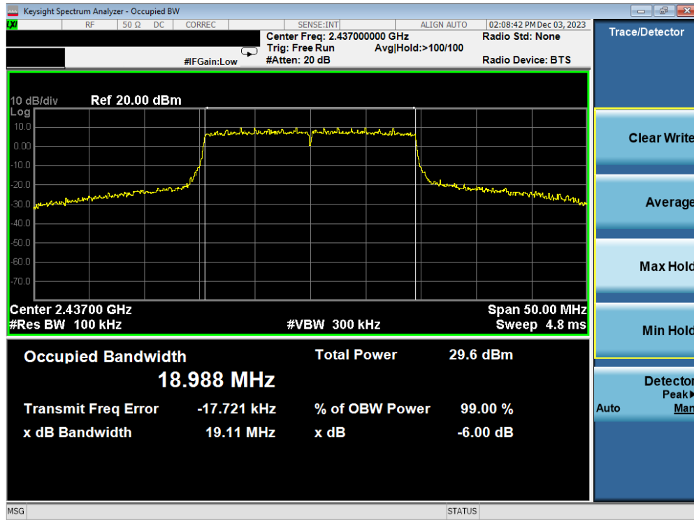
Plot 7-11. 6dB BW & 99% OBW Plot Antenna WF7b (802.11ax OFDMA – RU242 – Ch. 6)
