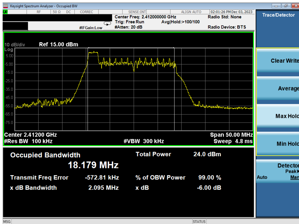
Plot 7-1. 6dB BW & 99% OBW Plot Antenna WF7b (802.11ax OFDMA – RU26 Index 0 – Ch. 1)
