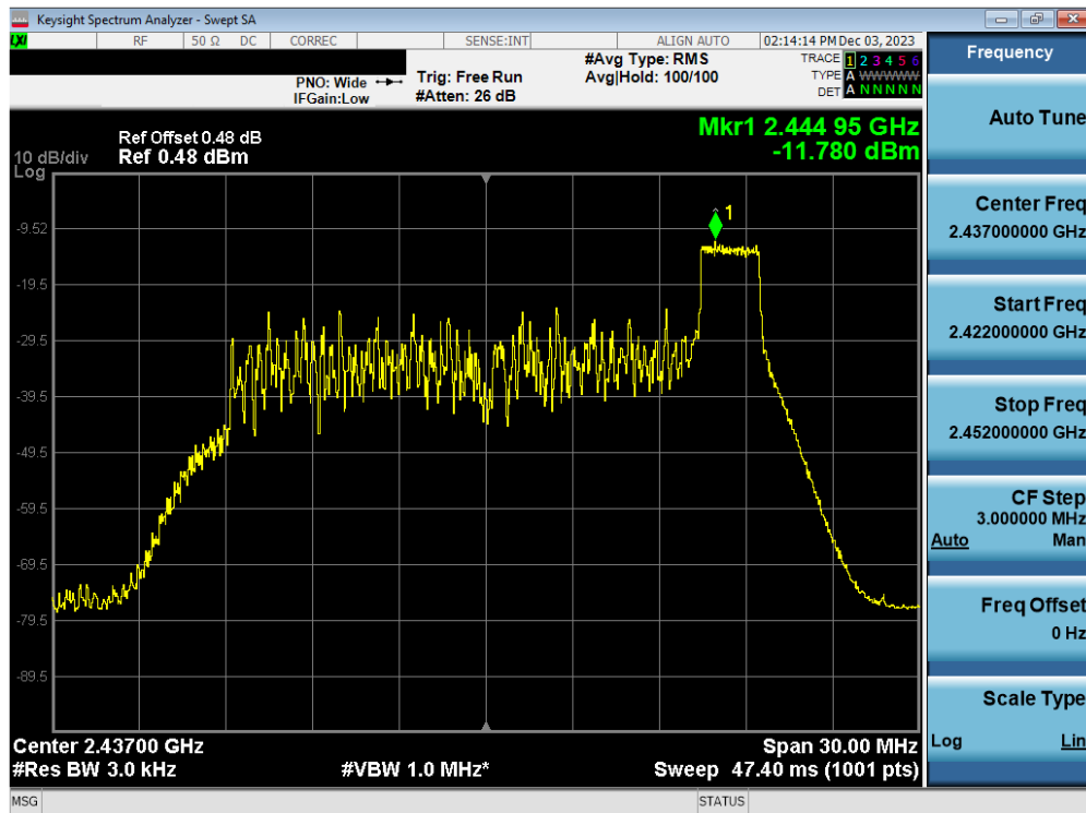
Plot 7-30. Power Spectral Density Plot Antenna WF7b (802.11ax OFDMA – RU26 Index 8 – Ch. 6)
