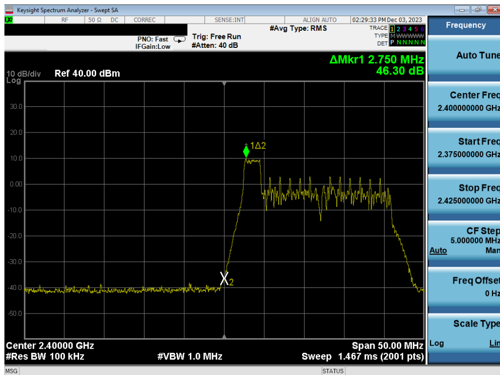
Plot 7-73. Band Edge Antenna WF7b (802.11ax OFDMA – RU26 Index 0 – Ch. 1)
