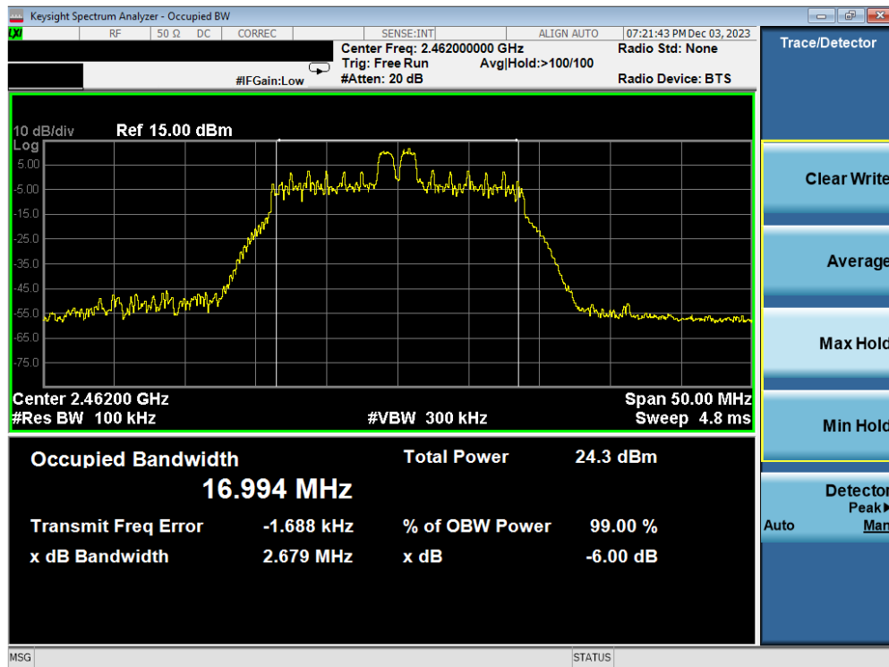
Plot 7-20. 6dB BW & 99% OBW Antenna WF2b (802.11ax OFDMA – RU26 Index 4 – Ch. 11)
