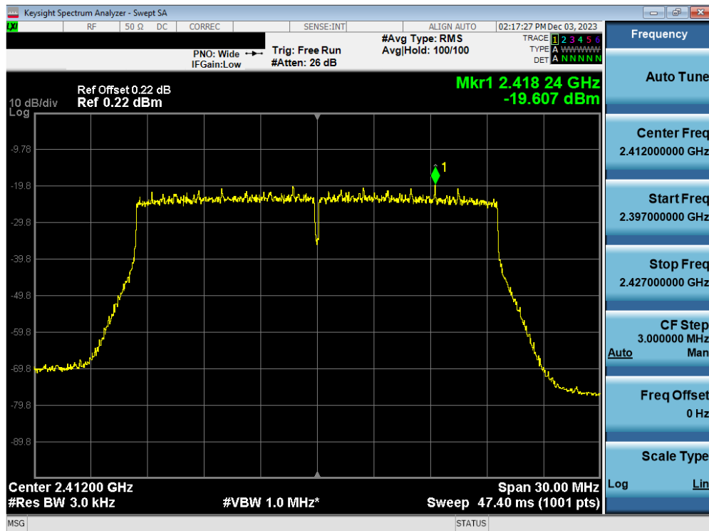
Plot 7-34. Power Spectral Density Plot Antenna WF7b (802.11ax OFDMA – RU242 – Ch. 1)
