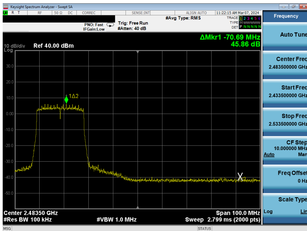
Plot 7-101. Band Edge Antenna WF2b (802.11ax OFDMA – RU242 – Ch. 9)
