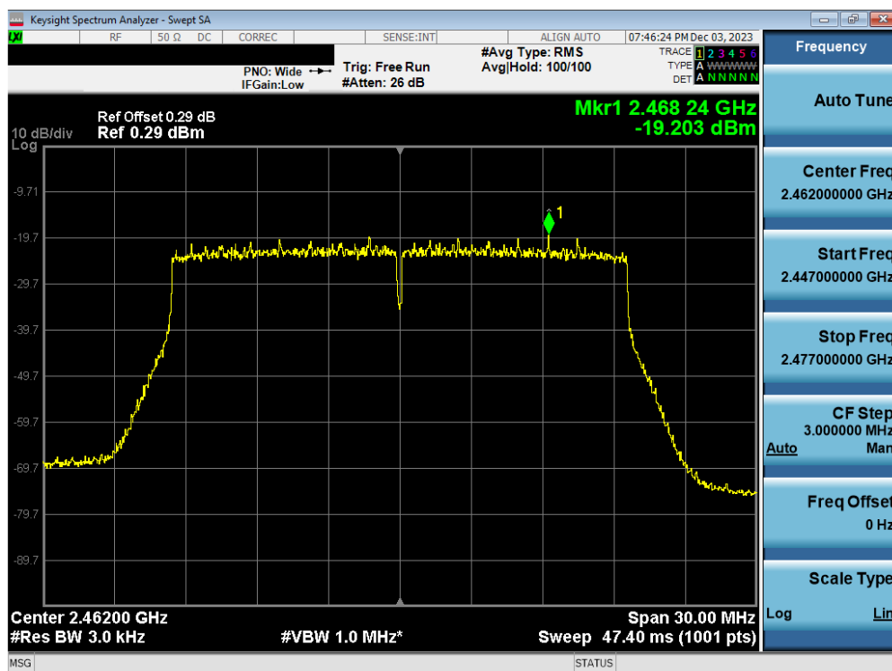
Plot 7-72. Power Spectral Density Plot Antenna WF2b (802.11ax OFDMA – RU242 – Ch. 11)
