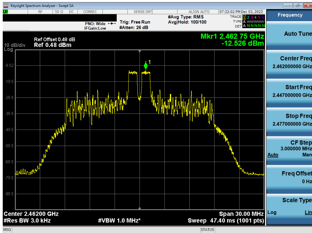
Plot 7-44. Power Spectral Density Plot Antenna WF2b (802.11ax OFDMA – RU26 Index 4 – Ch. 11)
