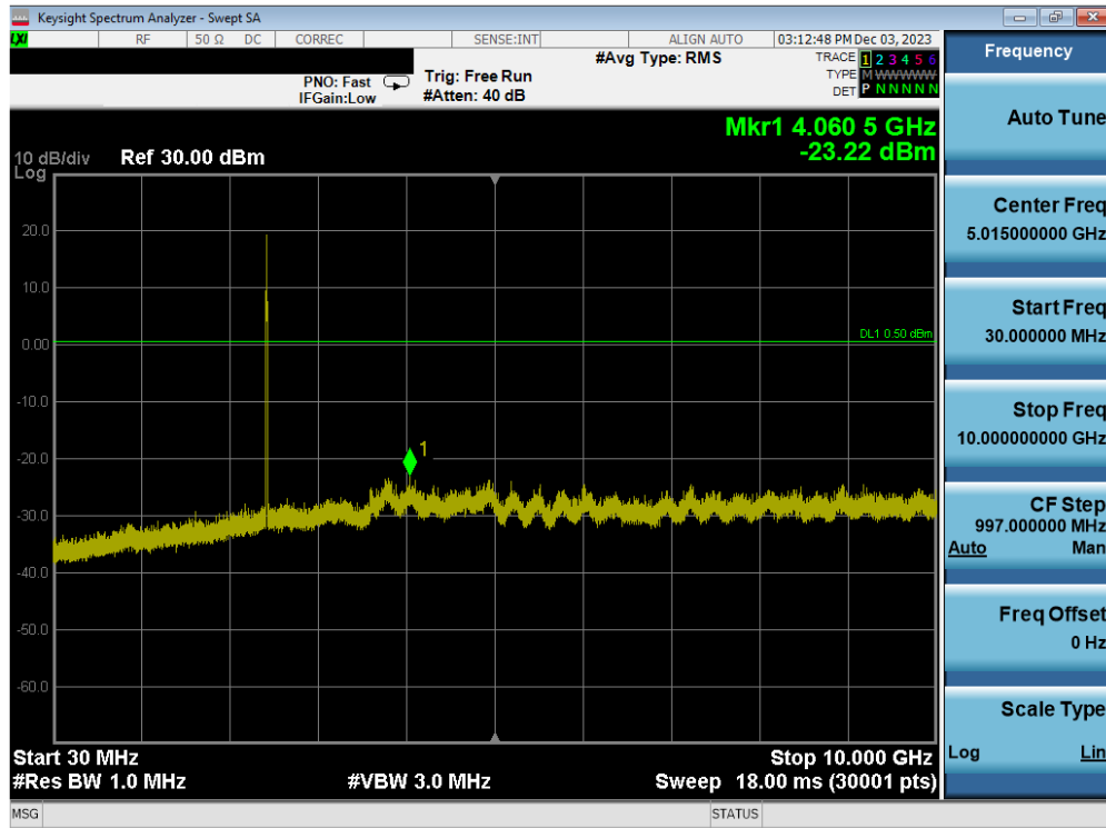
Plot 7-107. Conducted Spurious Plot Antenna WF7b (802.11ax OFDMA – RU26 – Ch. 6)
