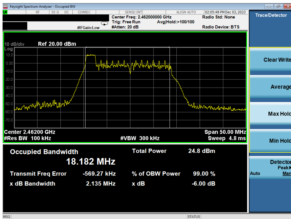
Plot 7-7. 6dB BW & 99% OBW Antenna WF7b (802.11ax OFDMA – RU26 Index 0 – Ch. 11)
