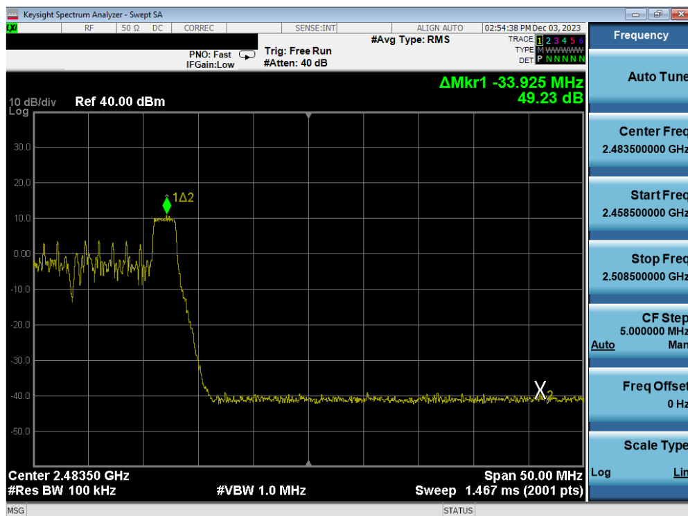
Plot 7-74. Band Edge Antenna WF7b (802.11ax OFDMA – RU26 Index 8 – Ch. 11)
