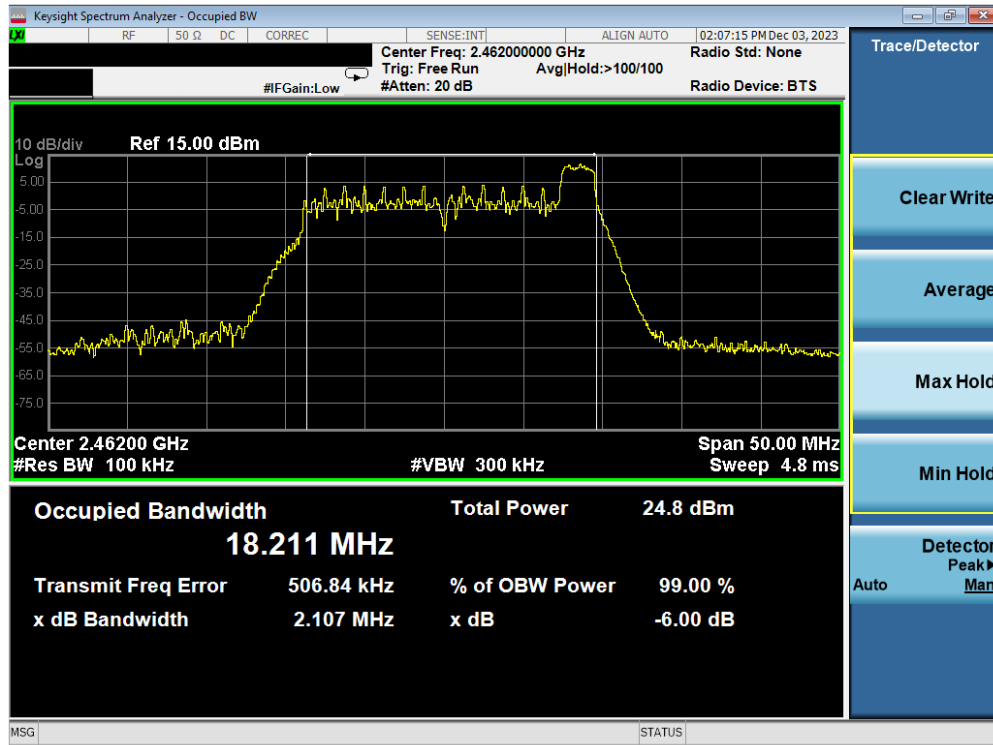
Plot 7-9. 6dB BW & 99% OBW Plot Antenna WF7b (802.11ax OFDMA – RU26 Index 8 – Ch. 11)
