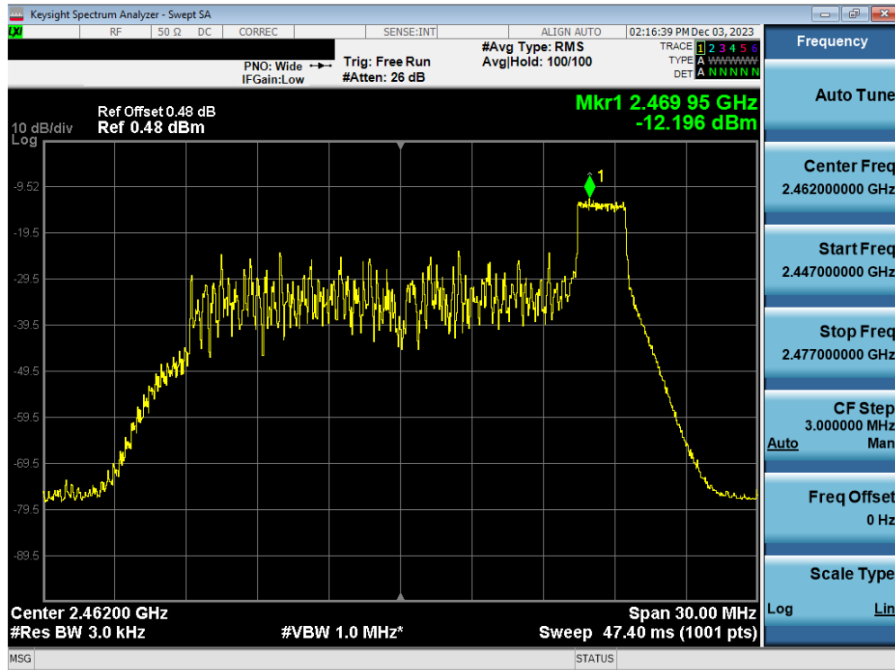
Plot 7-33. Power Spectral Density Plot Antenna WF7b (802.11ax OFDMA – RU26 Index 8 – Ch. 11)
