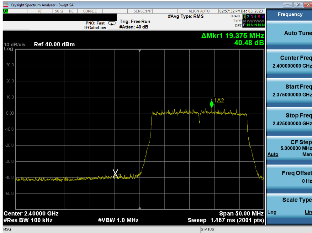
Plot 7-76. Band Edge Antenna WF7b (802.11ax OFDMA – RU242 – Ch. 1)
