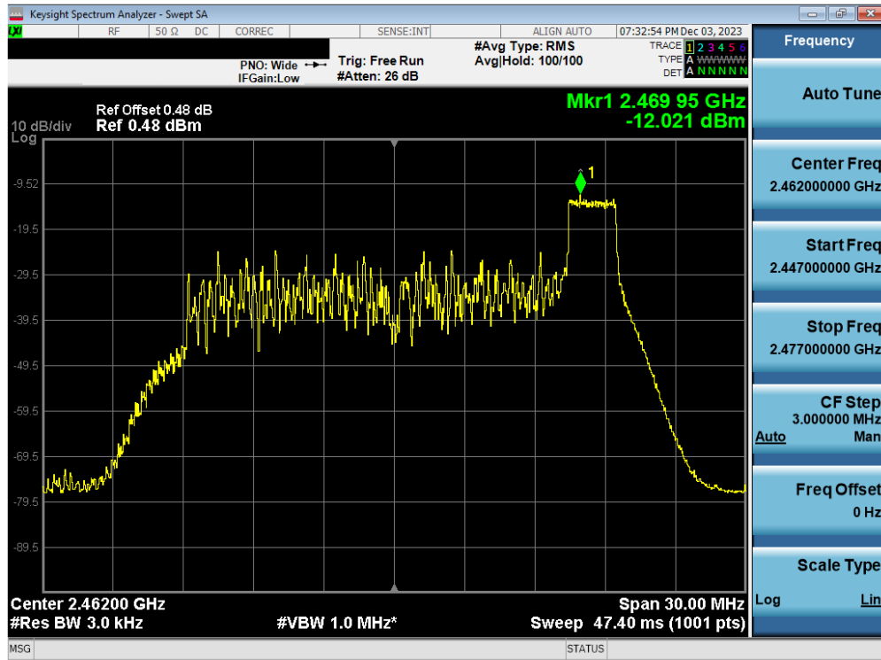
Plot 7-45. Power Spectral Density Plot Antenna WF2b (802.11ax OFDMA – RU26 Index 8 – Ch. 11)
