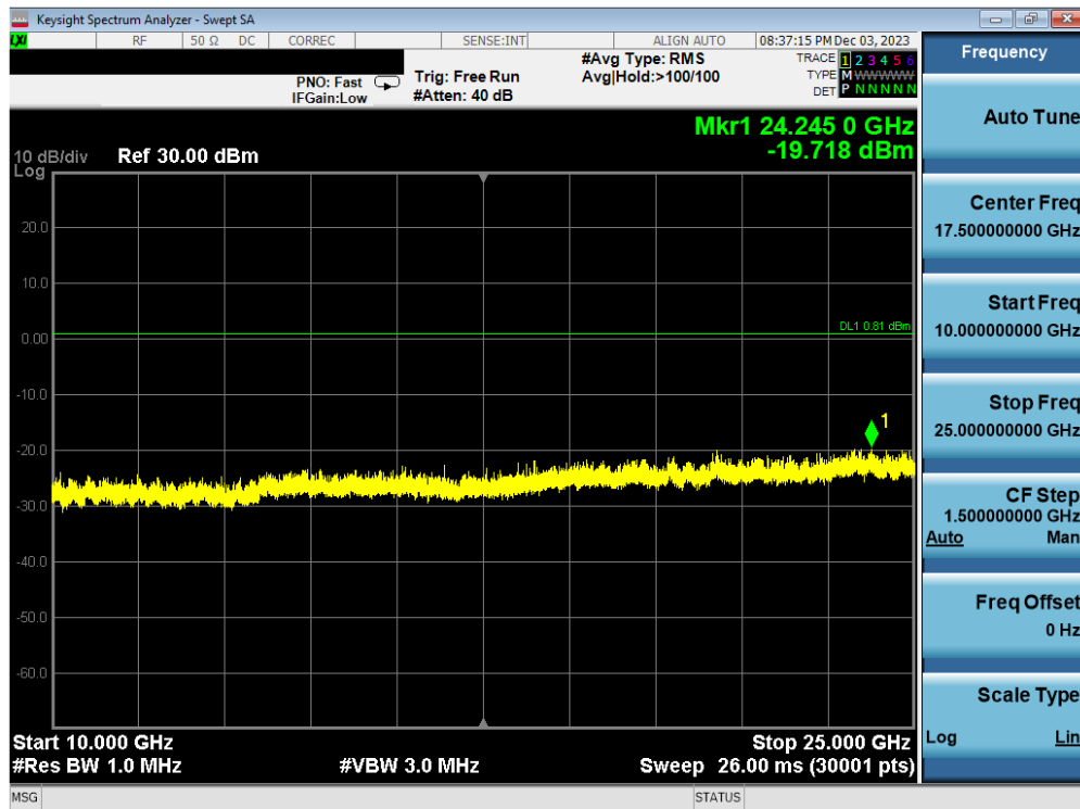
Plot 7-120. Conducted Spurious Plot Antenna WF2b (802.11ax OFDMA – RU26 – Ch. 6)
