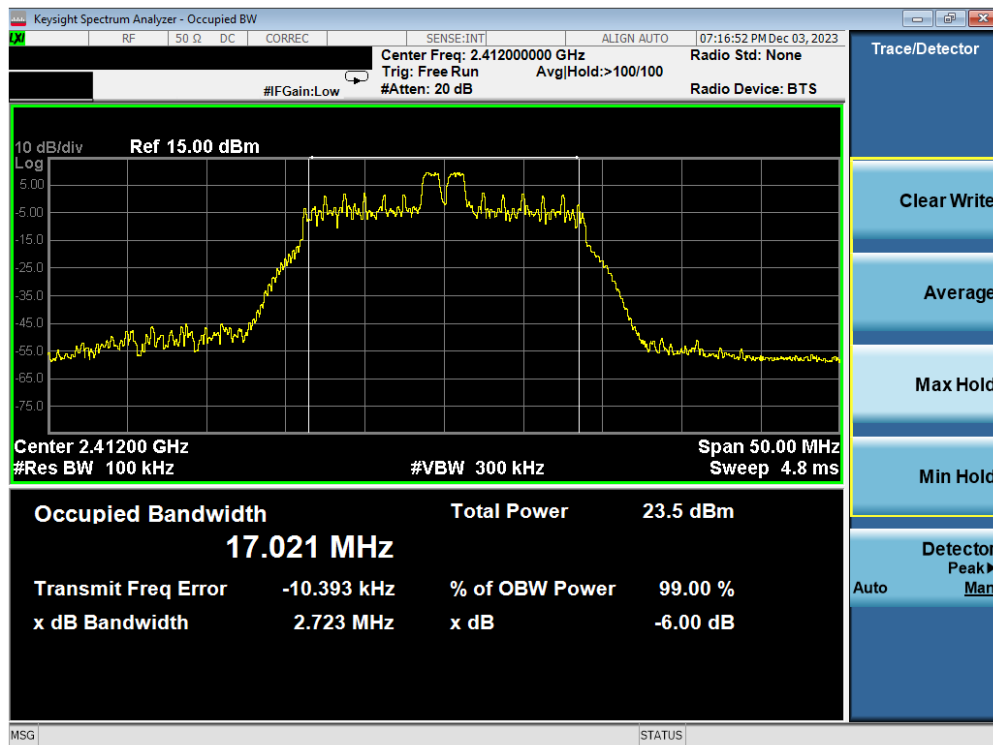
Plot 7-14. 6dB BW & 99% OBW Plot Antenna WF2b (802.11ax OFDMA – RU26 Index 4 – Ch. 1)
