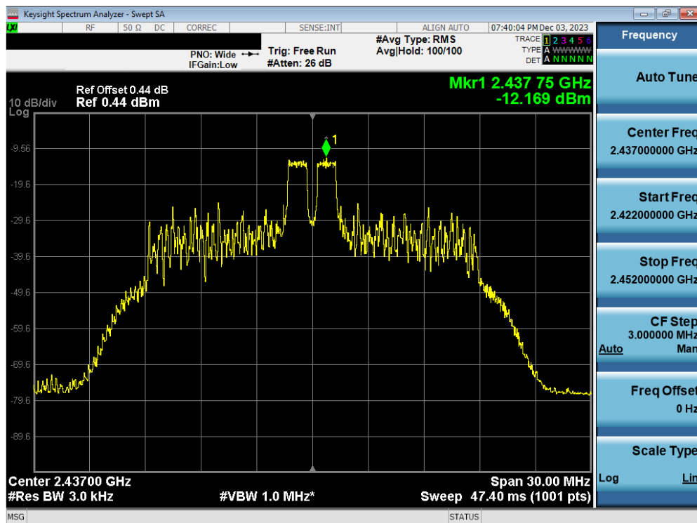
Plot 7-58. Power Spectral Density Plot Antenna WF2b (802.11ax OFDMA – RU26 Index 4 – Ch. 6)
