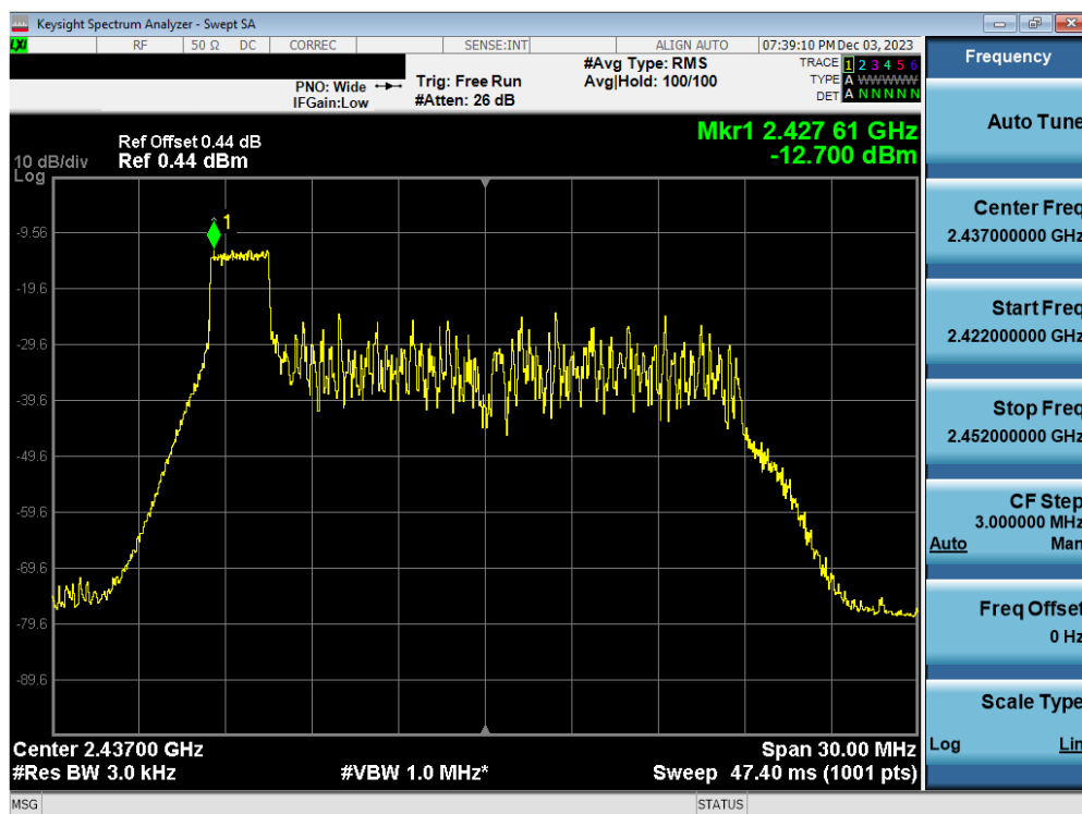
Plot 7-56. Power Spectral Density Plot Antenna WF2b (802.11ax OFDMA – RU26 Index 0 – Ch. 6)
