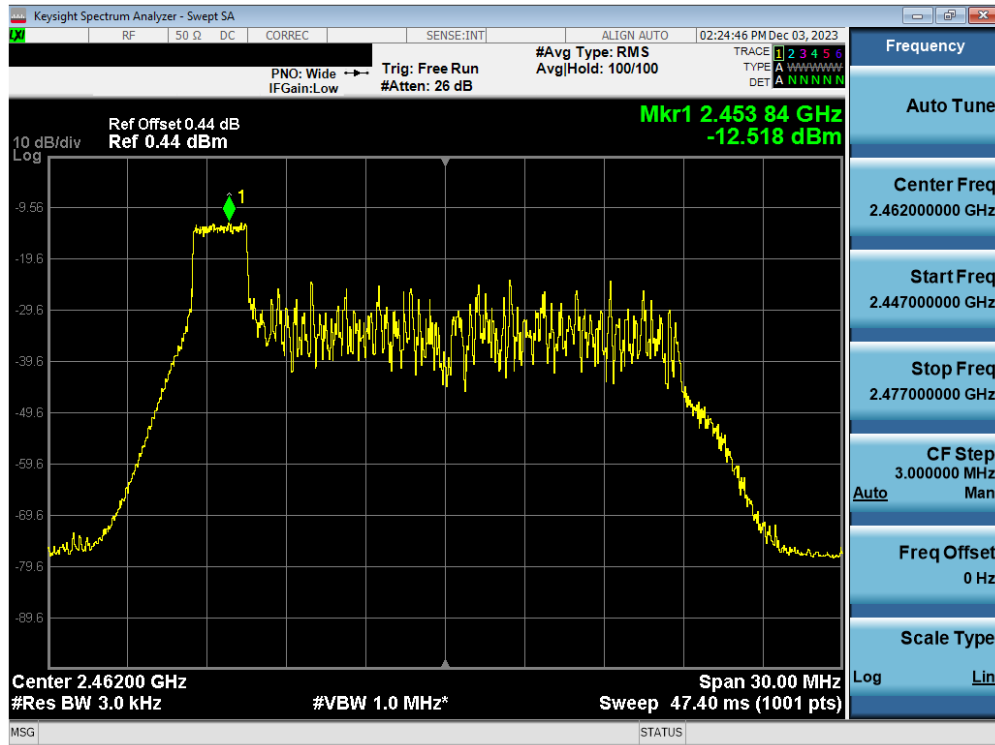
Plot 7-61. Power Spectral Density Plot Antenna WF7b (802.11ax OFDMA – RU26 Index 0 – Ch. 11)
