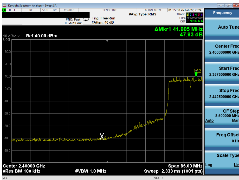
Plot 7-97. Band Edge Antenna WF2b (802.11ax OFDMA – RU242 – Ch. 6(low))
