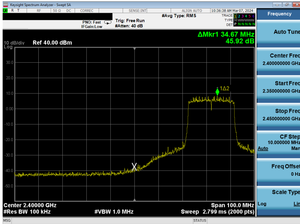
Plot 7-80. Band Edge Antenna WF7b (802.11ax OFDMA – RU242 – Ch. 5)
