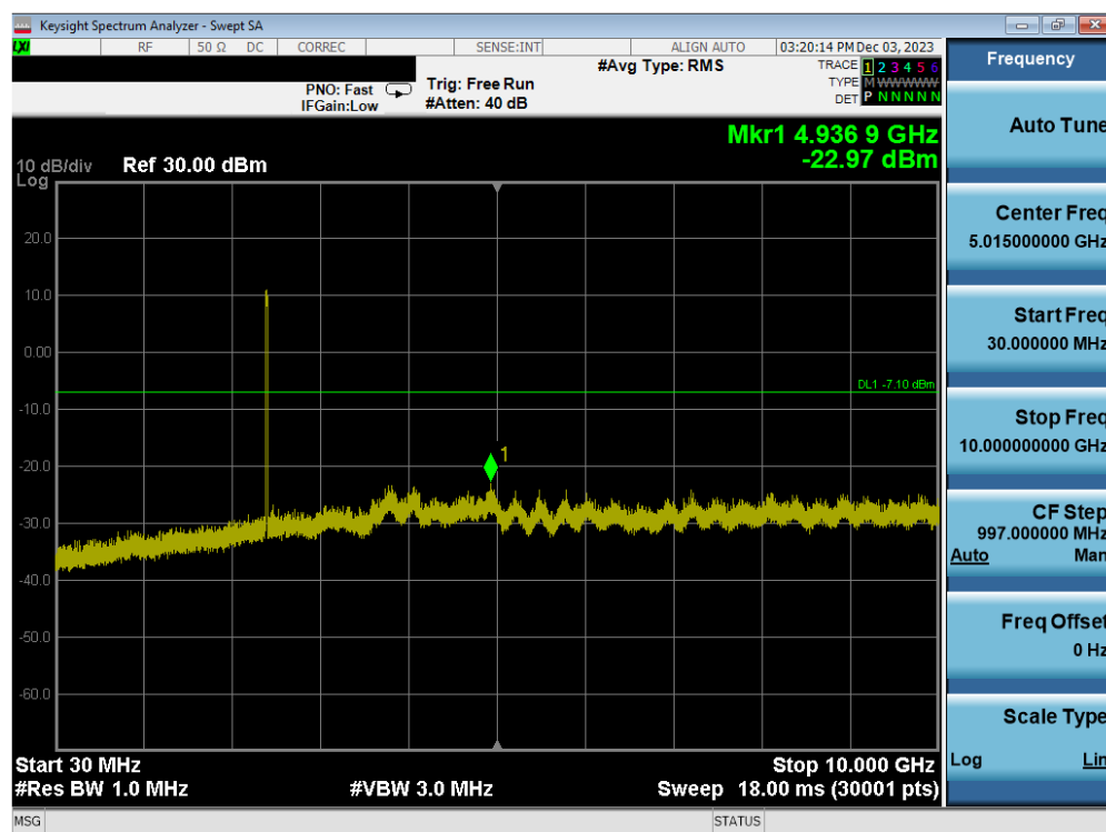
Plot 7-111. Conducted Spurious Plot Antenna WF7b (802.11ax OFDMA – RU242 – Ch. 1)
