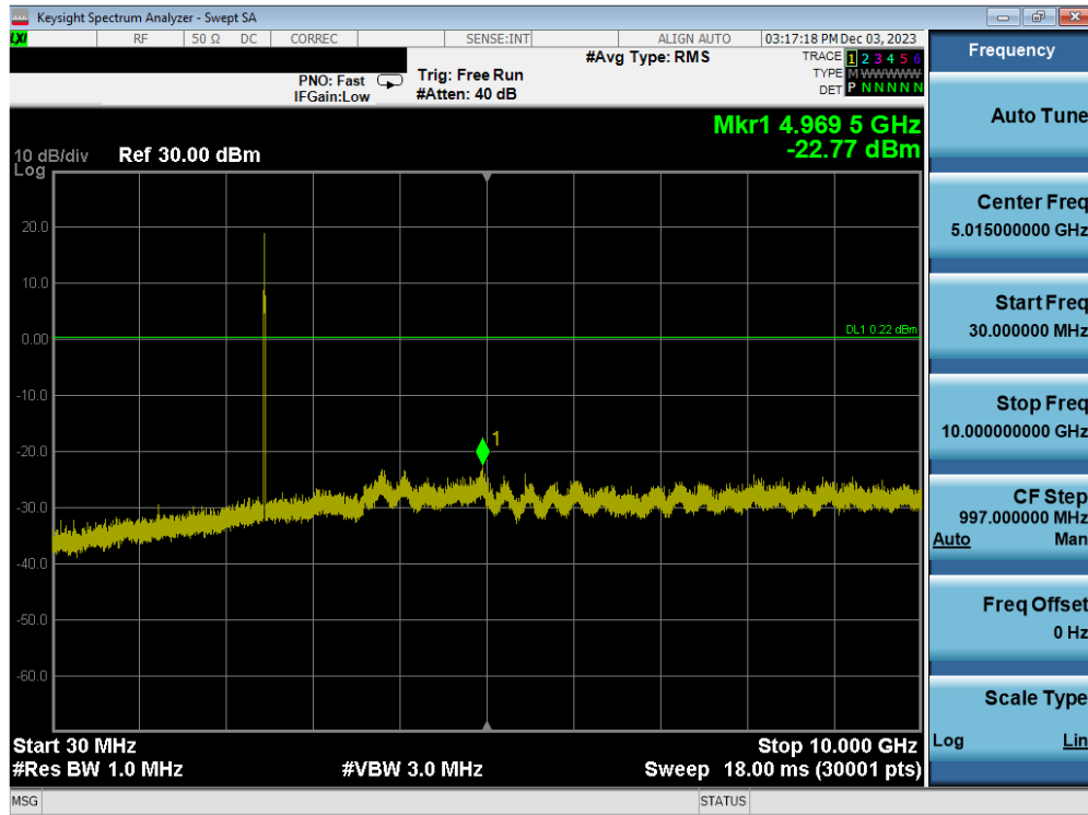
Plot 7-109. Conducted Spurious Plot Antenna WF7b (802.11ax OFDMA – RU26 – Ch. 11)
