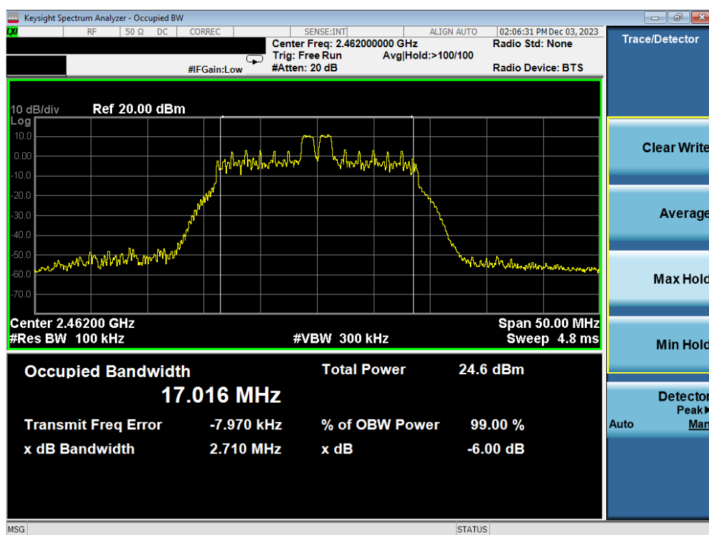
Plot 7-8. 6dB BW & 99% OBW Antenna WF7b (802.11ax OFDMA – RU26 Index 4 – Ch. 11)
