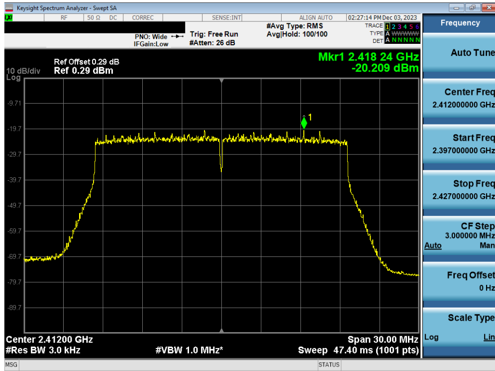
Plot 7-67. Power Spectral Density Plot Antenna WF7b (802.11ax OFDMA – RU242 – Ch. 1)
