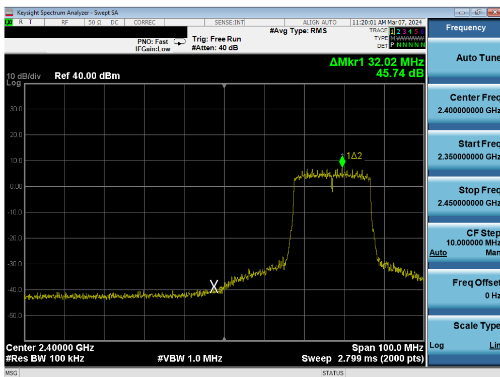
Plot 7-95. Band Edge Antenna WF2b (802.11ax OFDMA – RU242 – Ch. 4)
