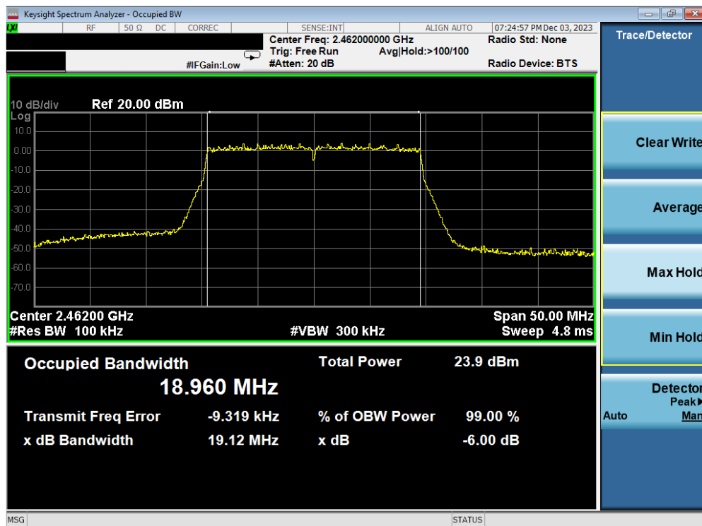
Plot 7-24. 6dB BW & 99% OBW Plot Antenna WF2b (802.11ax OFDMA – RU242 – Ch. 11)
