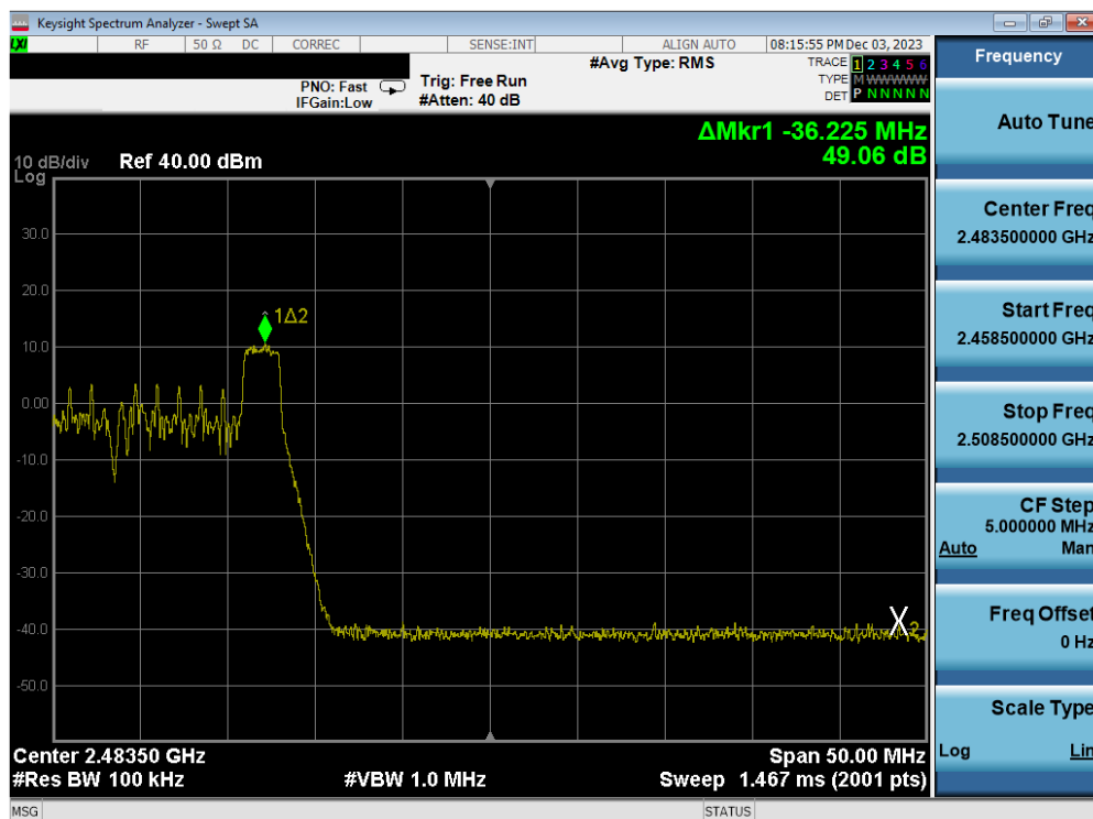
Plot 7-90. Band Edge Antenna WF2b (802.11ax OFDMA – RU26 Index 8 – Ch. 11)
