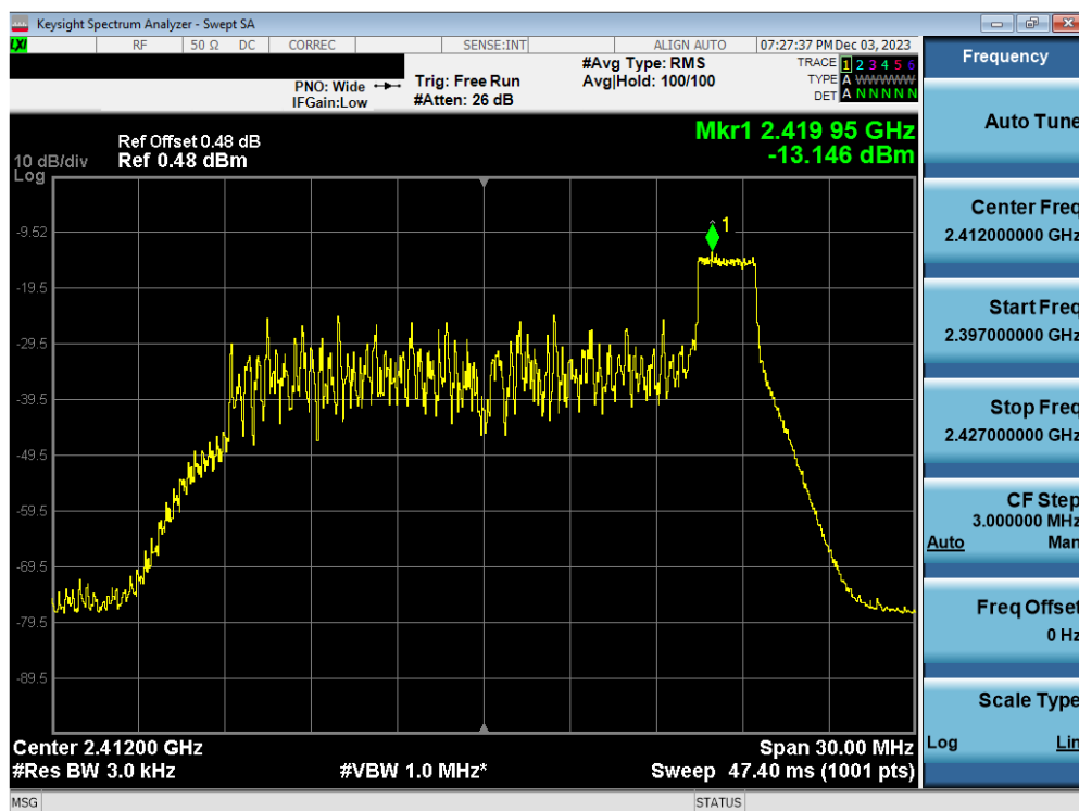
Plot 7-39. Power Spectral Density Plot Antenna WF2b (802.11ax OFDMA – RU26 Index 8 – Ch. 1)
