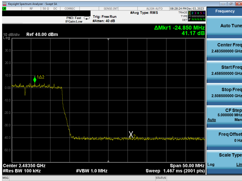
Plot 7-103. Band Edge Antenna WF2b (802.11ax OFDMA – RU242 – Ch. 11)
