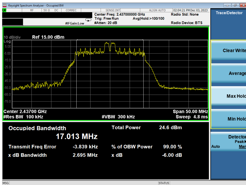
Plot 7-5. 6dB BW & 99% OBW Plot Antenna WF7b (802.11ax OFDMA – RU26 Index 4 – Ch. 6)
