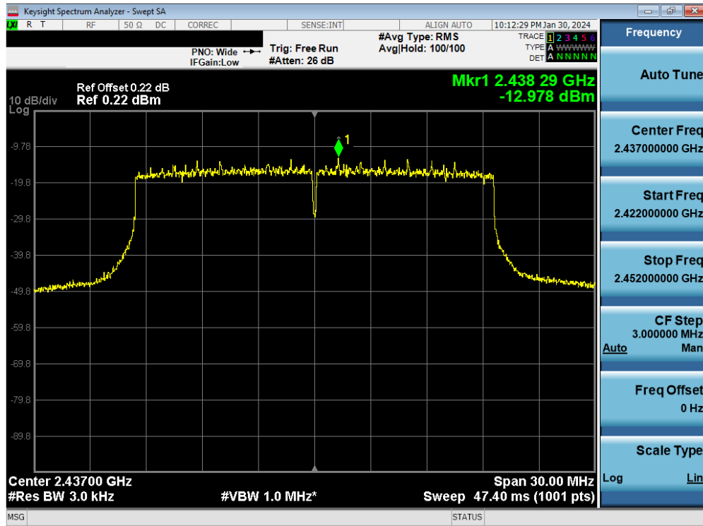
Plot 7-35. Power Spectral Density Plot Antenna WF7b (802.11ax OFDMA – RU242 – Ch. 6)
