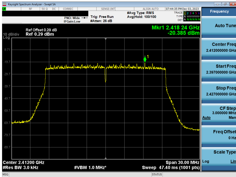
Plot 7-68. Power Spectral Density Plot Antenna WF2b (802.11ax OFDMA – RU242 – Ch. 1)
