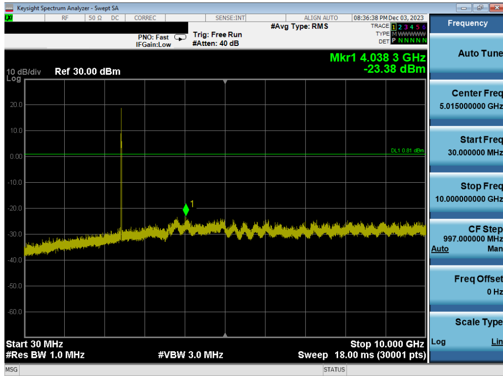
Plot 7-119. Conducted Spurious Plot Antenna WF2b (802.11ax OFDMA – RU26 – Ch. 6)
