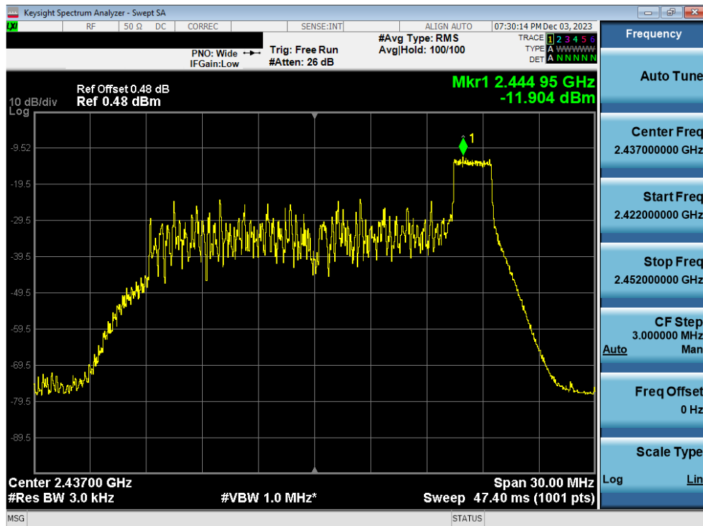
Plot 7-42. Power Spectral Density Plot Antenna WF2b (802.11ax OFDMA – RU26 Index 8 – Ch. 6)
