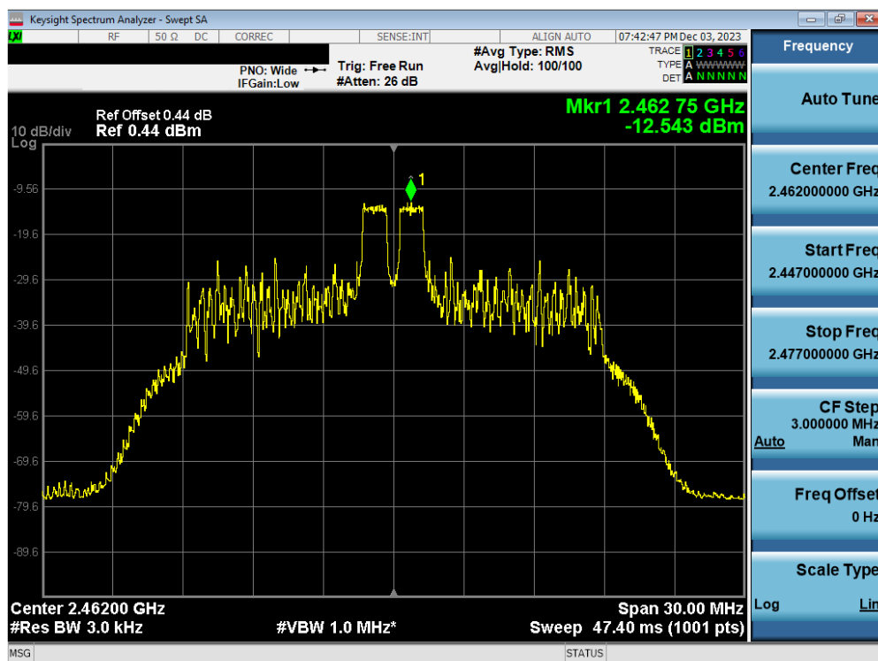
Plot 7-64. Power Spectral Density Plot Antenna WF2b (802.11ax OFDMA – RU26 Index 4 – Ch. 11)
