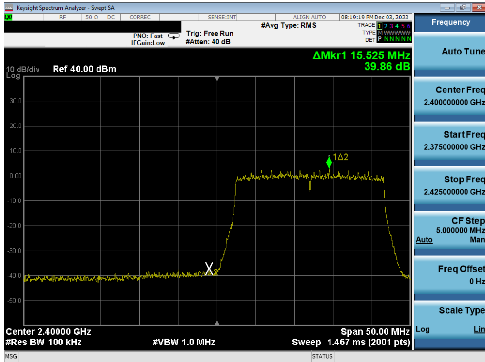
Plot 7-92. Band Edge Antenna WF2b (802.11ax OFDMA – RU242 – Ch. 1)
