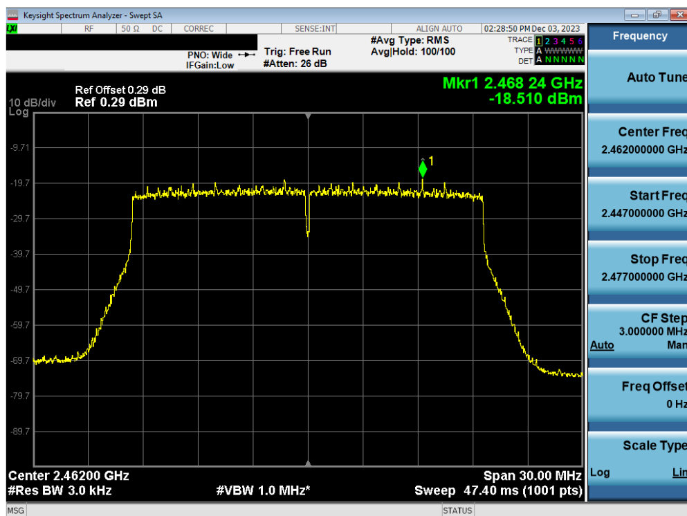
Plot 7-71. Power Spectral Density Plot Antenna WF7b (802.11ax OFDMA – RU242 – Ch. 11)
