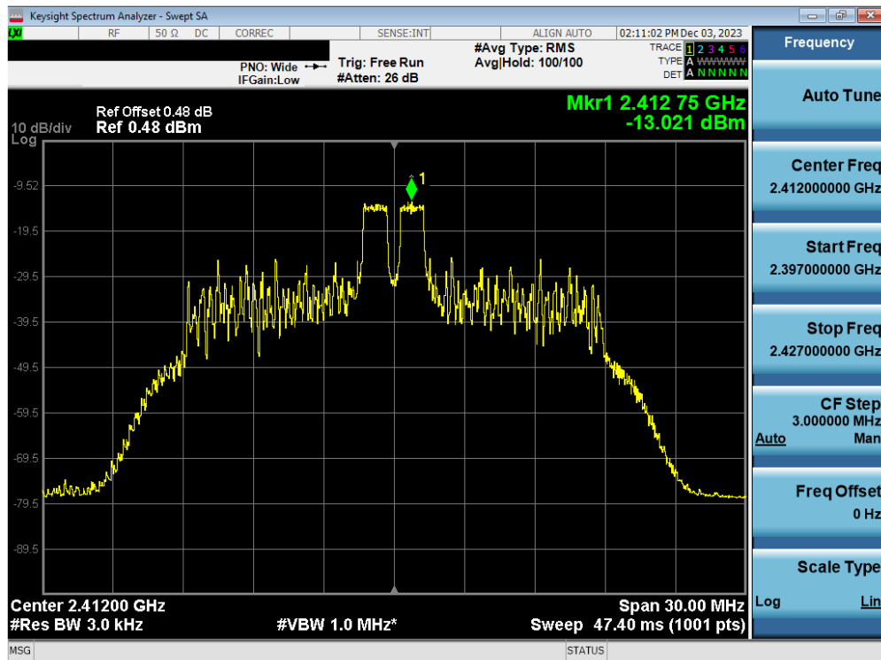
Plot 7-26. Power Spectral Density Plot Antenna WF7b (802.11ax OFDMA – RU26 Index 4 – Ch. 1)
