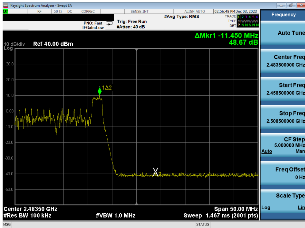
Plot 7-75. Band Edge Antenna WF7b (802.11ax OFDMA – RU26 Index 8 – Ch. 12)
