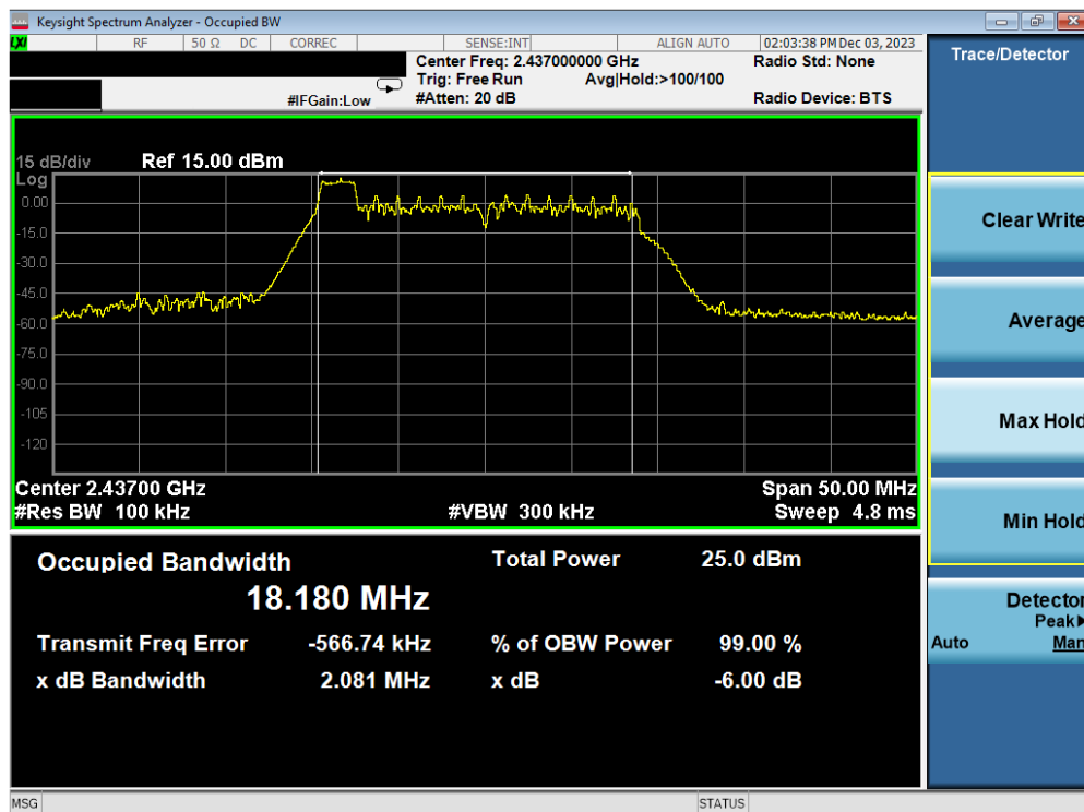
Plot 7-4. 6dB BW & 99% OBW Plot Antenna WF7b (802.11ax OFDMA – RU26 Index 0 – Ch. 6)
