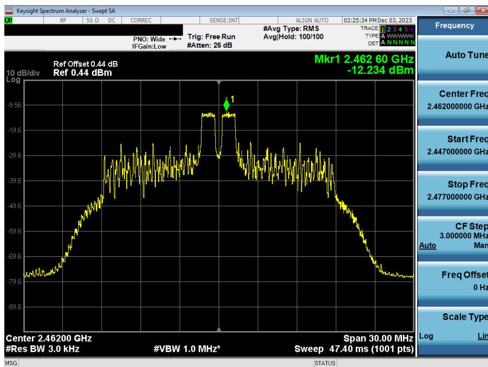
Plot 7-63. Power Spectral Density Plot Antenna WF7b (802.11ax OFDMA – RU26 Index 4 – Ch. 11)
