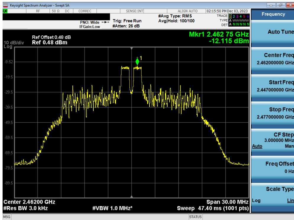
Plot 7-32. Power Spectral Density Plot Antenna WF7b (802.11ax OFDMA – RU26 Index 4 – Ch. 11)
