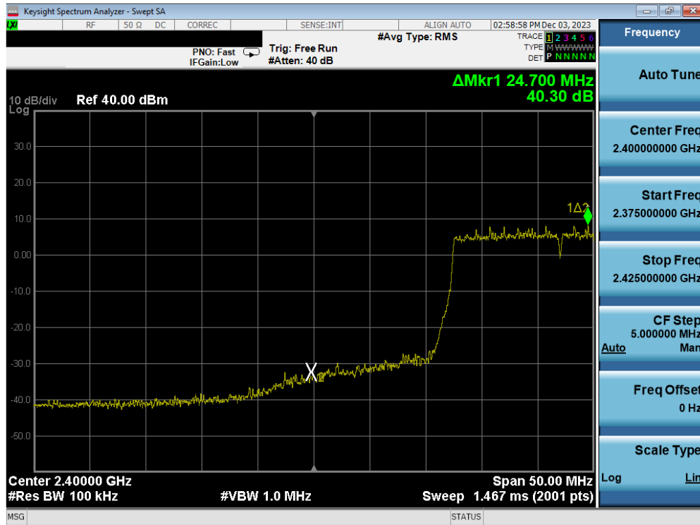
Plot 7-78. Band Edge Antenna WF7b (802.11ax OFDMA – RU242 – Ch. 3)
