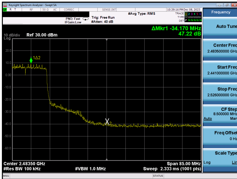
Plot 7-84. Band Edge Antenna WF7b (802.11ax OFDMA – RU242 – Ch. 8)
