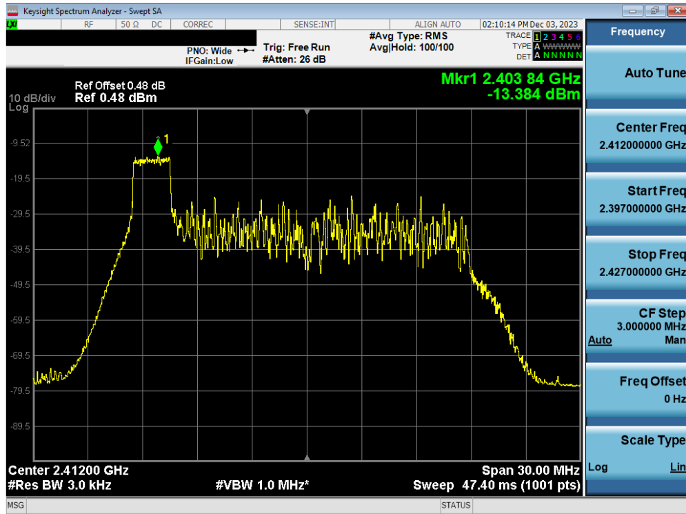
Plot 7-25. Power Spectral Density Plot Antenna WF7b (802.11ax OFDMA – RU26 Index 0 – Ch. 1)
