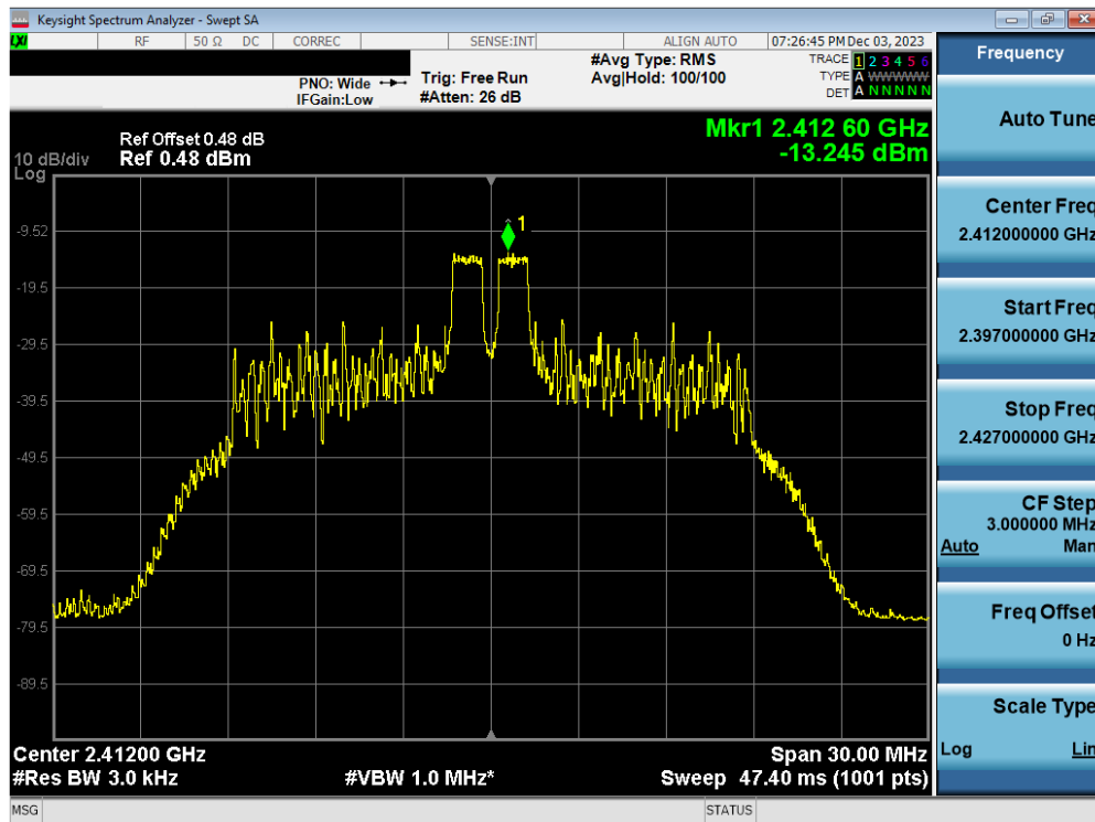
Plot 7-38. Power Spectral Density Plot Antenna WF2b (802.11ax OFDMA – RU26 Index 4 – Ch. 1)
