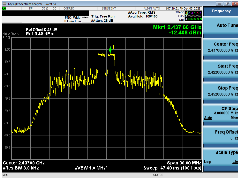
Plot 7-41. Power Spectral Density Plot Antenna WF2b (802.11ax OFDMA – RU26 Index 4 – Ch. 6)
