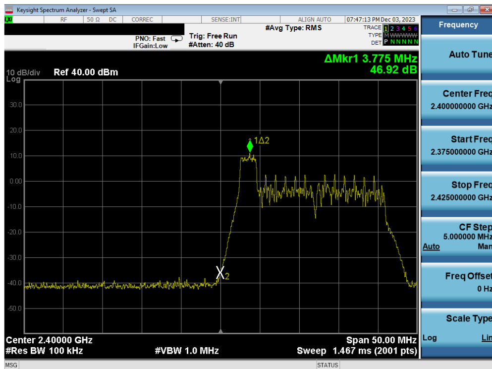
Plot 7-89. Band Edge Antenna WF2b (802.11ax OFDMA – RU26 Index 0 – Ch. 1)
