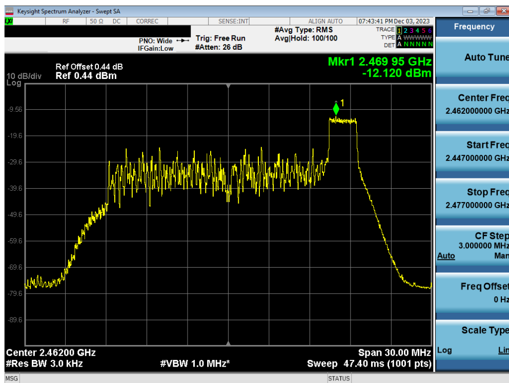
Plot 7-66. Power Spectral Density Plot Antenna WF2b (802.11ax OFDMA – RU26 Index 8 – Ch. 11)
