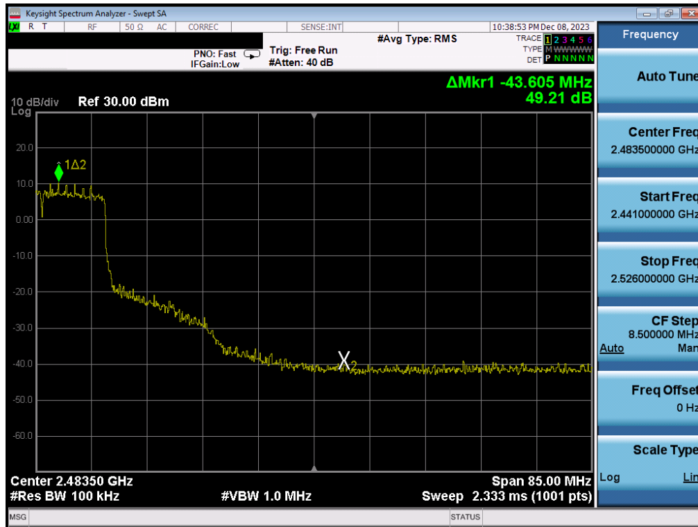
Plot 7-83. Band Edge Antenna WF7b (802.11ax OFDMA – RU242 – Ch. 7)
