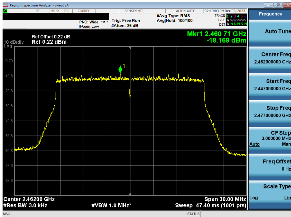
Plot 7-36. Power Spectral Density Plot Antenna WF7b (802.11ax OFDMA – RU242 – Ch. 11)
