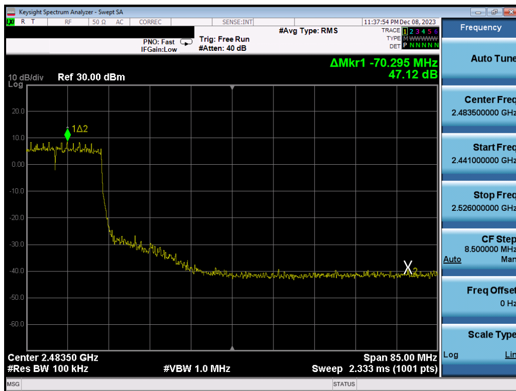
Plot 7-100. Band Edge Antenna WF2b (802.11ax OFDMA – RU242 – Ch. 8)
