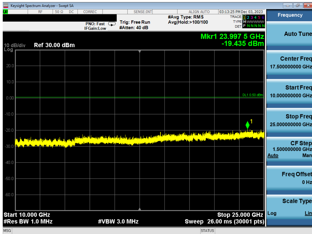
Plot 7-108. Conducted Spurious Plot Antenna WF7b (802.11ax OFDMA – RU26 – Ch. 6)
