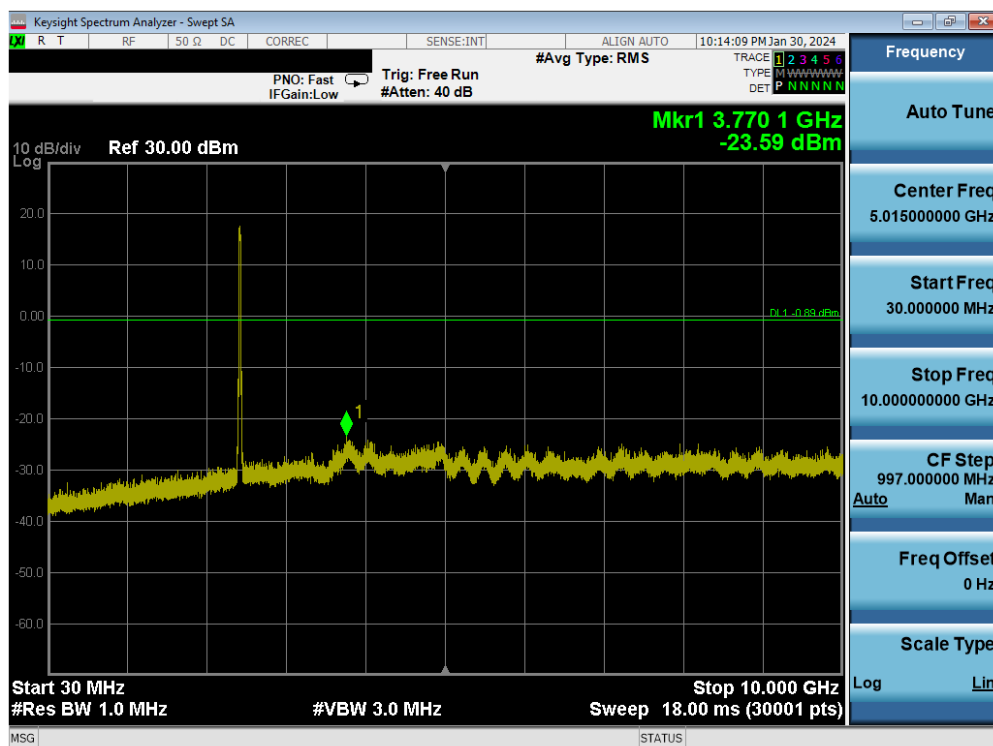
Plot 7-113. Conducted Spurious Plot Antenna WF7b (802.11ax OFDMA – RU242 – Ch. 6)
