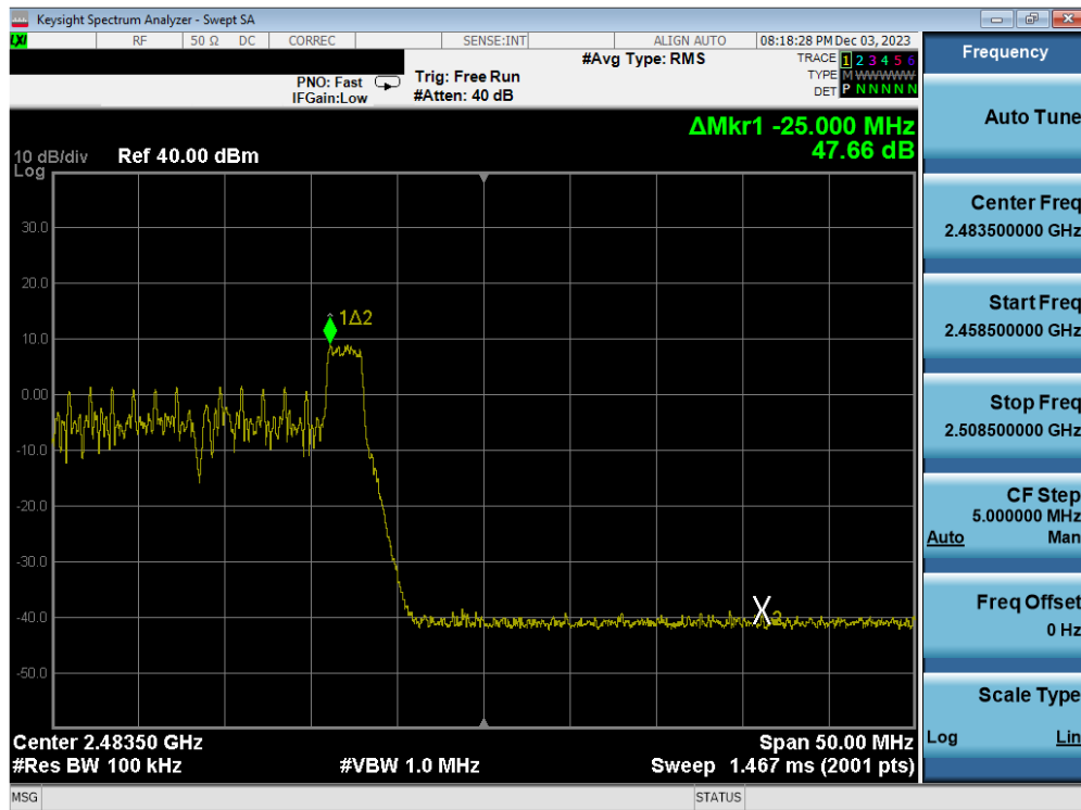
Plot 7-91. Band Edge Antenna WF2b (802.11ax OFDMA – RU26 Index 8 – Ch. 12)
