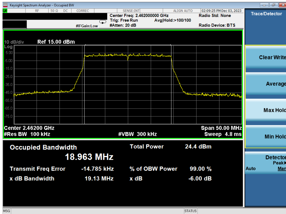
Plot 7-12. 6dB BW & 99% OBW Plot Antenna WF7b (802.11ax OFDMA – RU242 – Ch. 11)
