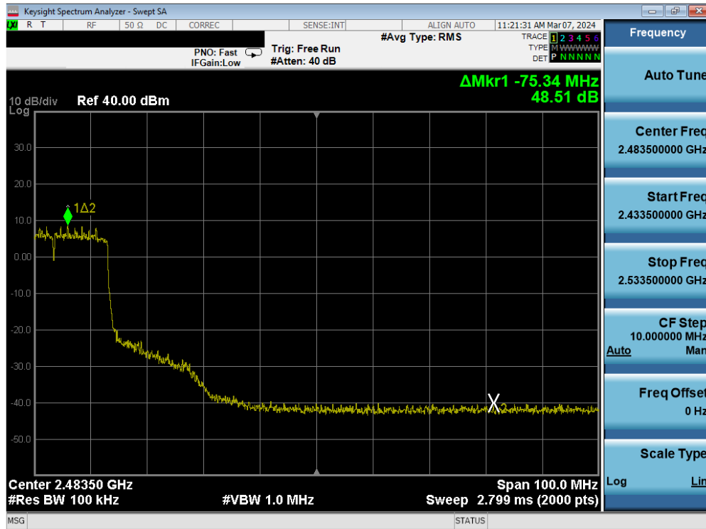
Plot 7-98. Band Edge Antenna WF2b (802.11ax OFDMA – RU242 – Ch. 6(high))
