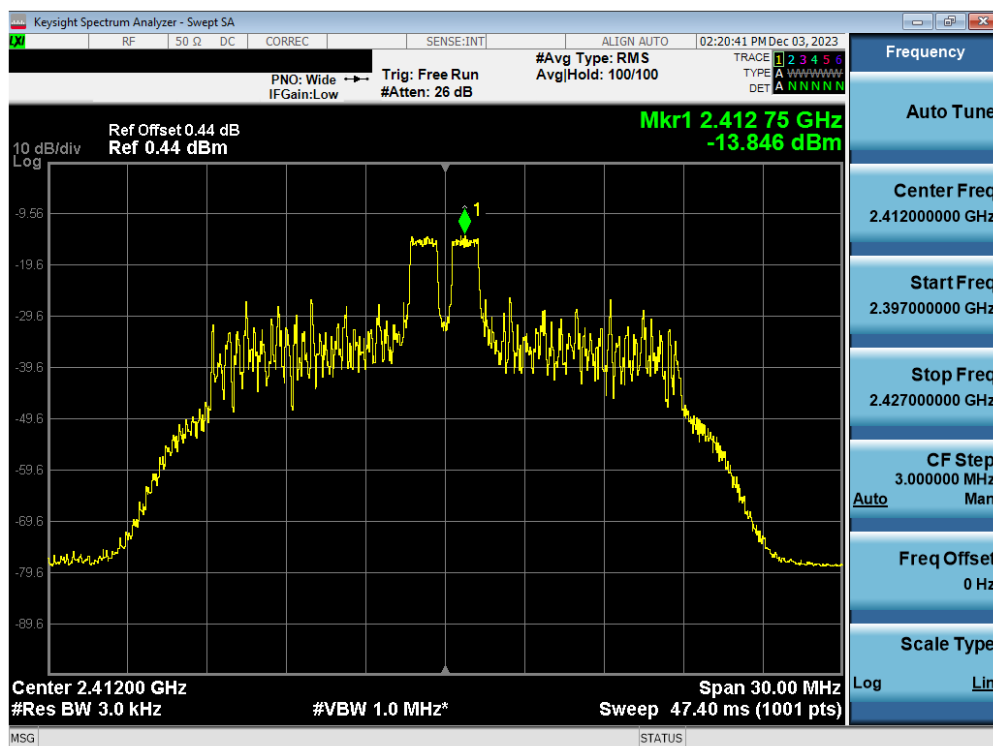
Plot 7-51. Power Spectral Density Plot Antenna WF7b (802.11ax OFDMA – RU26 Index 4 – Ch. 1)
