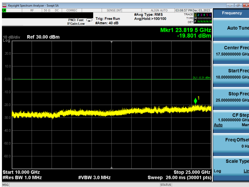
Plot 7-106. Conducted Spurious Plot Antenna WF7b (802.11ax OFDMA – RU26 – Ch. 1)
