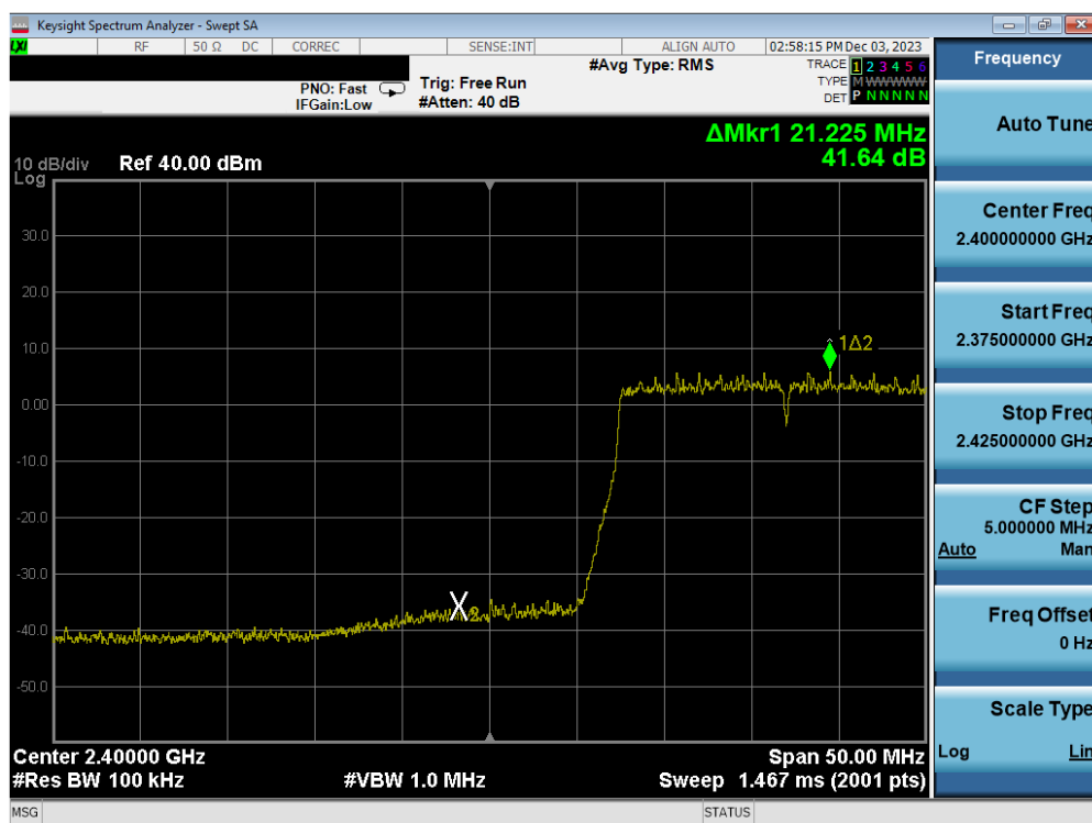
Plot 7-77. Band Edge Antenna WF7b (802.11ax OFDMA – RU242 – Ch. 2)
