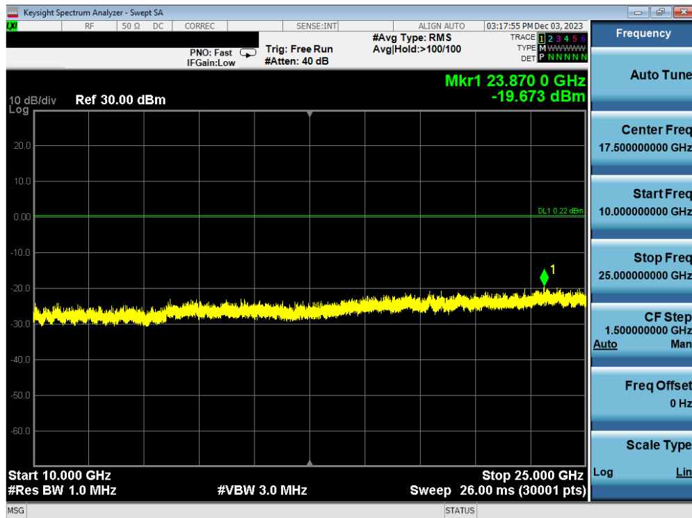
Plot 7-110. Conducted Spurious Plot Antenna WF7b (802.11ax OFDMA – RU26 – Ch. 11)
