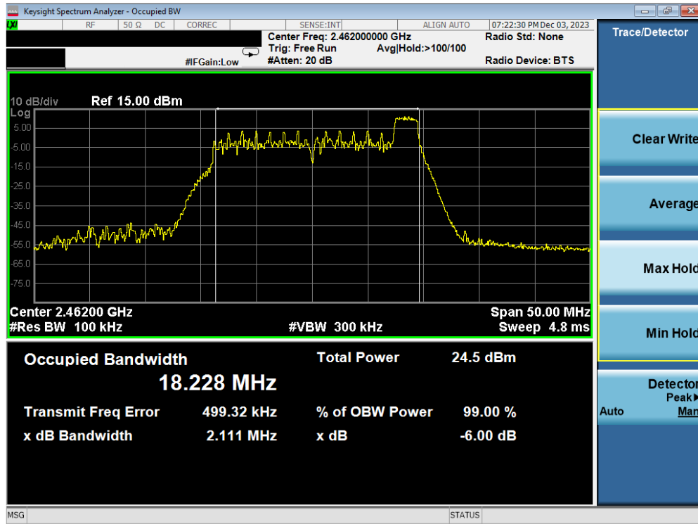
Plot 7-21. 6dB BW & 99% OBW Plot Antenna WF2b (802.11ax OFDMA – RU26 Index 8 – Ch. 11)
