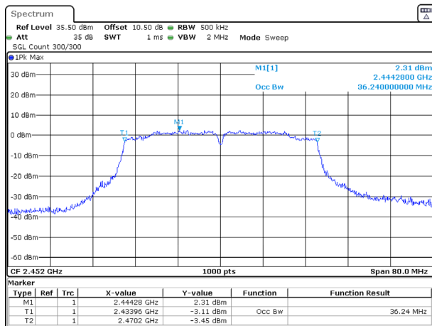
802.11n40_2452MHz_Chain 0
