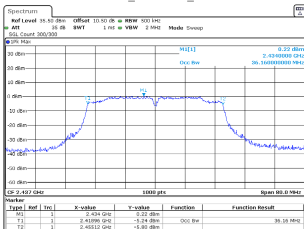
802.11n40_2437MHz_Chain 1
