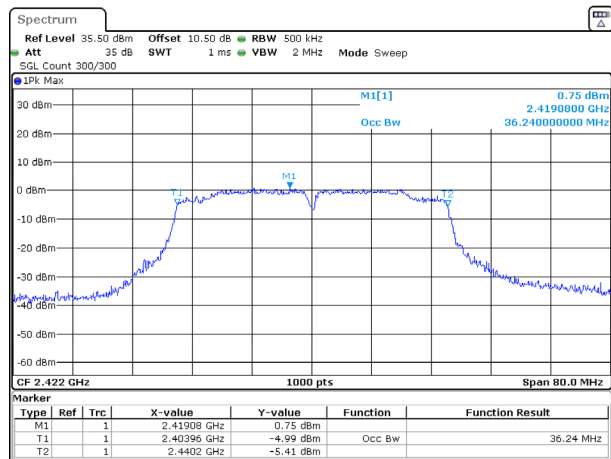
802.11n40_2422MHz_Chain 1
