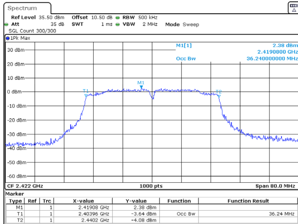
802.11n40_2422MHz_Chain 0
