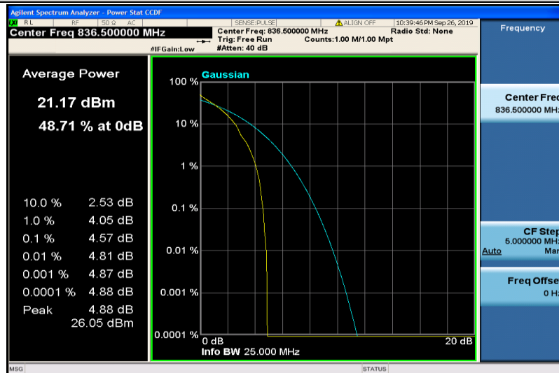
Band5-3MHz-QPSK-20525-1RB#0
