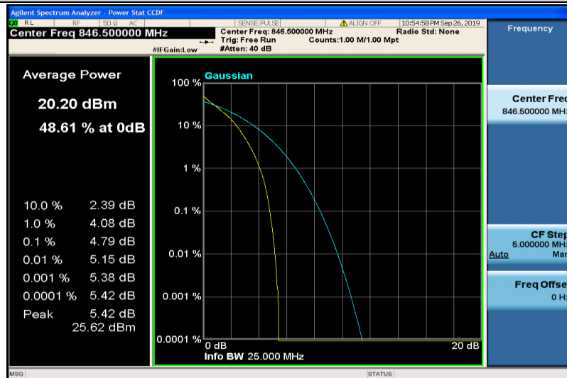
Band5-5MHz-QPSK-20625-25RB#0
