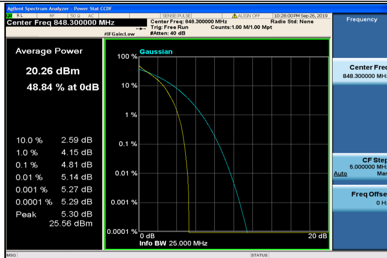
Band5-1.4MHz-QPSK-20643-6RB#0
