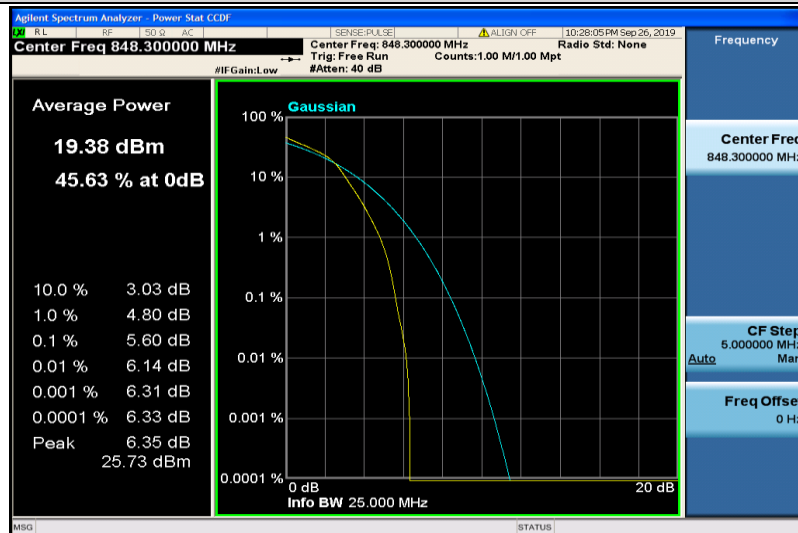
Band5-1.4MHz-16QAM-20643-6RB#0
