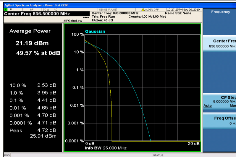
Band5-1.4MHz-QPSK-20525-1RB#0
