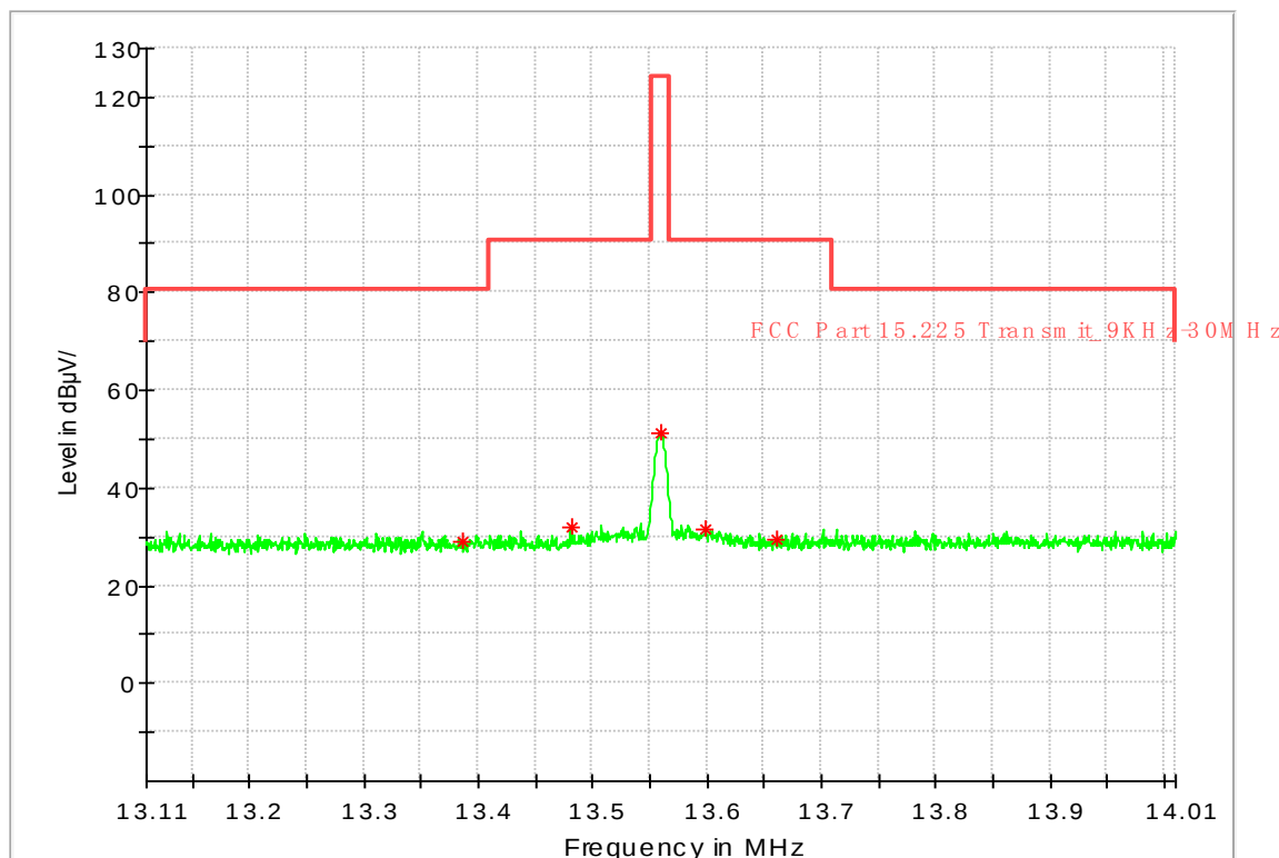
MEASUREMENT RESULT: QP Detector
