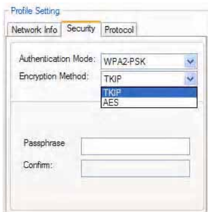
Figure 37: TKIP/AES Settings
