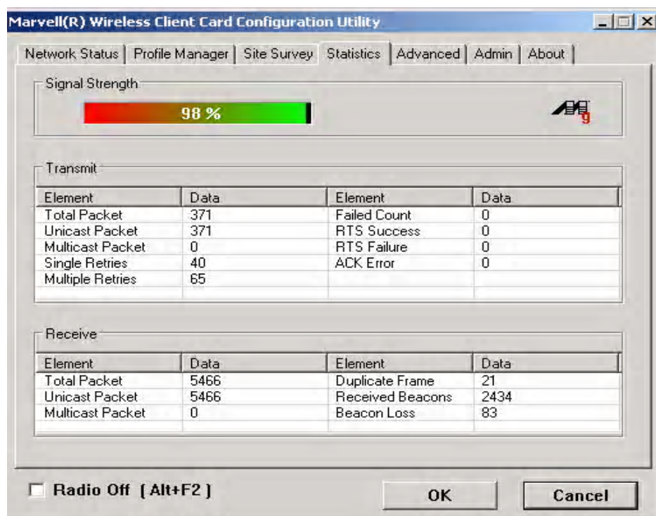
Figure 42: Statistics Window
