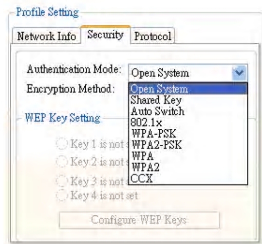
Figure 22: Authentication Modes
