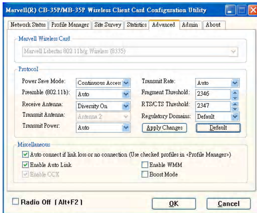
Figure 45: Advanced Tab
