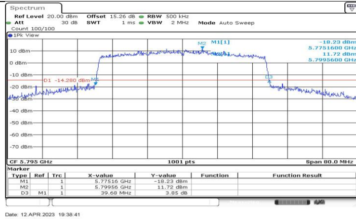
11AX40-CDD_Ant4_5795
