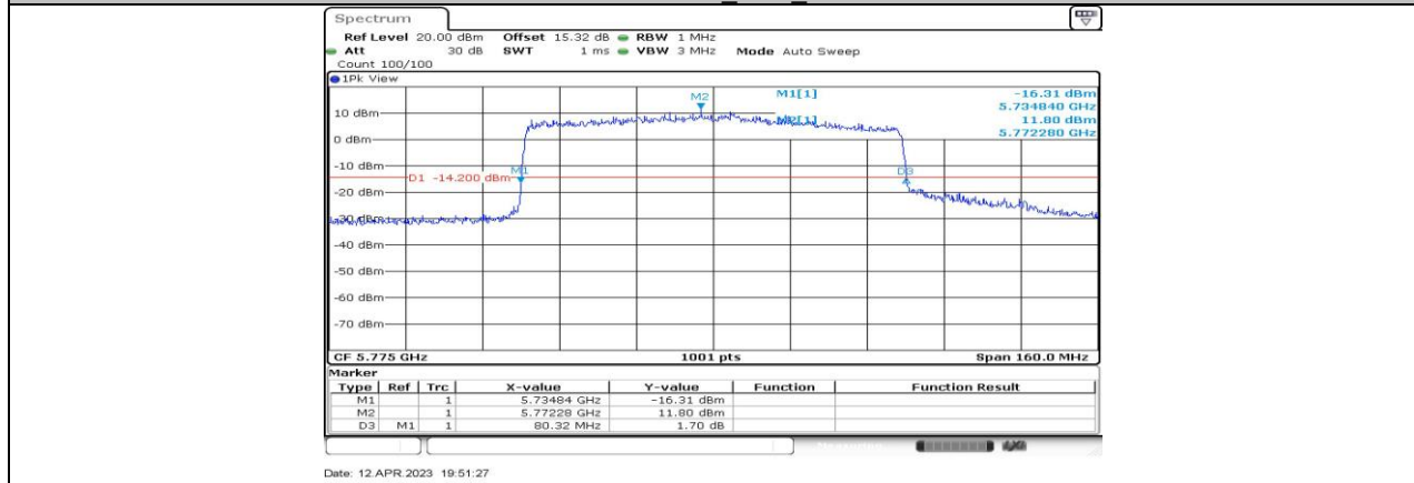
11AX80-CDD_Ant3_5775
