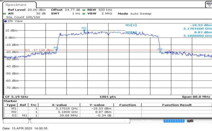
11BE40-CDD_Ant4_5190
