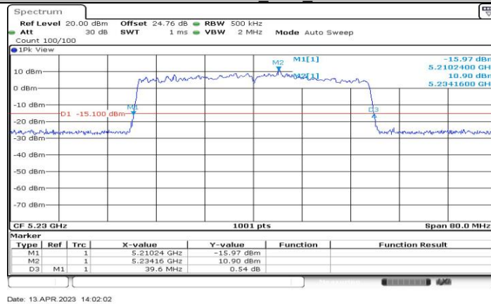
11BE40-CDD_Ant4_5230
