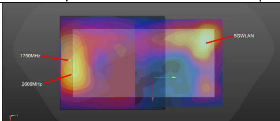
Sensor Off Back 23mm_ WWAN+5G WLAN
