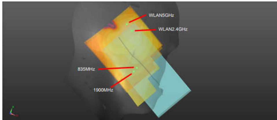
Head Left Cheek 0mm_WWAN+2.4G/5G WLAN
