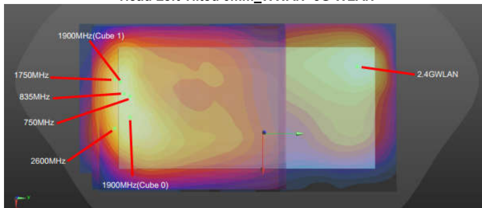
Hotspot & Body at Back 5mm_WWAN+2.4G WLAN
