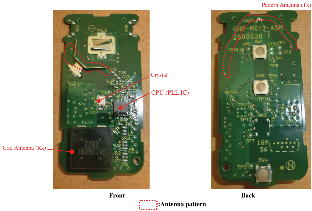
Figure 8.2 FOB appearance (PCB)
