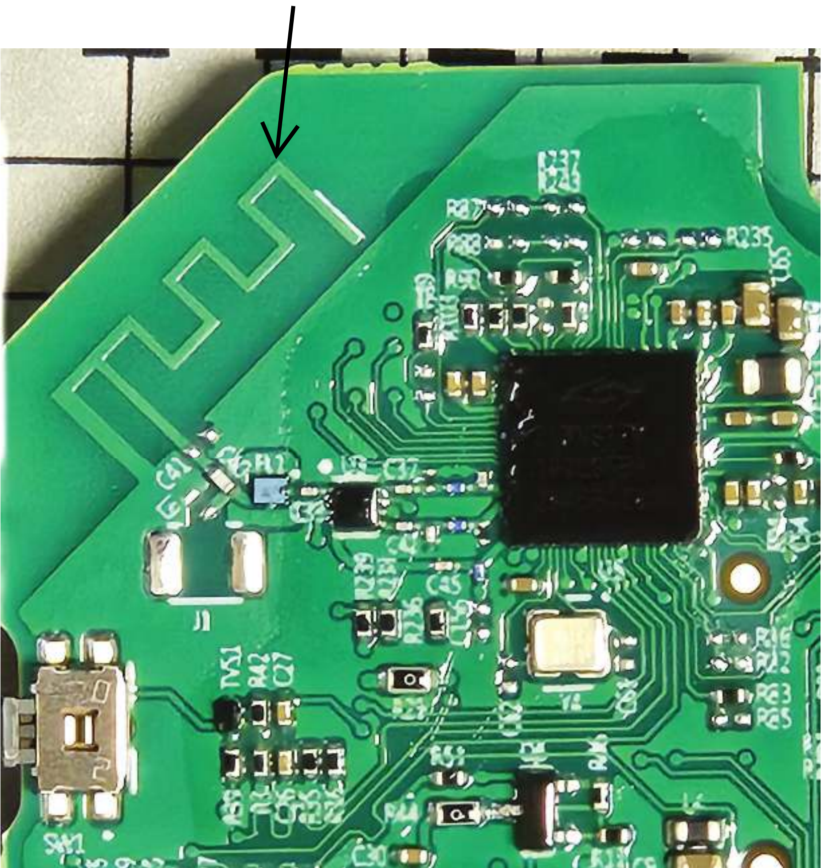
WIFI Meander Antenna
