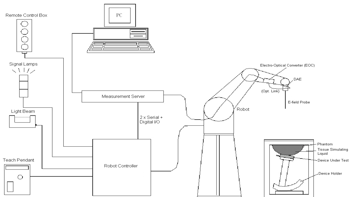
Fig-3.1 DASY System Setup
