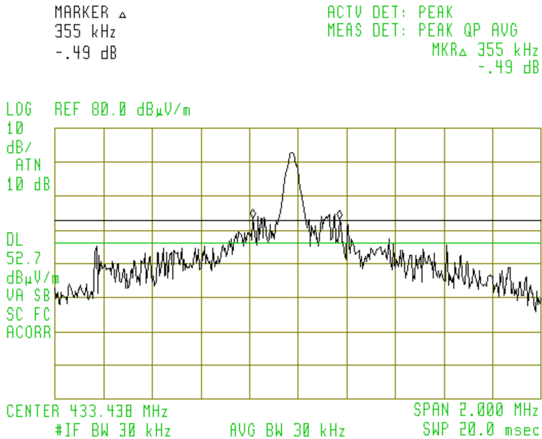
Figure 6.1 20 dB Occupied Bandwidth
