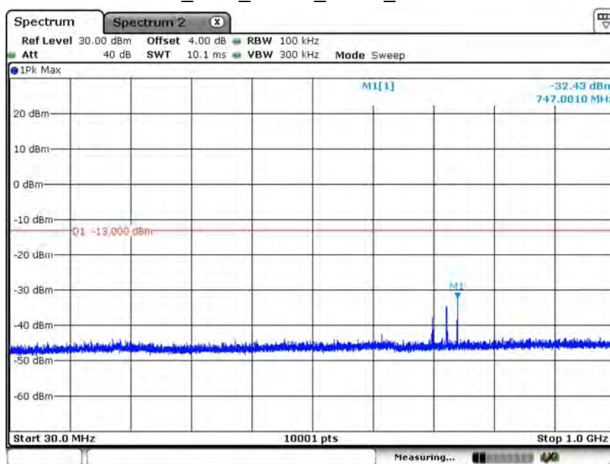
PCS_1900_CH512_GPRS_Below 1G
