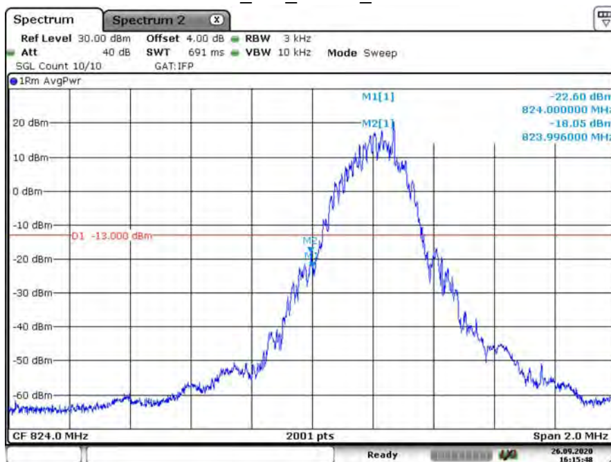
GSM_850_CH128_GPRS
