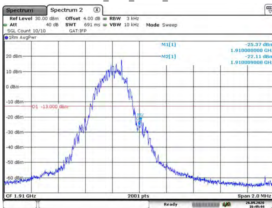
PCS_1900_CH810_GPRS
