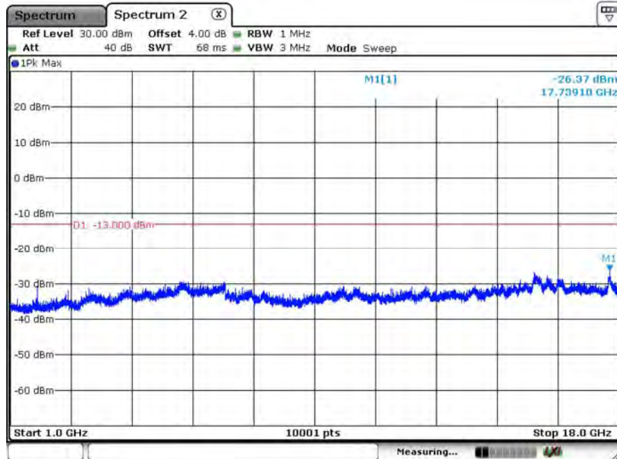
GSM_850_CH128_GPRS_Above 1G
