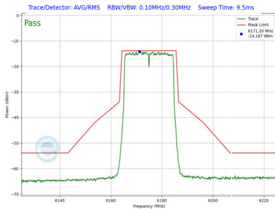
Plot 7-446. In-Band Emission Plot Antenna WF8 Low Power Indoor (20MHz 802.11a (UNII Band 5) – Ch. 45, MCS2)
