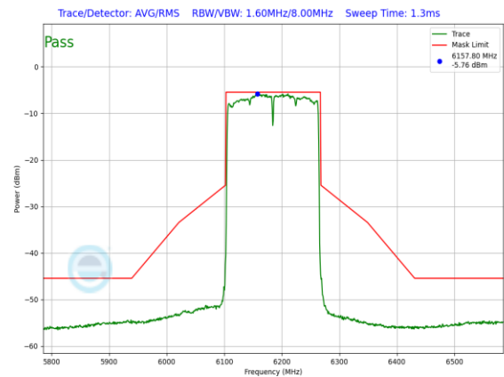
Plot 7-449. In-Band Emission Plot Antenna WF8 Low Power Indoor (160MHz 802.11a (UNII Band 5) – Ch. 47, MCS2)
