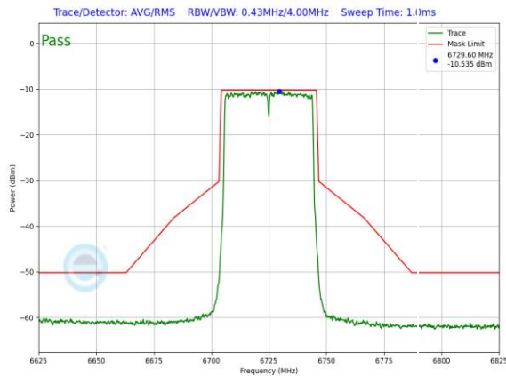
Plot 7-457. In-Band Emission Plot Antenna WF8 Low Power Indoor (40MHz 802.11ax (UNII Band 7) – Ch. 155, MCS2)
