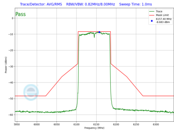
Plot 7-448. In-Band Emission Plot Antenna WF8 Low Power Indoor (80MHz 802.11a (UNII Band 5) – Ch. 39, MCS2)
