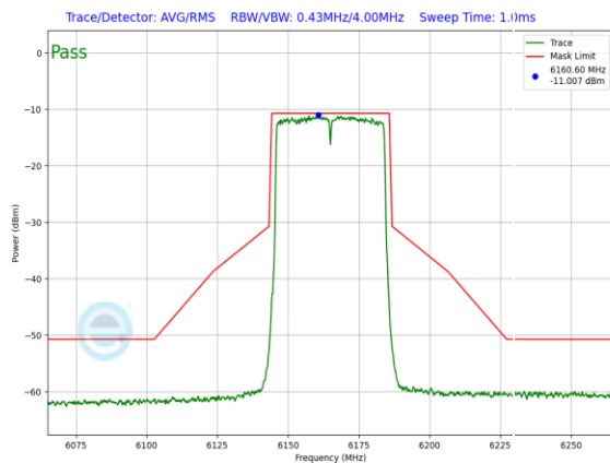
Plot 7-447. In-Band Emission Plot Antenna WF8 Low Power Indoor (40MHz 802.11a (UNII Band 5) – Ch. 43, MCS2)
