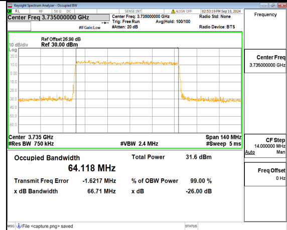
n77(3700-3980MHz) 70M DFT-s-OFDM QPSK Outer_Full Low
