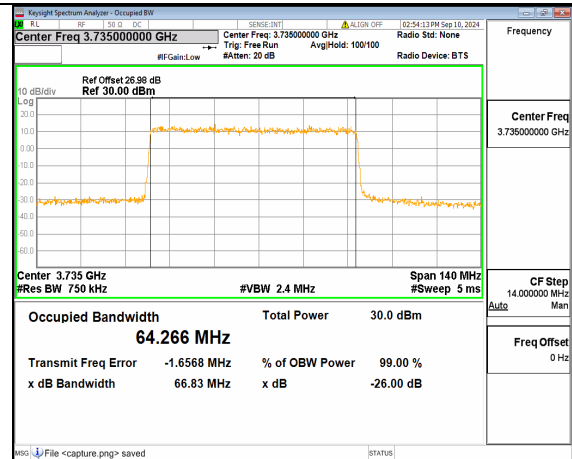
n77(3700-3980MHz) 70M DFT-s-OFDM 64QAM Outer_Full Low
