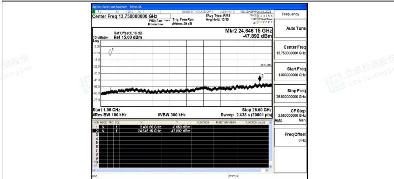
2DH5_Ant1_2441_0~Reference
