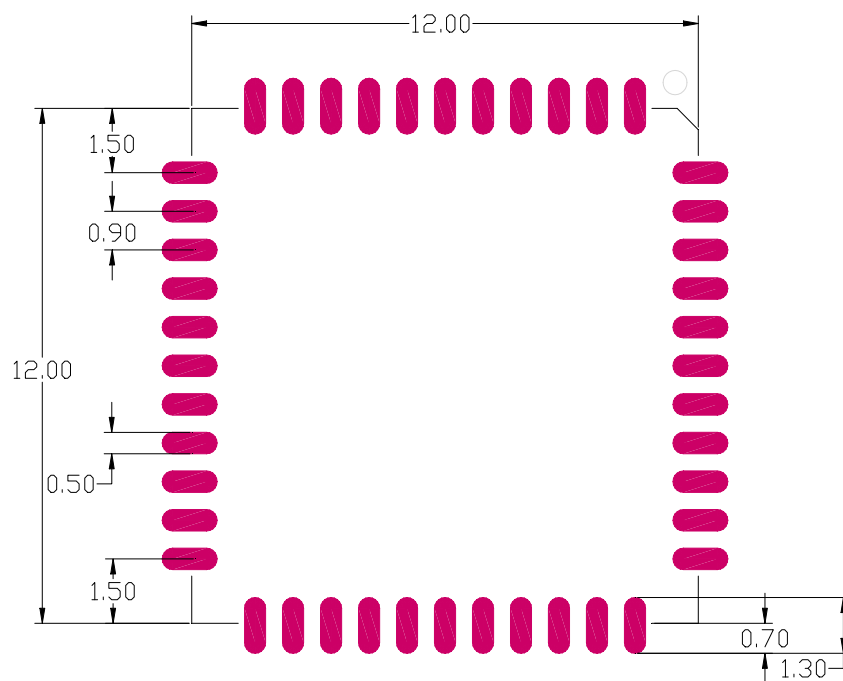
(Top view)
