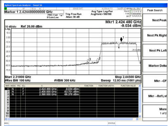
Channel 3 / 2422 MHz
