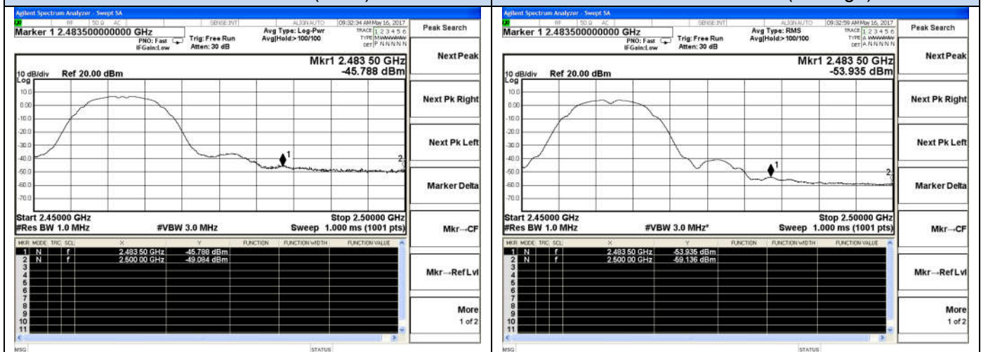
802.11b-High channel(Average)
