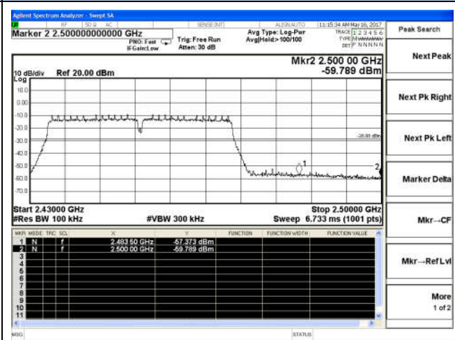
Channel 9 / 2452 MHz
