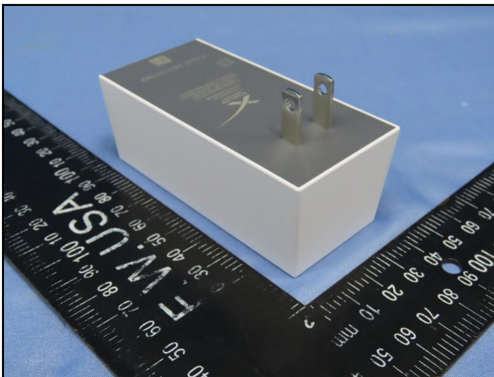
Adapter 1 (Model: UTP-231L)
