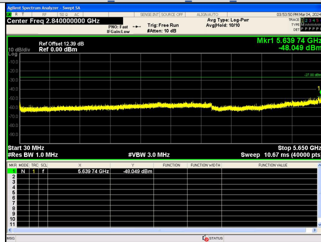
Spurious Emission:30.0~5650 MHz IEEE 802.11ac_Channel 149_20MHz_Antenna 0
