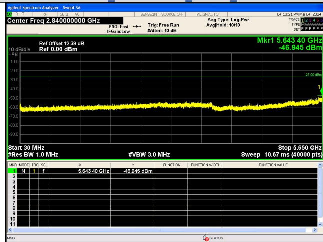
Spurious Emission:30.0~5650 MHz IEEE 802.11n_Channel 151_40MHz_Antenna 0
