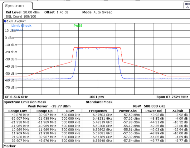
802.11ax (20MHz) 6515MHz Chain C NSS-1
