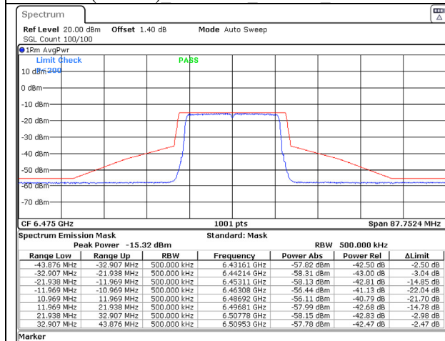
802.11ax (20MHz) 6475MHz Chain A NSS-1
