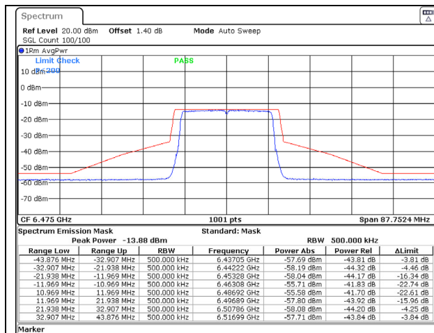
802.11ax (20MHz) 6475MHz Chain C NSS-1
