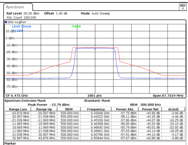
802.11ax (20MHz) 6475MHz Chain D NSS-1
