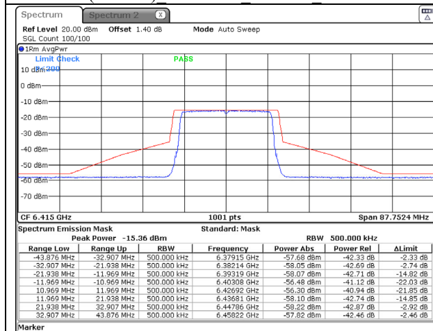
802.11ax (20MHz) 6415MHz Chain A NSS-1
