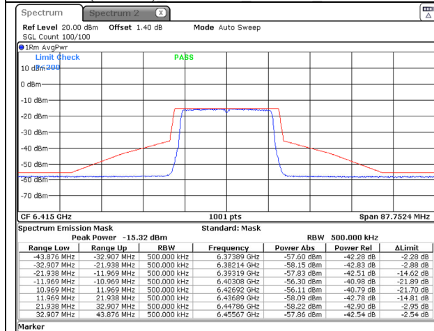
802.11ax (20MHz) 6415MHz Chain C NSS-1
