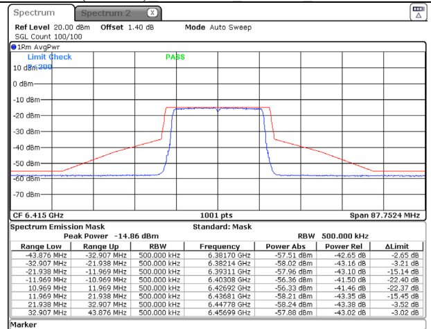
802.11ax (20MHz) 6415MHz Chain D NSS-1
