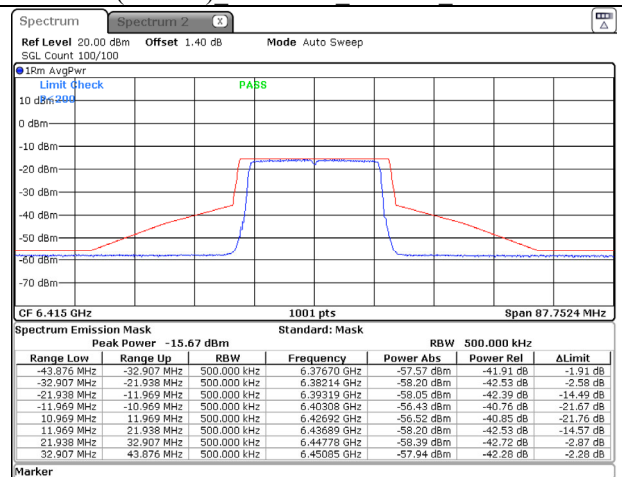
802.11ax (20MHz) 6415MHz Chain B NSS-1
