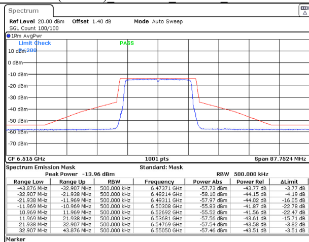
802.11ax (20MHz) 6515MHz Chain A NSS-1
