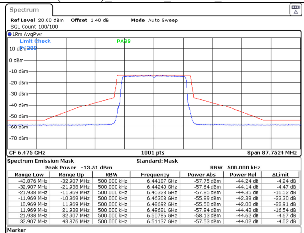
802.11ax (20MHz) 6475MHz Chain B NSS-1
