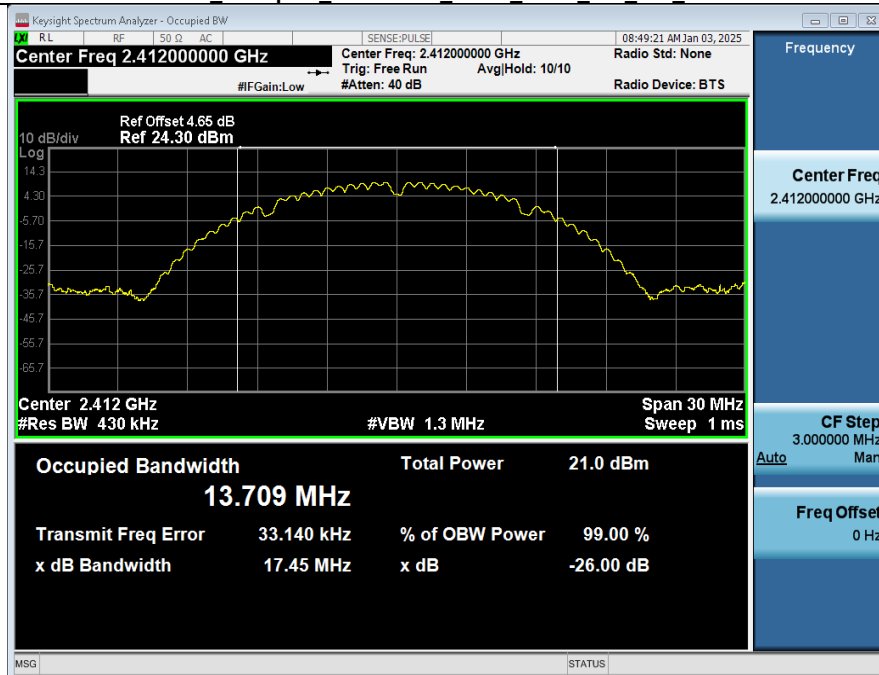
99% Occupied Bandwidth NVNT ANT2 802_11b_2412
