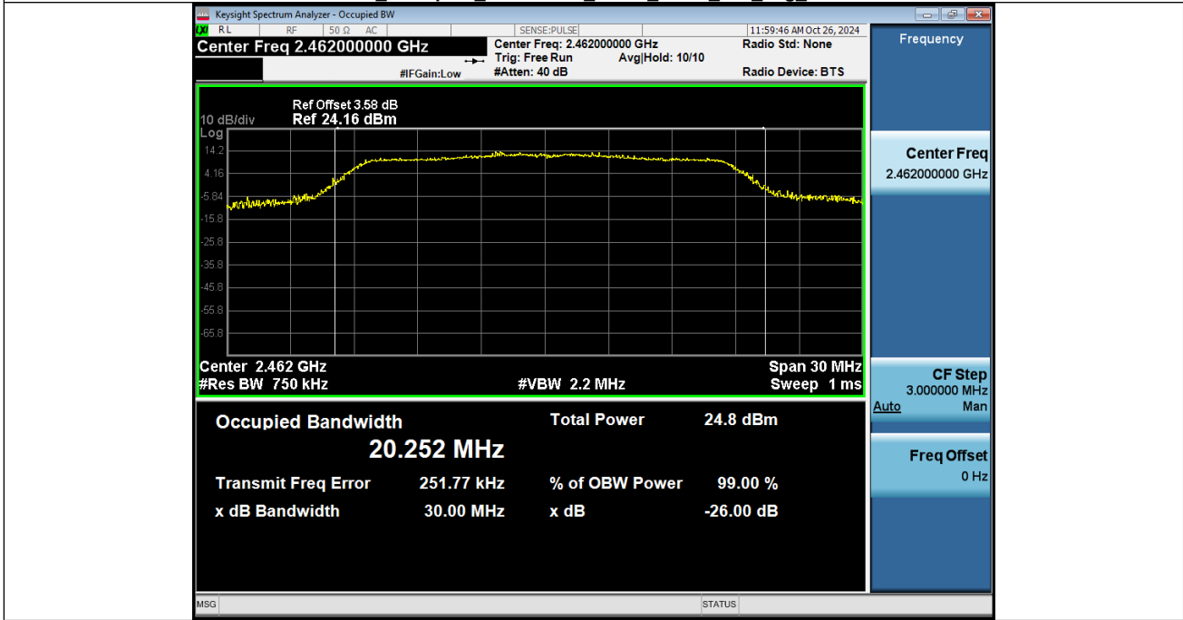
99%_Occupied_Bandwidth_NVNT_ANT2_802_11g_2462
