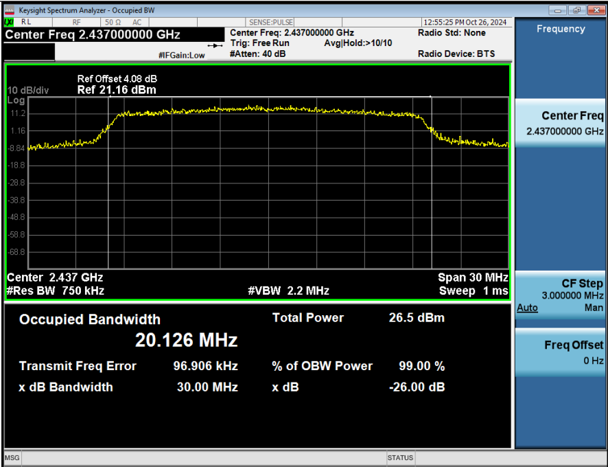
99% Occupied Bandwidth NVNT_ANT2_802_11ax(HE20)_2437
