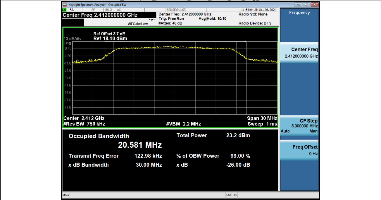
99%_Occupied_Bandwidth_NVNT_ANT2_802_11g_2412
