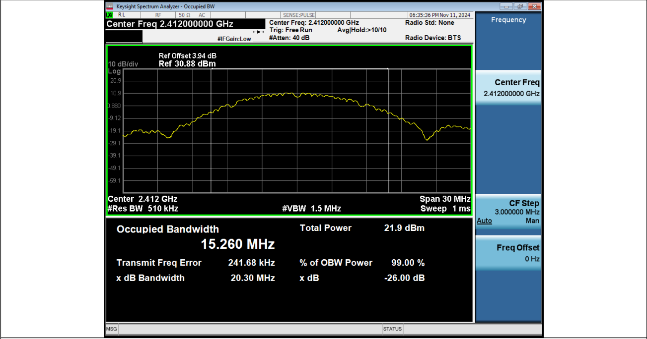
99% Occupied_Bandwidth_NVNT_ANT2_802_11b_2412
