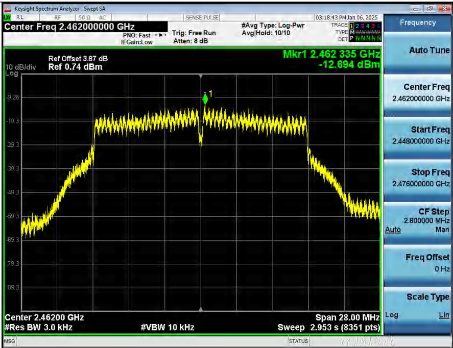
Power_Spectral_Density_NVNT_ANT2_802_11g_2462
