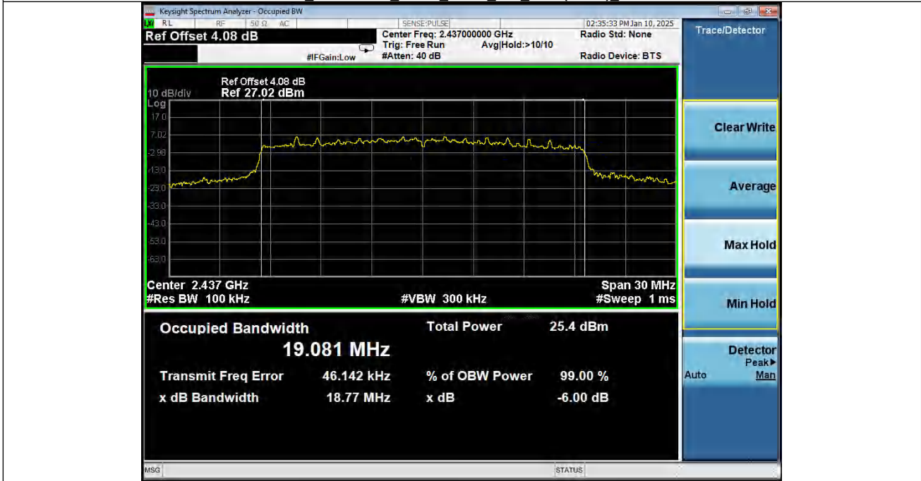
-6dB_Bandwidth_NVNT_ANT2_802_11ax(HE20)_2437
