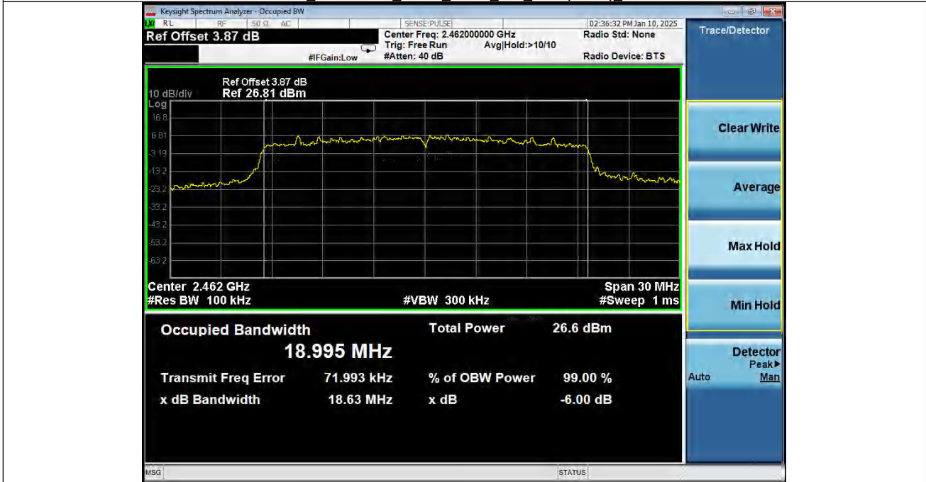
-6dB_Bandwidth_NVNT_ANT2_802_11ax(HE20)_2462
