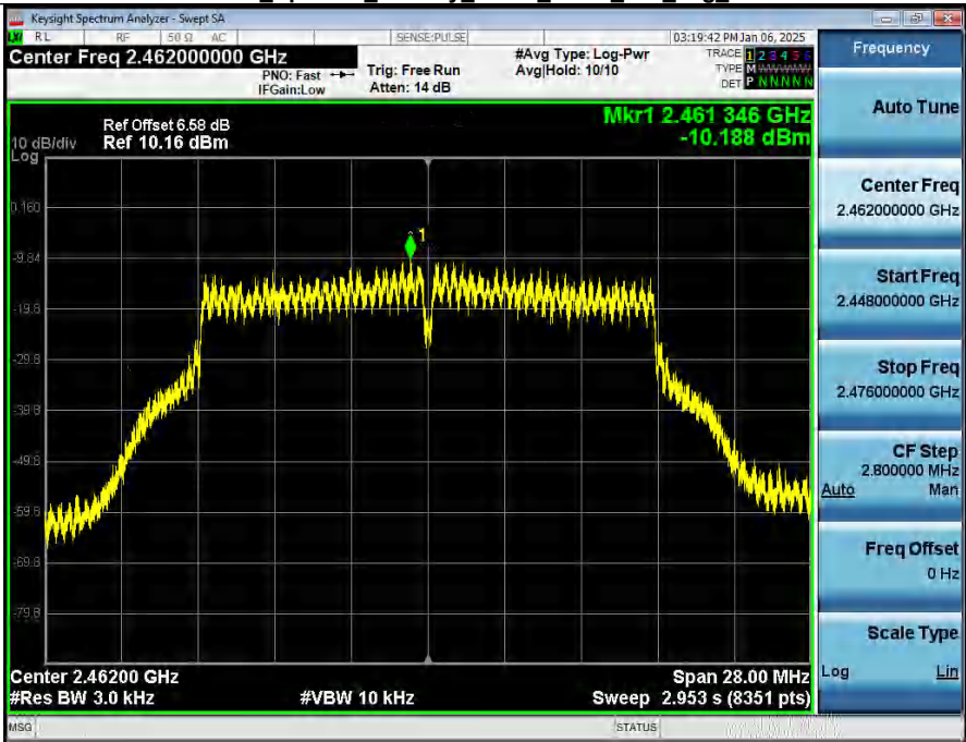
Power_Spectral_Density_NVNT_ANT2_802_11g_2462
