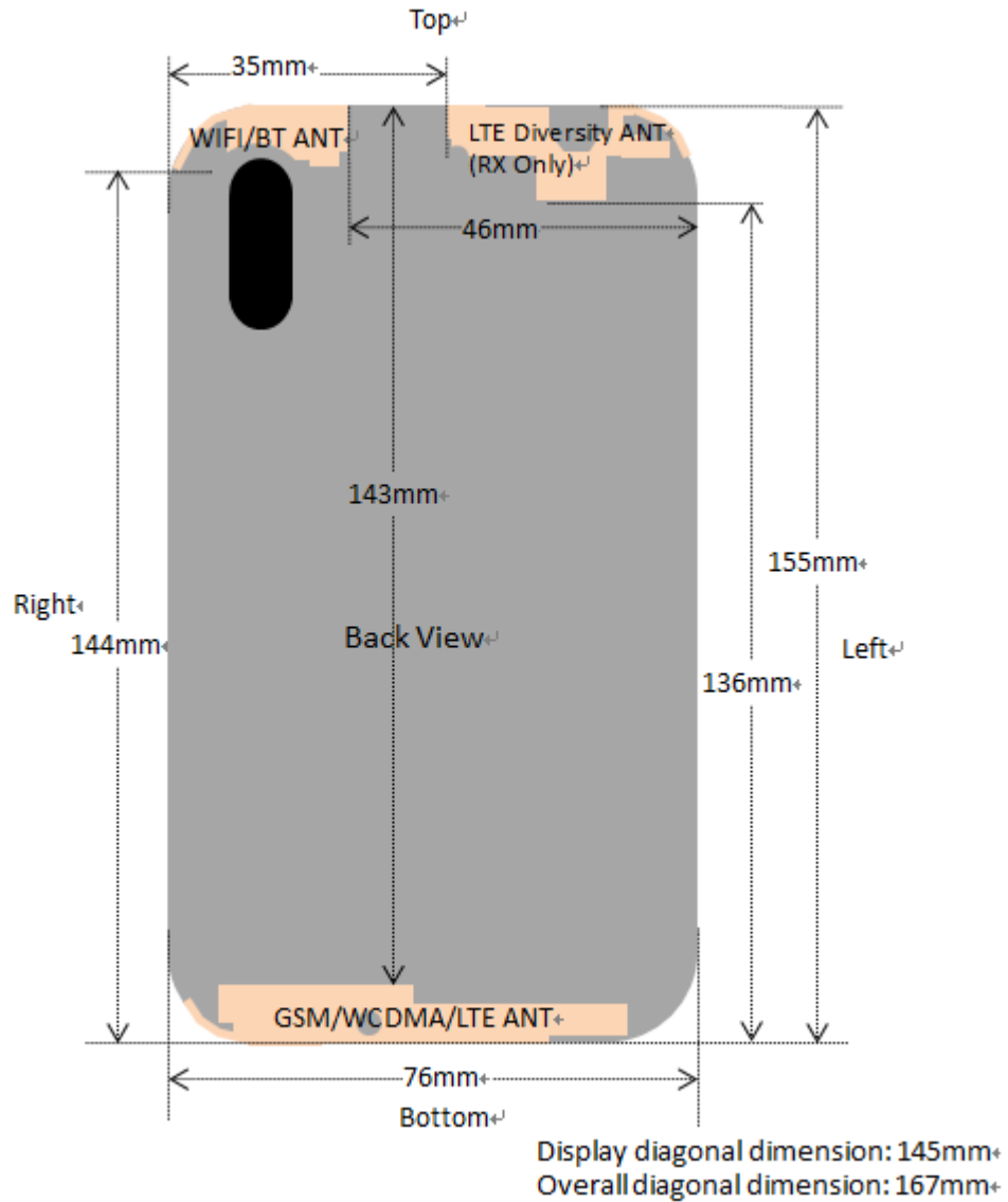
Fig.14.1 EUT Antenna Locations
