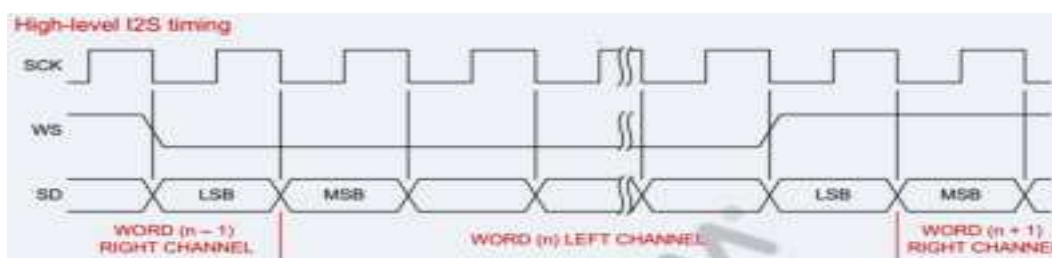
Figure 20: I2S timing
