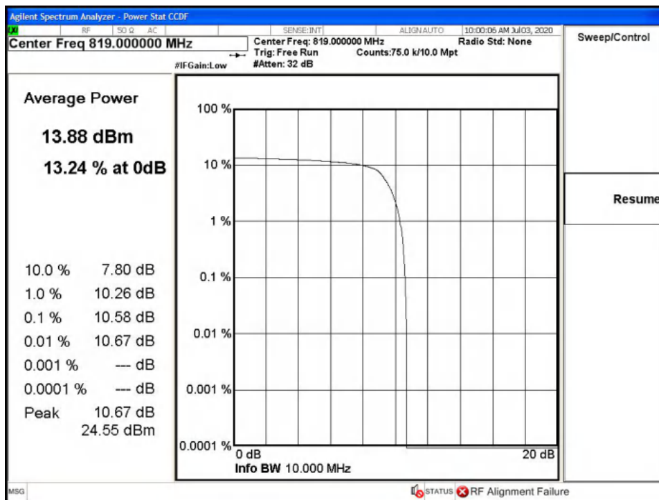
Band26-CH26740-819MHz-3MHz Bandwidth-QPSK
