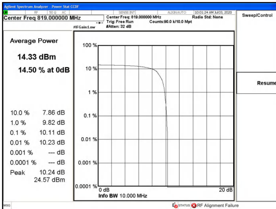
Band26-CH26740-819MHz-10MHz Bandwidth-16QAM
