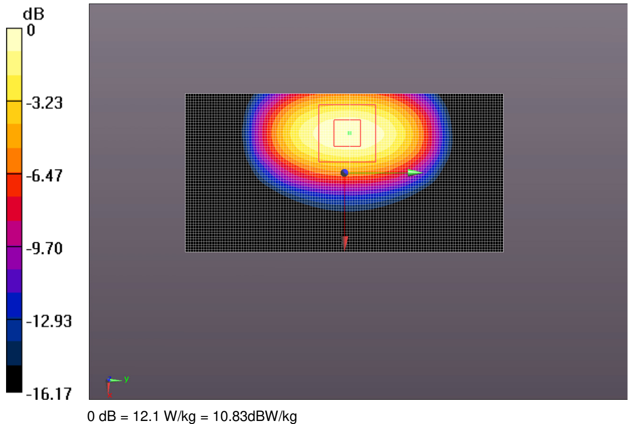
Fig.B.16 validation 1800MHz 250mW
