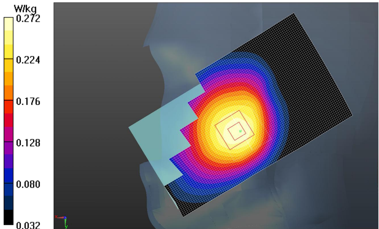
Fig.15 LTE Band 12
