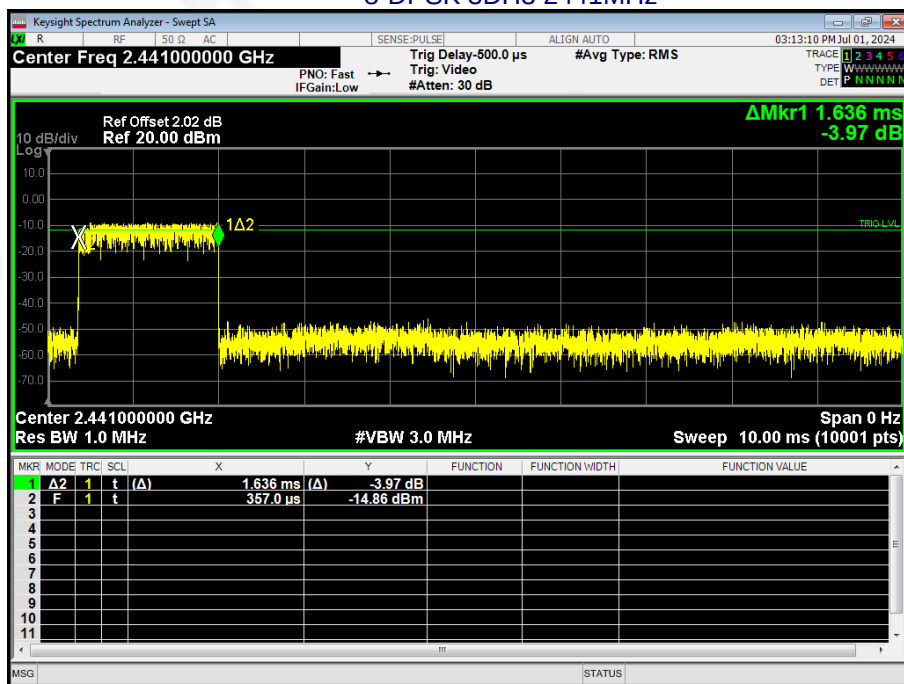
8-DPSK 3DH3 2441MHz
