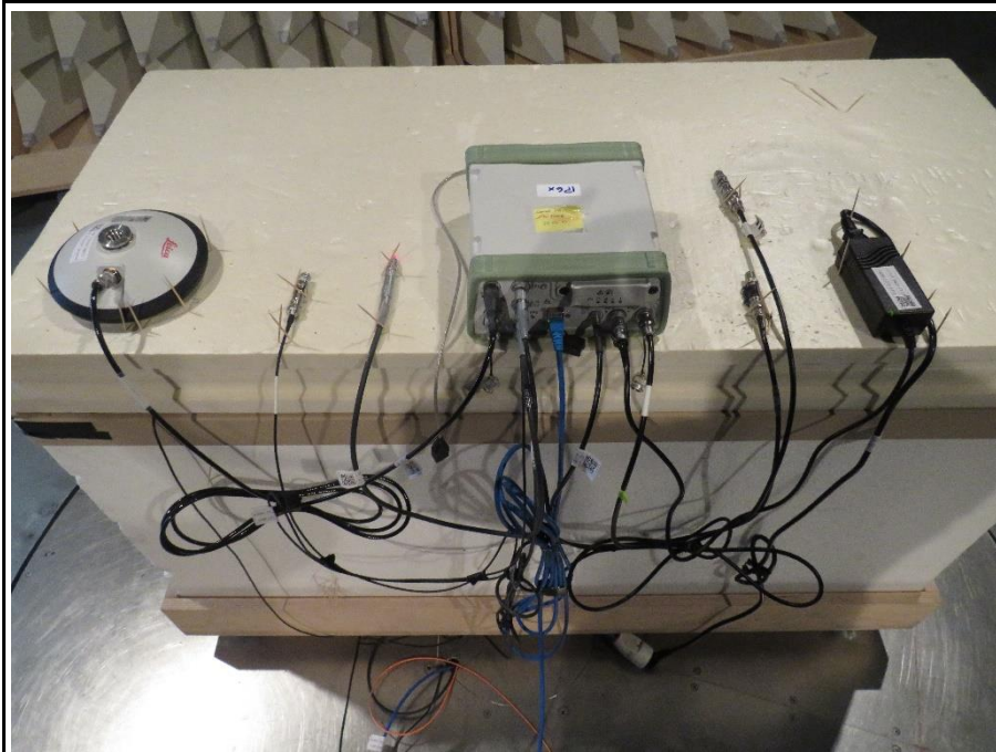
Test setup top view assembly
