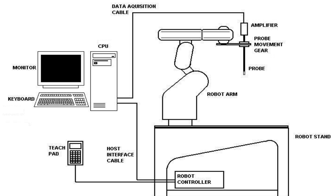
Figure 1: Schematic diagram of the SAR measurement system
