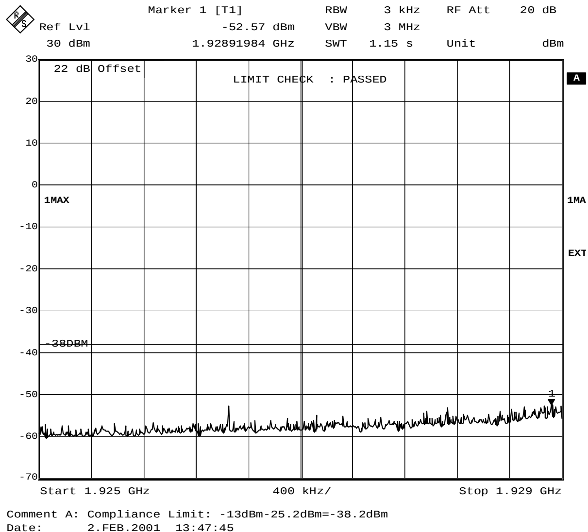
Fig. 10 – Spurious emissions in the frequency range 1925 MHz – 1929 MHz. Limit: -13dBm-25.2dB=-38.2dBm
