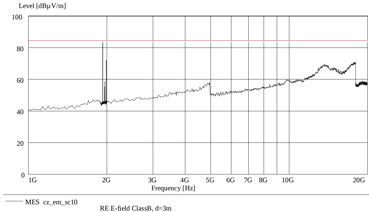
Fig. 33 – Radiated Emission 1GHz – 20 GHz.
