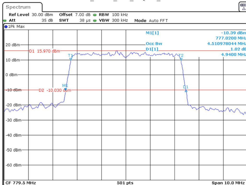
Band 13_5 MHz_Low_16QAM_RB25#0
