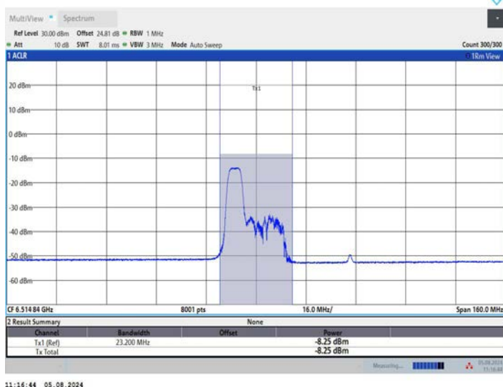
11AX80MIMO_Ant1_6545_106Tone_RU53
