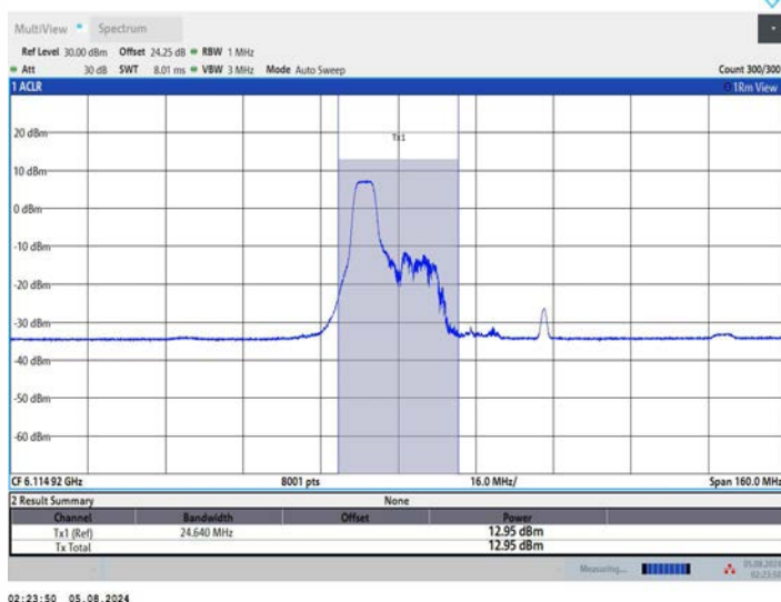
11AX80MIMO_Ant1_6145_106Tone_RU53
