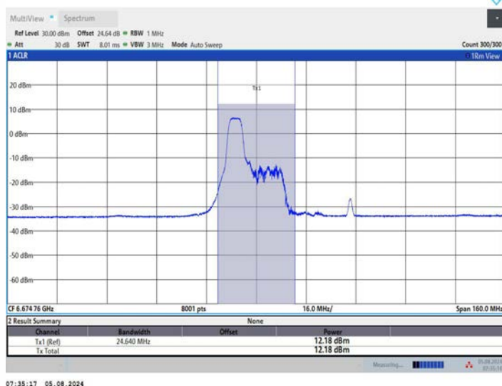
11AX80MIMO_Ant1_6705_106Tone_RU53
