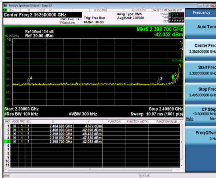
ZIGBEE_Ant1_Low_2405
