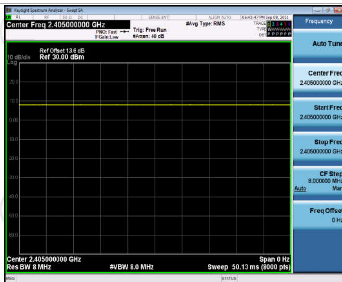
ZIGBEE_Ant1_2405
