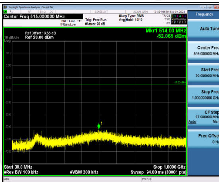
ZIGBEE_Ant1_2440_30~1000
