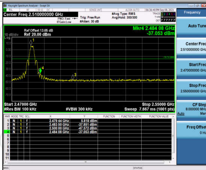
ZIGBEE_Ant1_High_2480
