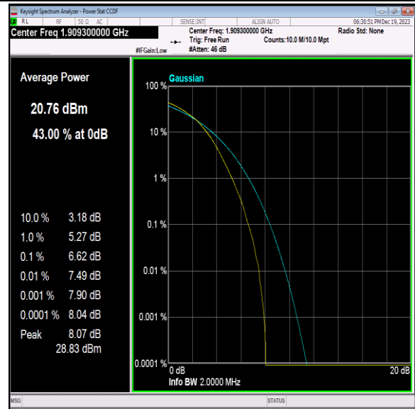
Band2-1.4MHz-64QAM-19193-6RB#0-PASS
