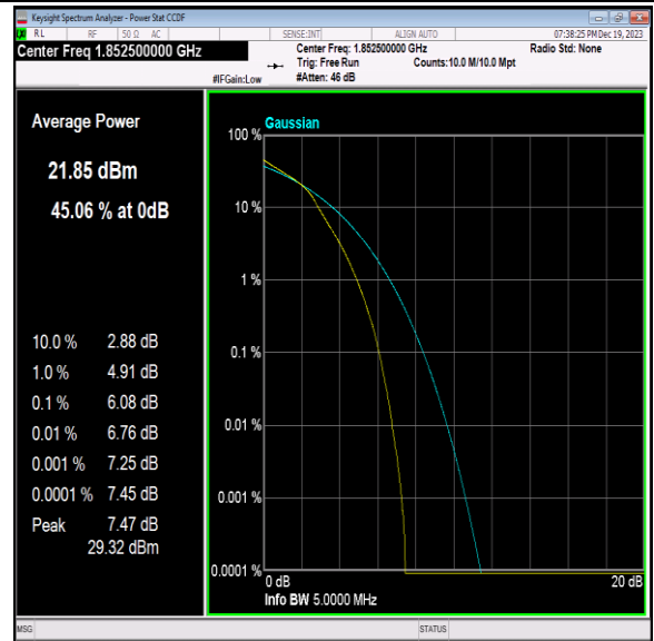
Band2-5MHz-16QAM-18625-25RB#0-PASS
