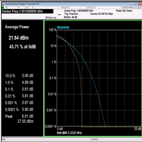
Band2-3MHz-64QAM-18615-1RB#0-PASS
