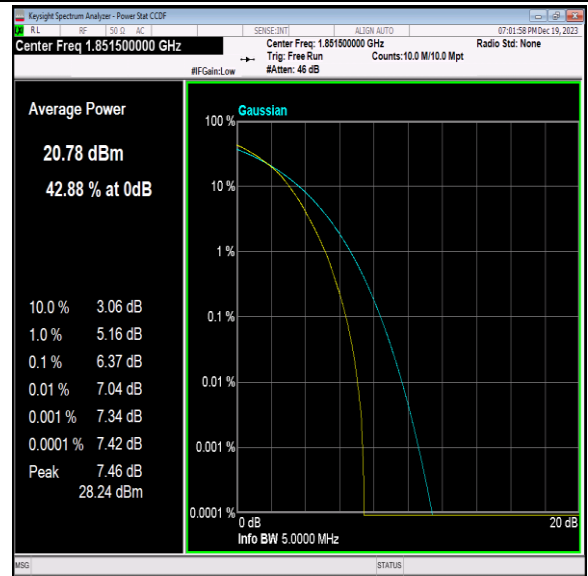
Band2-3MHz-64QAM-18615-15RB#0-PASS
