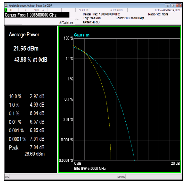
Band2-3MHz-16QAM-19185-15RB#0-PASS
