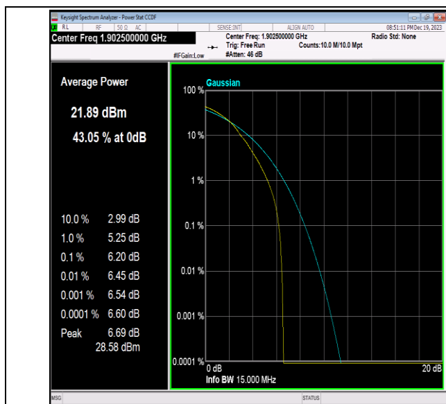
Band2-15MHz-64QAM-19125-1RB#0-PASS
