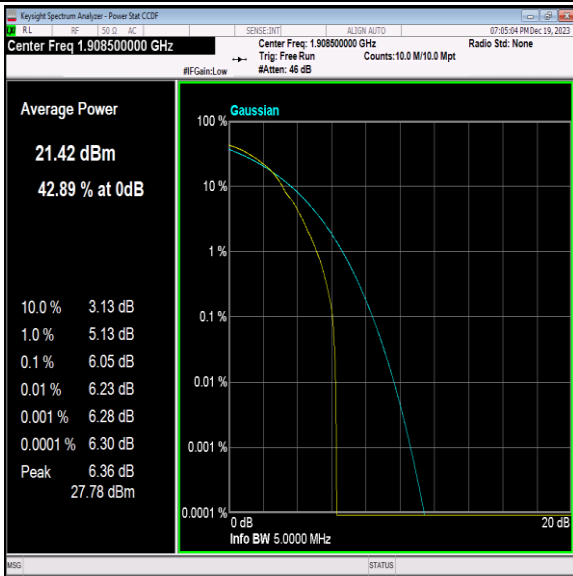
Band2-3MHz-64QAM-19185-1RB#0-PASS
