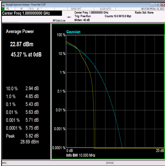
Band2-10MHz-16QAM-18900-1RB#0-PASS
