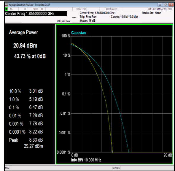
Band2-10MHz-64QAM-18650-50RB#0-PASS
