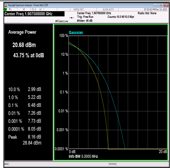
Band2-5MHz-64QAM-19175-25RB#0-PASS
