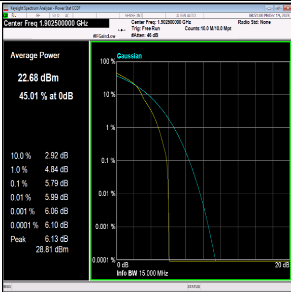
Band2-15MHz-16QAM-19125-1RB#0-PASS
