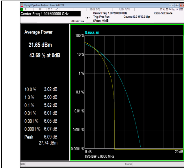
Band2-5MHz-64QAM-19175-1RB#0-PASS
