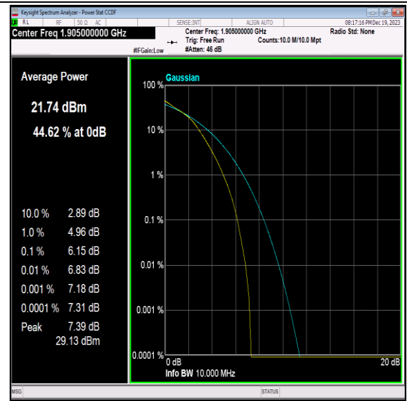
Band2-10MHz-16QAM-19150-50RB#0-PASS
