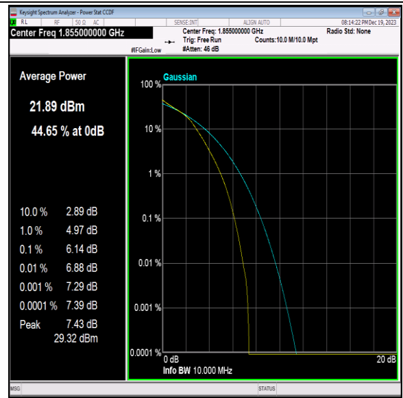
Band2-10MHz-16QAM-18650-50RB#0-PASS
