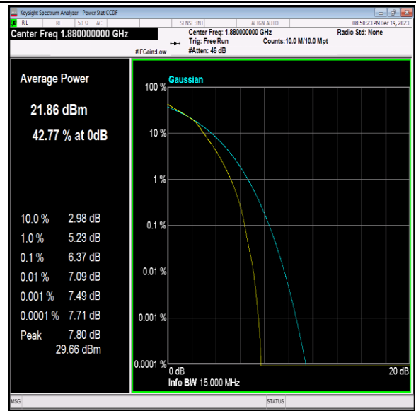
Band2-15MHz-16QAM-18900-75RB#0-PASS
