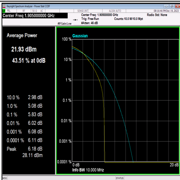
Band2-10MHz-64QAM-19150-1RB#0-PASS
