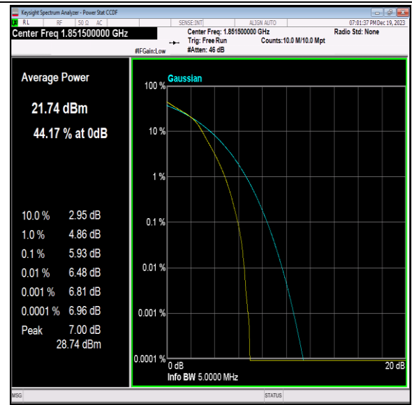
Band2-3MHz-16QAM-18615-15RB#0-PASS
