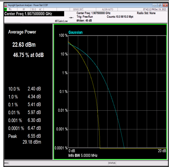
Band2-5MHz-QPSK-19175-25RB#0-PASS
