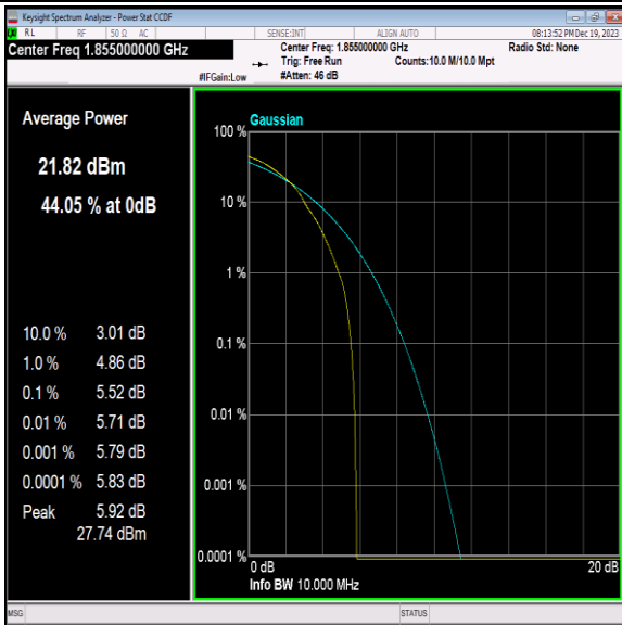
Band2-10MHz-64QAM-18650-1RB#0-PASS
