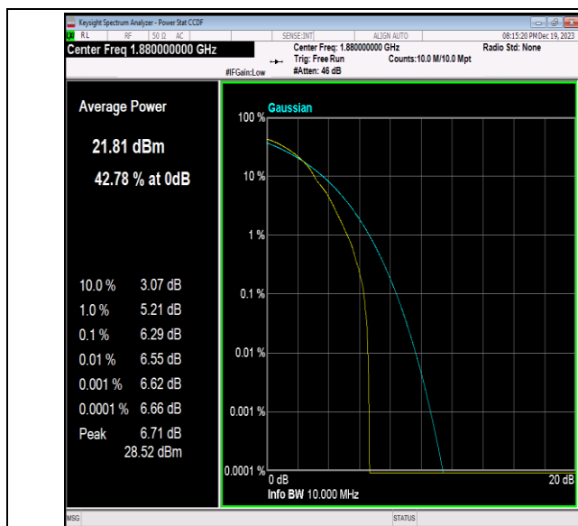
Band2-10MHz-64QAM-18900-1RB#0-PASS
