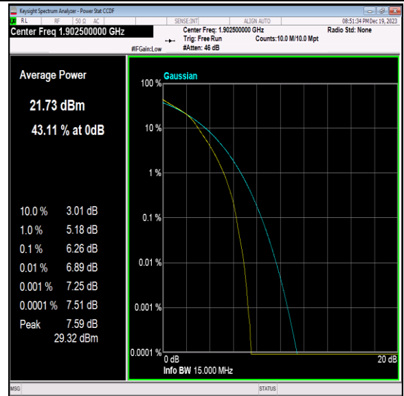
Band2-15MHz-16QAM-19125-75RB#0-PASS
