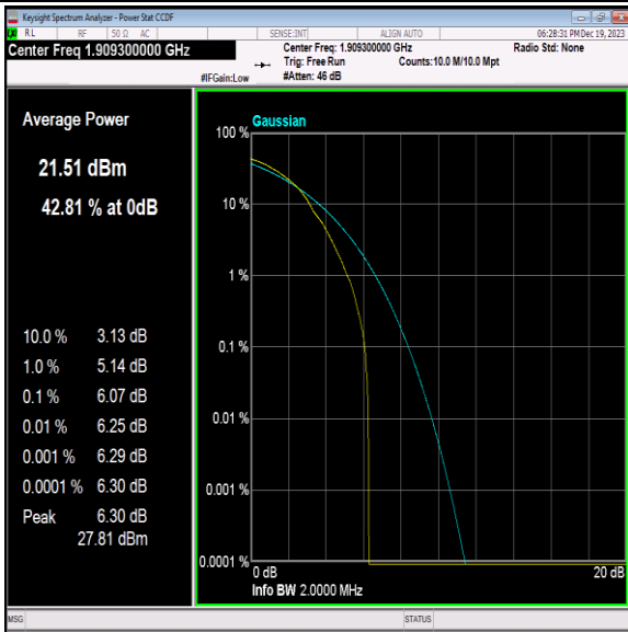
Band2-1.4MHz-64QAM-19193-1RB#0-PASS
