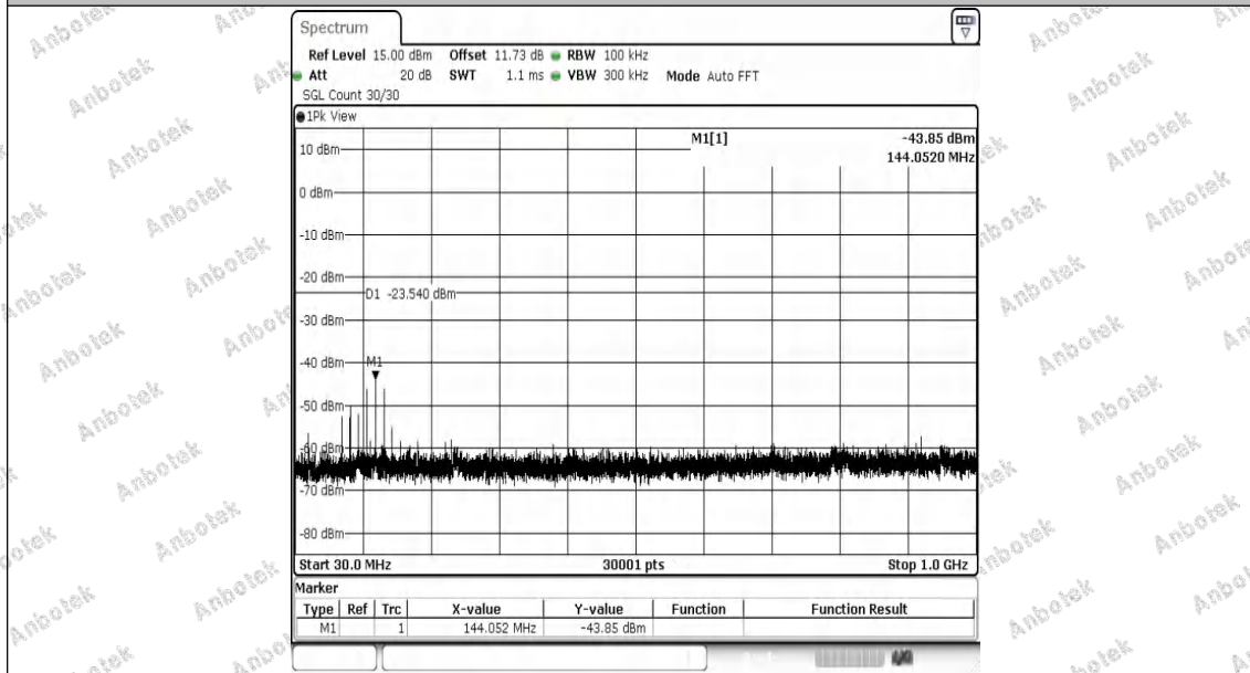
3DH5-Ant1-2480-30~1000-PASS
