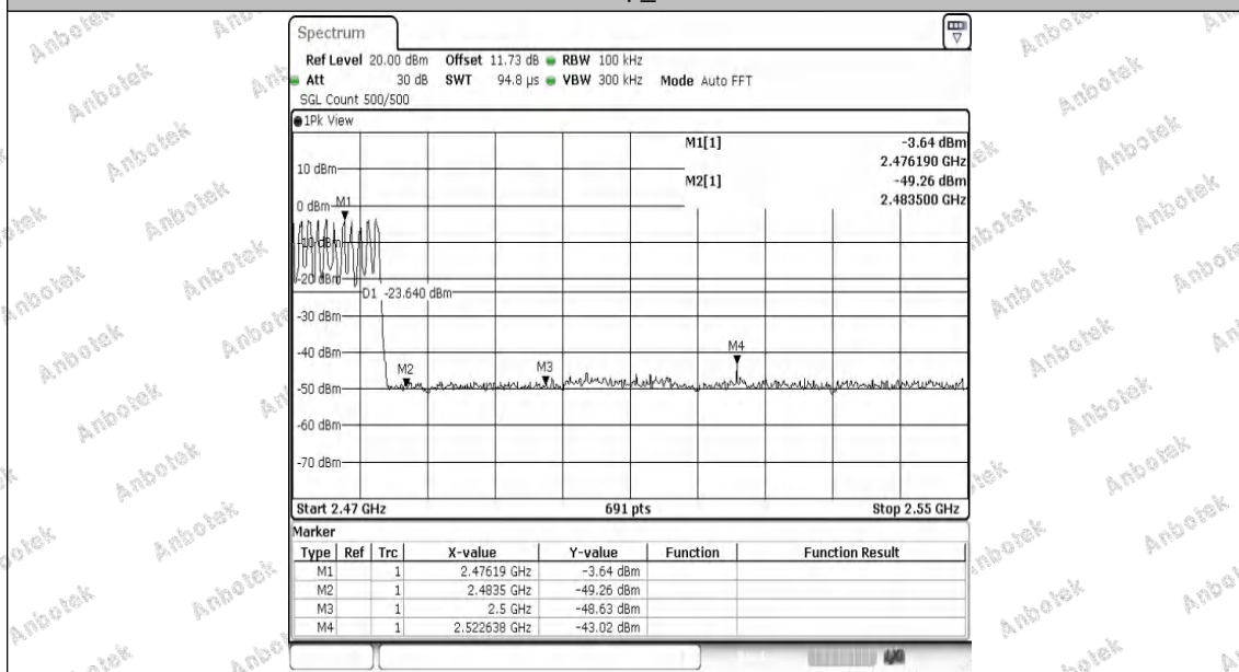
DH5-Ant1-Hop_2480-PASS
