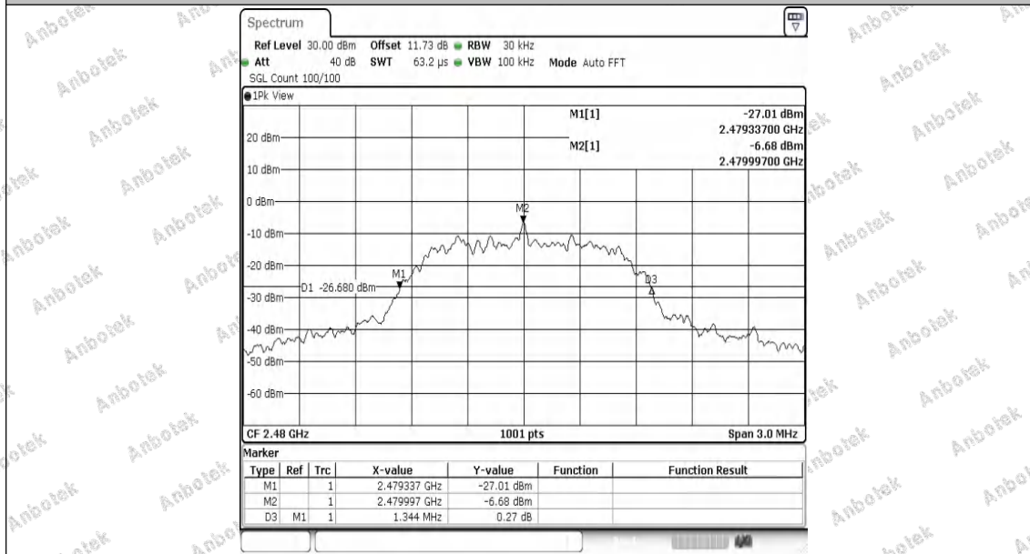
2DH5-Ant1-2480
