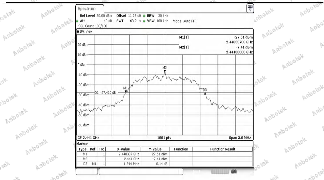
2DH5-Ant1-2441
