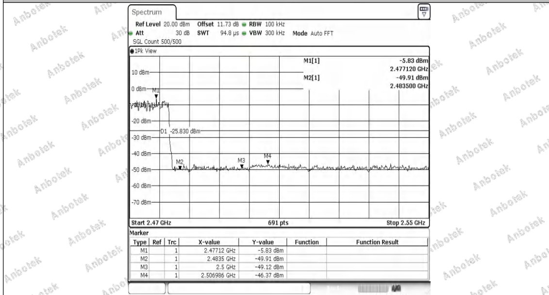
2DH5-Ant1-Hop_2480-PASS
