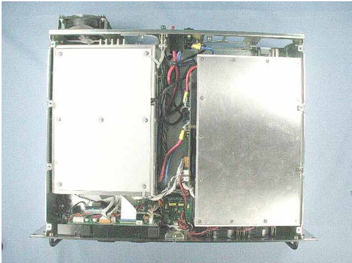
Inside of EUT with inner covers
