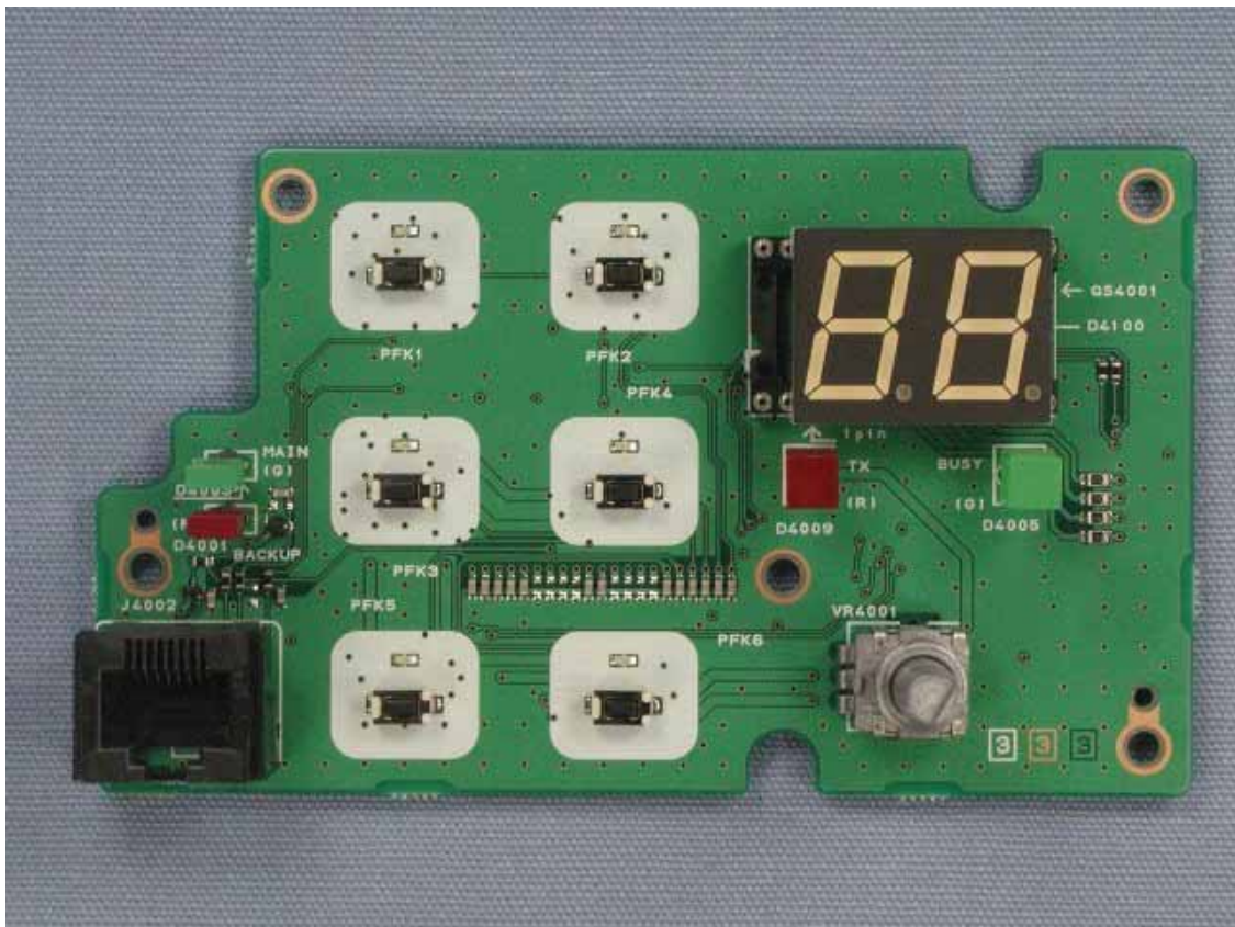
Side-A of PANEL-UNIT
