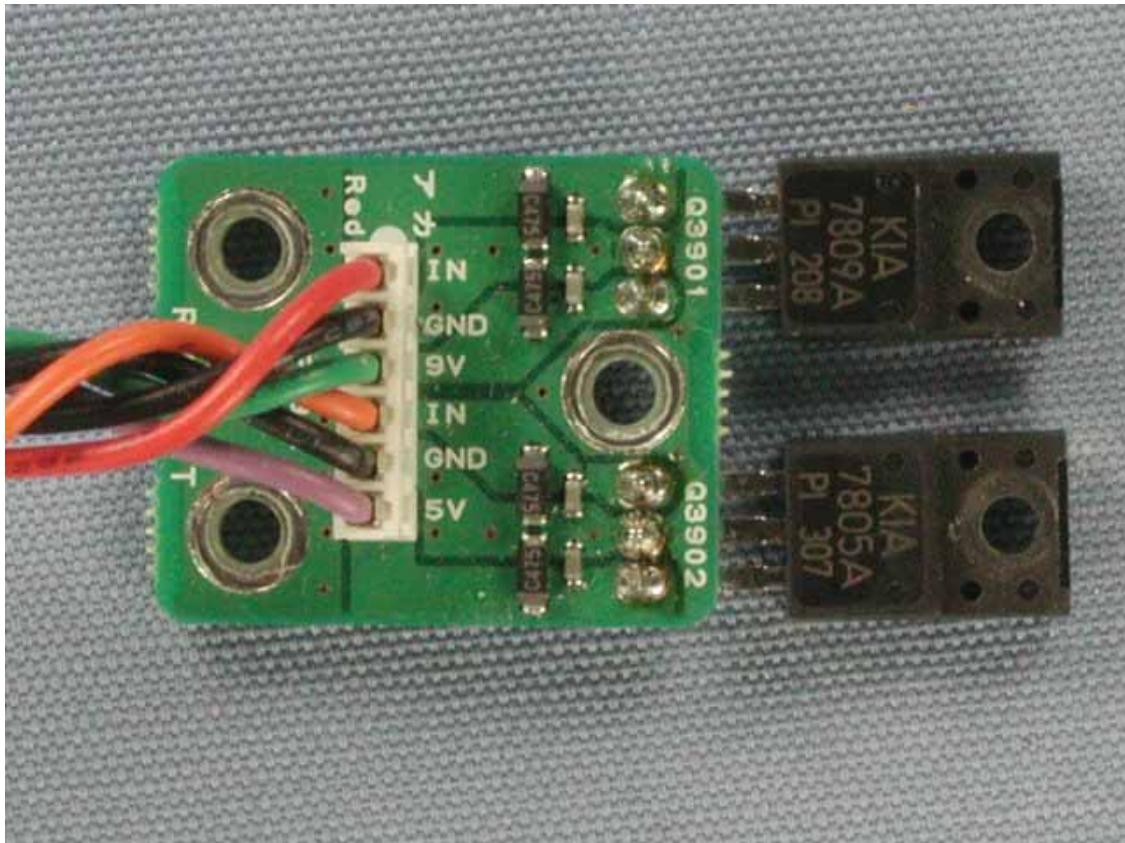
Side-A of REG-UNIT
