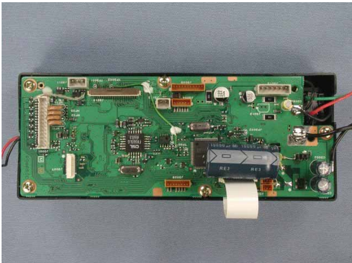
Inside of sub-panel with PWB (1)
