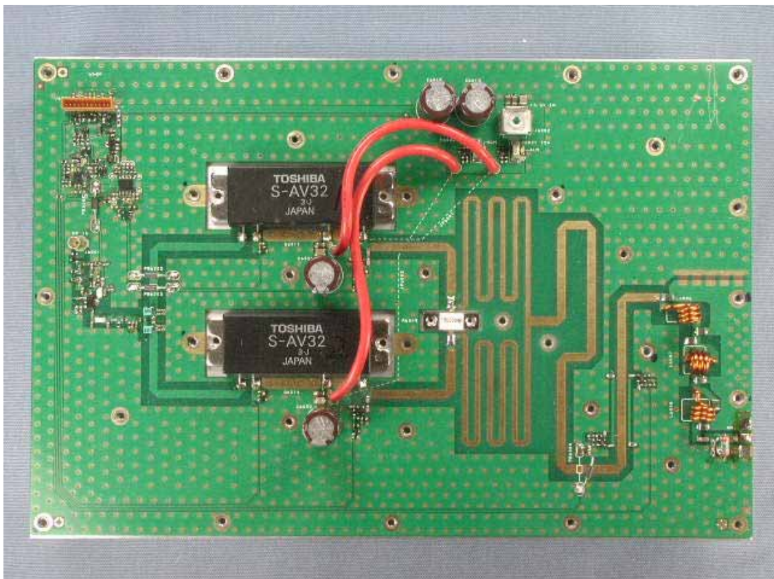
Side-A of 100W-PA-UNIT
