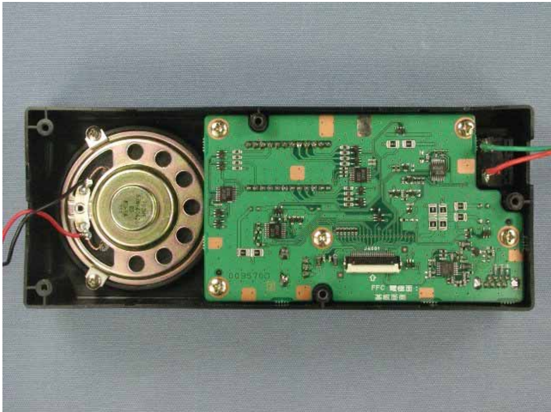
Inside of sub-panel with PWB (2)
