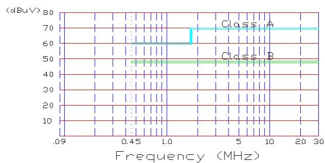
Fig. 11. Line-Conducted Limits
