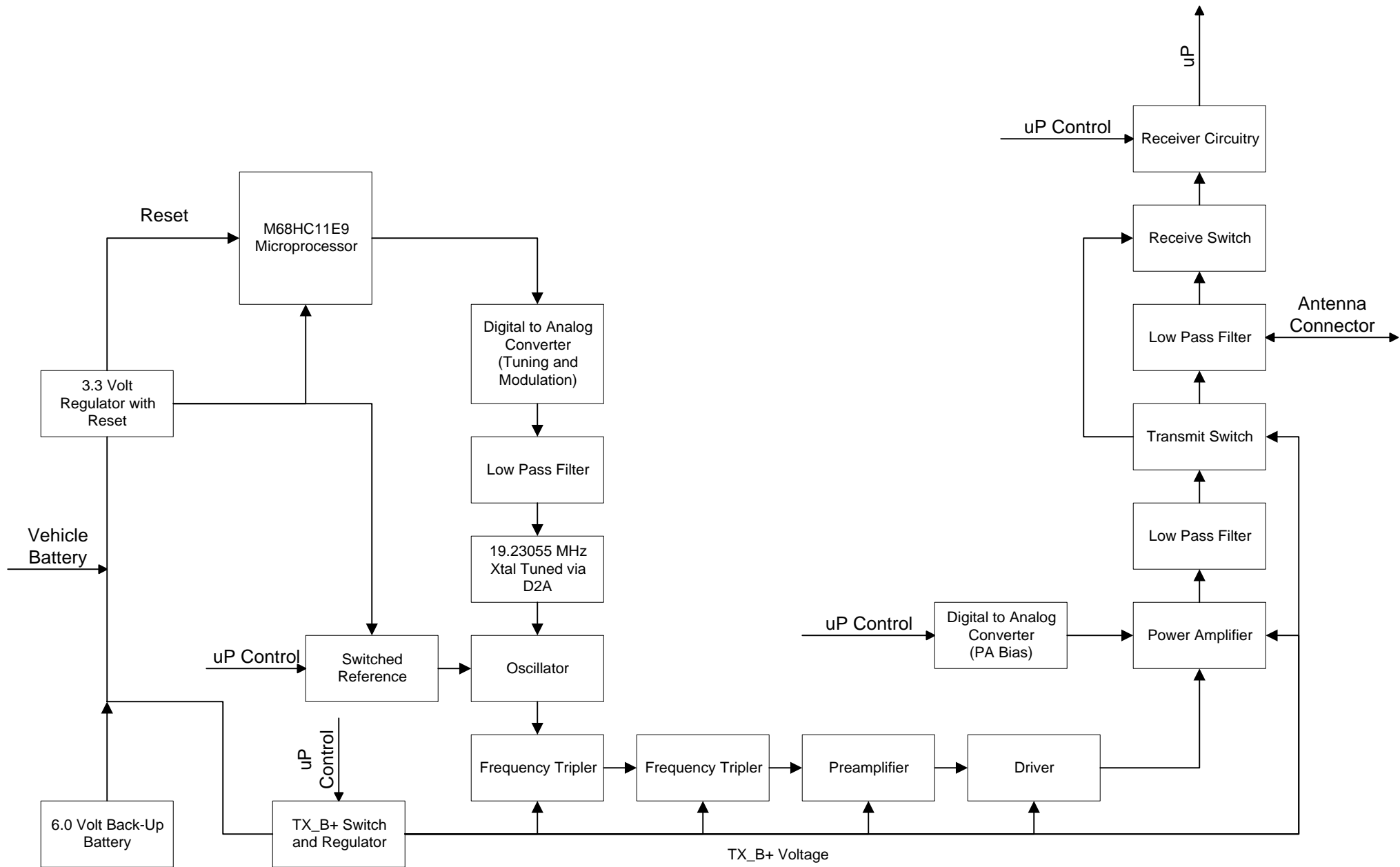
LoJack III Uplink Transmitter Block Diagram
