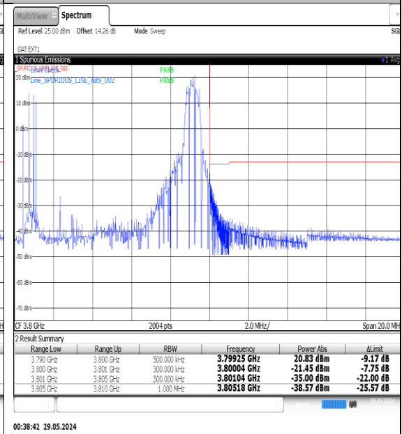
NTNV-N78-3700-3800-PC3-30-10-H-DFT-QPSK- Edge_1RB_Right-Ant1-PASS
