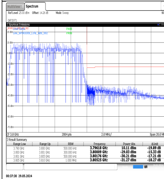
NTNV-N78-3700-3800-PC3-30-10-H-DFT-QPSK- Outer_Full-Ant1-PASS
