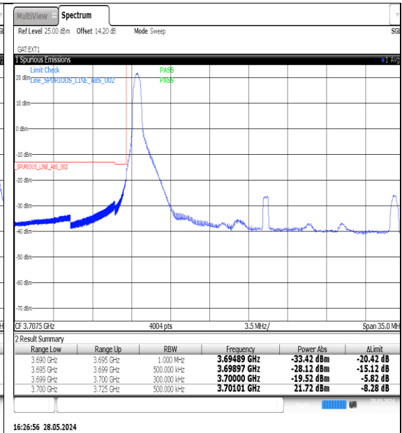
NTNV-N77-3700-3980-PC3-30-25-L-DFT-QPSK- Edge_1RB_Left-Ant1-PASS
