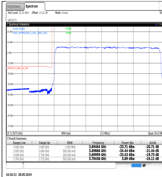
NTNV-N77-3700-3980-PC3-30-25-L-DFT-QPSK- Outer_Full-Ant1-PASS
