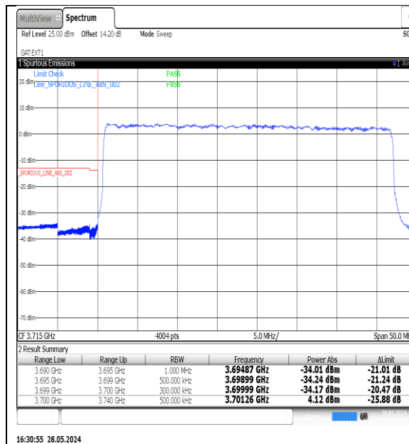
NTNV-N77-3700-3980-PC3-30-40-L-DFT-QPSK- Outer Full-Ant1-PASS
