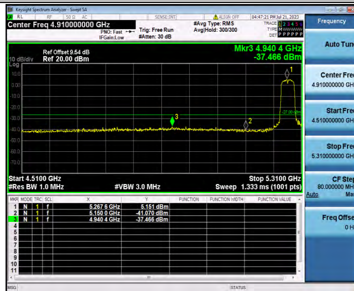
11AC40SISO_Ant2_Low_5270
