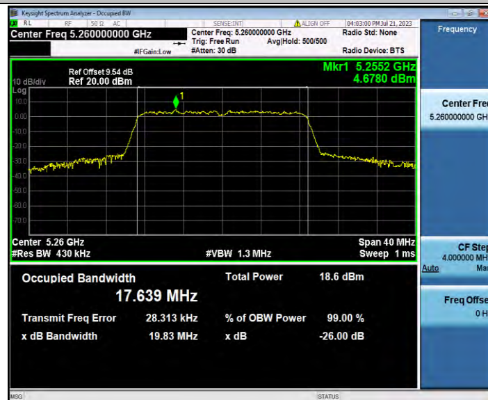
11AC20SISO_Ant2_5260
