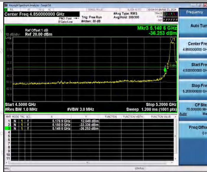
11A-CDD_Ant2_Low_5180
