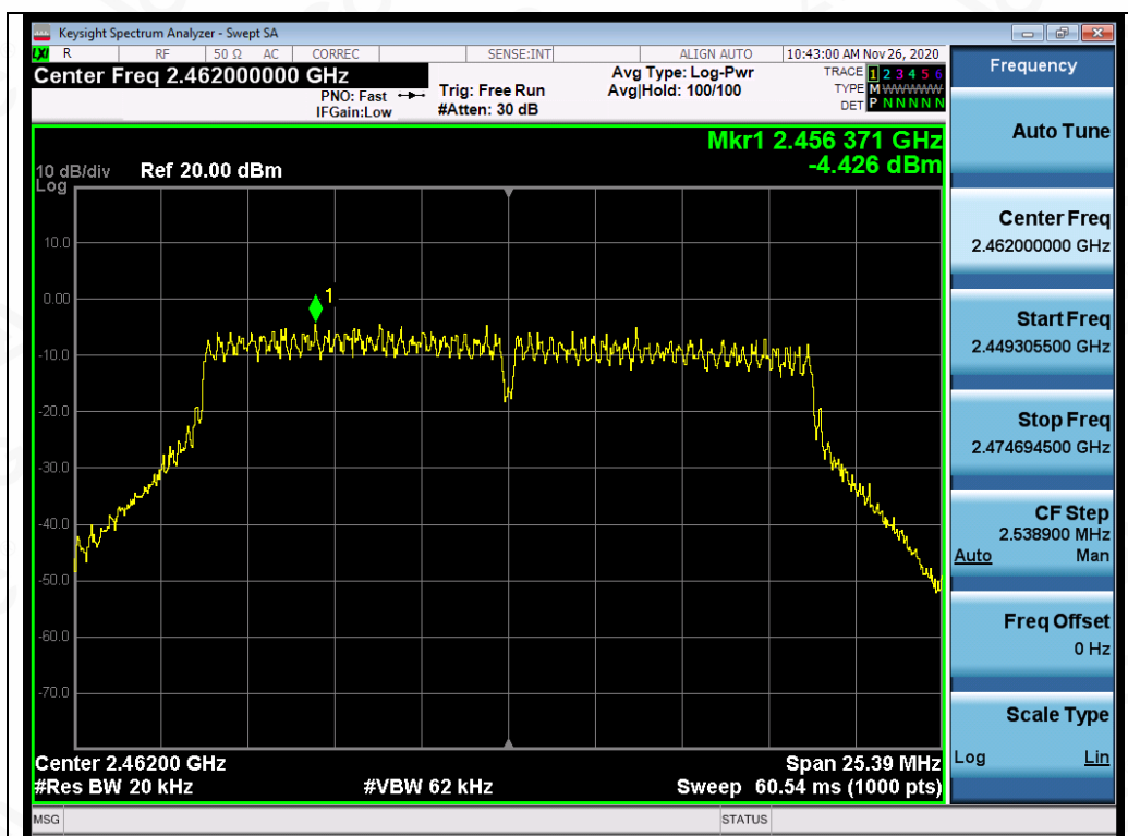
Test_Graph_802.11n20_ANT1_2462_MCS0_PSD
