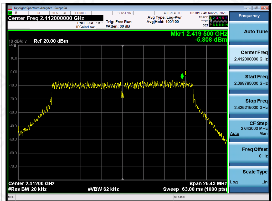
Test_Graph_802.11n20_ANT1_2412_MCS0_PSD
