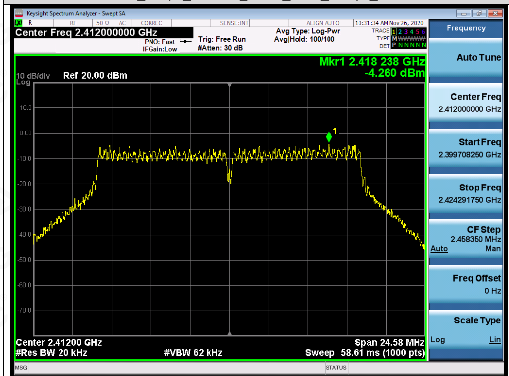
Test_Graph_802.11g_ANT1_2412_6Mbps_PSD
