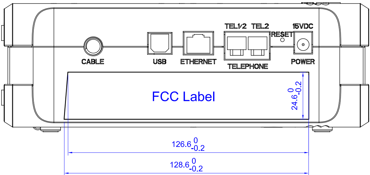
FCC Label Dimension
