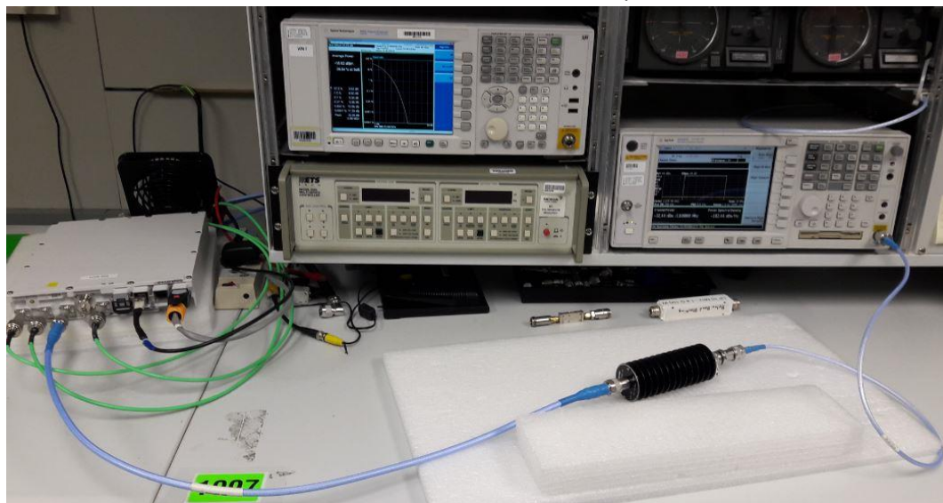
Photo of 20MHz to 3GHz Setup
