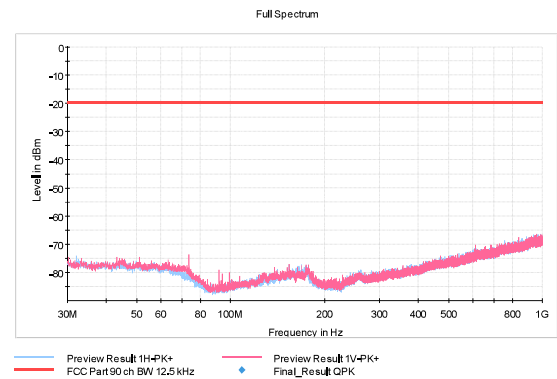
Figure 187: RX 469.5 MHz, 12.5 kHz, 4FSK
