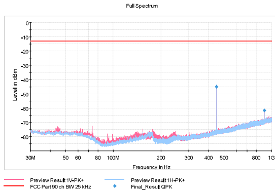
Figure 184: TX 450.5 MHz, 25 kHz, 4FSK
