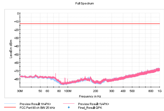
Figure 185: RX 450.5 MHz, 25 kHz, 4FSK
