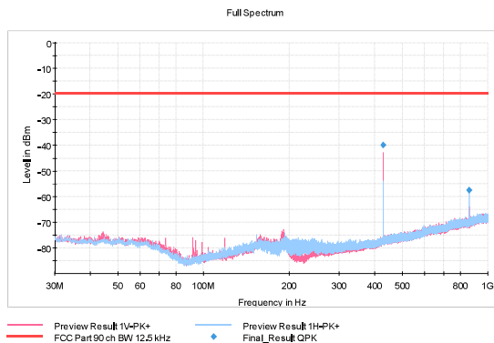
Figure 182: TX 429.5 MHz, 12.5 kHz, GMSK
