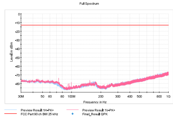
Figure 181: RX 410.0 MHz, 25 kHz, GMSK
