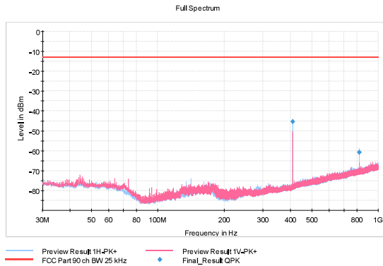
Figure 180: TX 410.0 MHz, 25 kHz, GMSK
