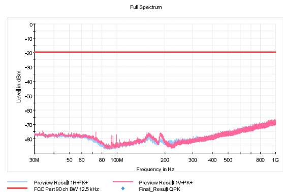
Figure 183: RX 429.5 MHz, 12.5 kHz, GMSK
