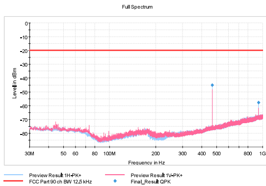
Figure 186: TX 469.5 MHz, 12.5 kHz, 4FSK
