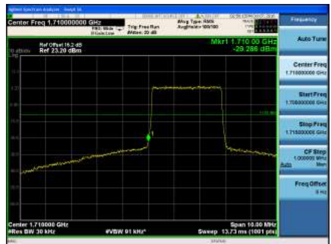
CH19975 (1712.5MHz) 16QAM Bandwidth 5MHz 25RB#0
