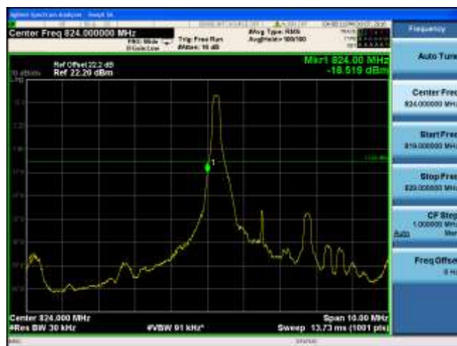
CH20415 (825.5MHz) 16QAM Bandwidth 3MHz 1RB#0
