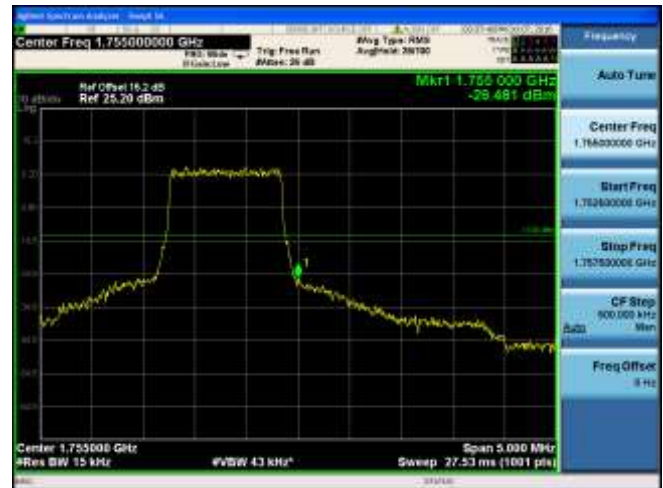
CH20385 (1753.5MHz) QPSK Bandwidth 3MHz 15RB#0
