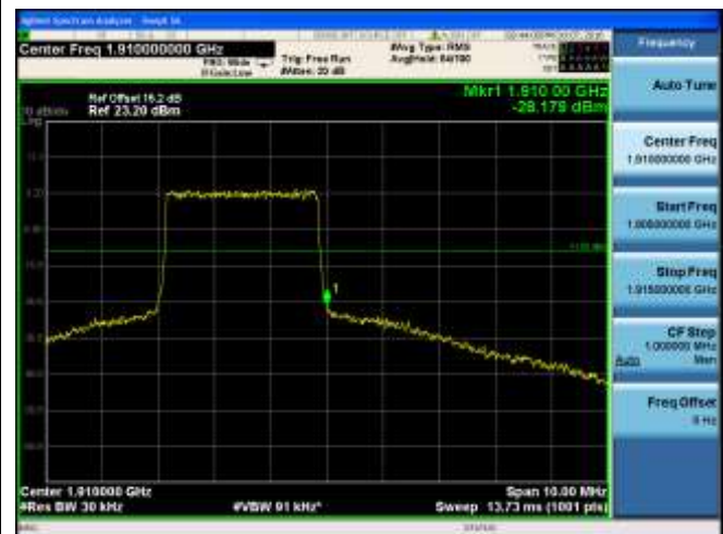
CH19175 (1907.5MHz) 16QAM Bandwidth 5MHz 25RB#0
