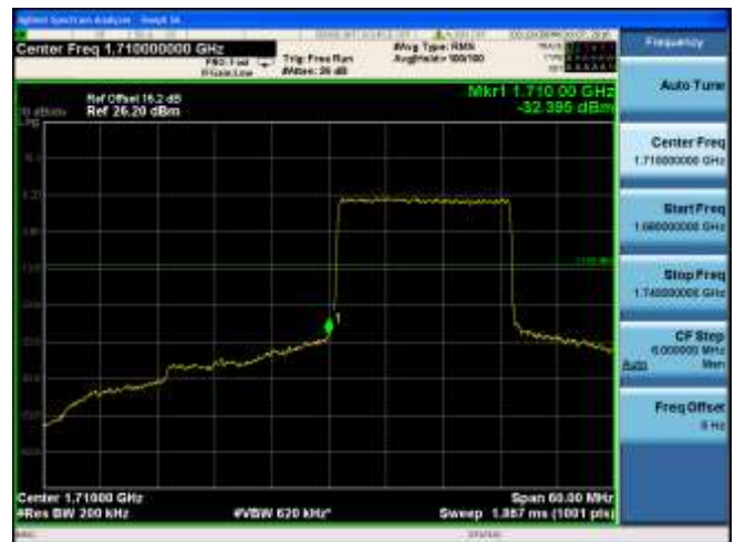
CH20050 (1720MHz) QPSK Bandwidth 20MHz 100RB#0
