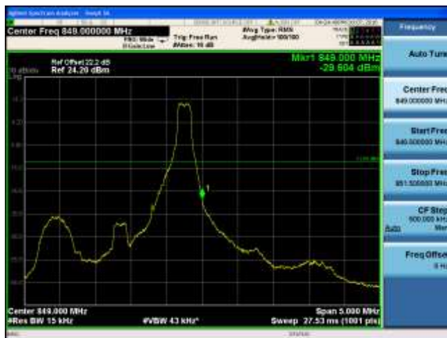
CH20635 (847.5MHz) 16QAM Bandwidth 3MHz 1RB#14
