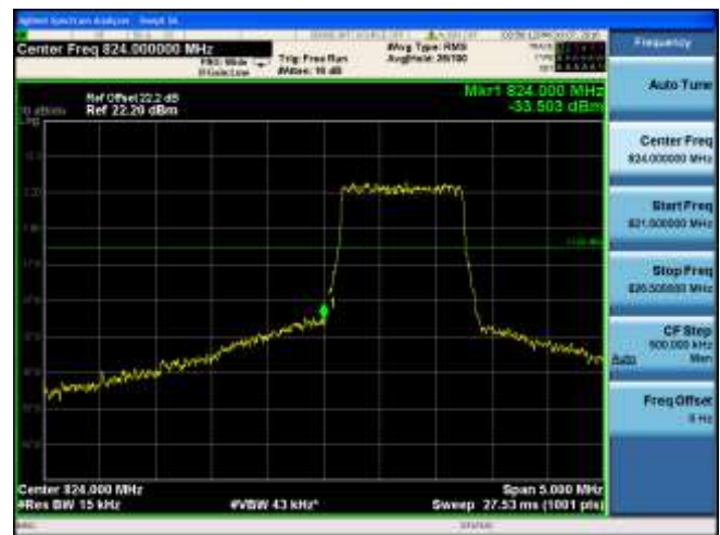
CH20415 (825.5MHz) 16QAM Bandwidth 3MHz 15RB#0
