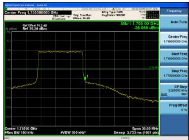
CH20325 (1747.5MHz) QPSK Bandwidth 15MHz 75RB#0
