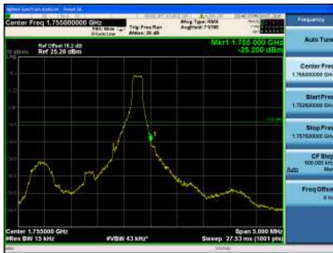
CH20385 (1753.5MHz) 16QAM Bandwidth 3MHz 1RB#14
