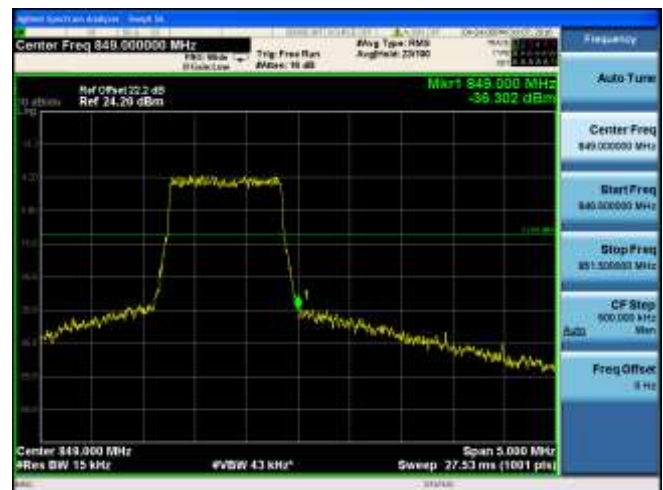
CH20635 (847.5MHz) 16QAM Bandwidth 3MHz 15RB#0
