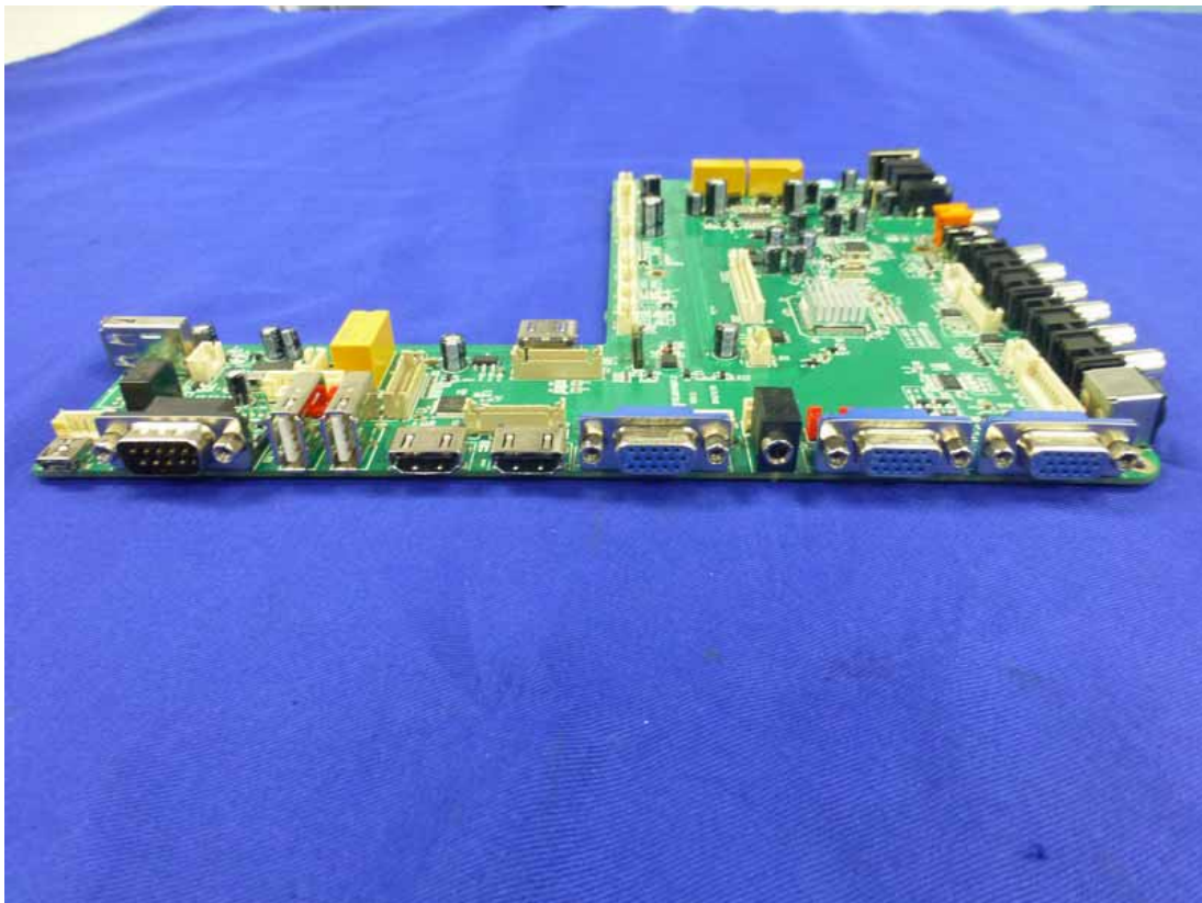
Figure 12 I/O Port of the Main Board
