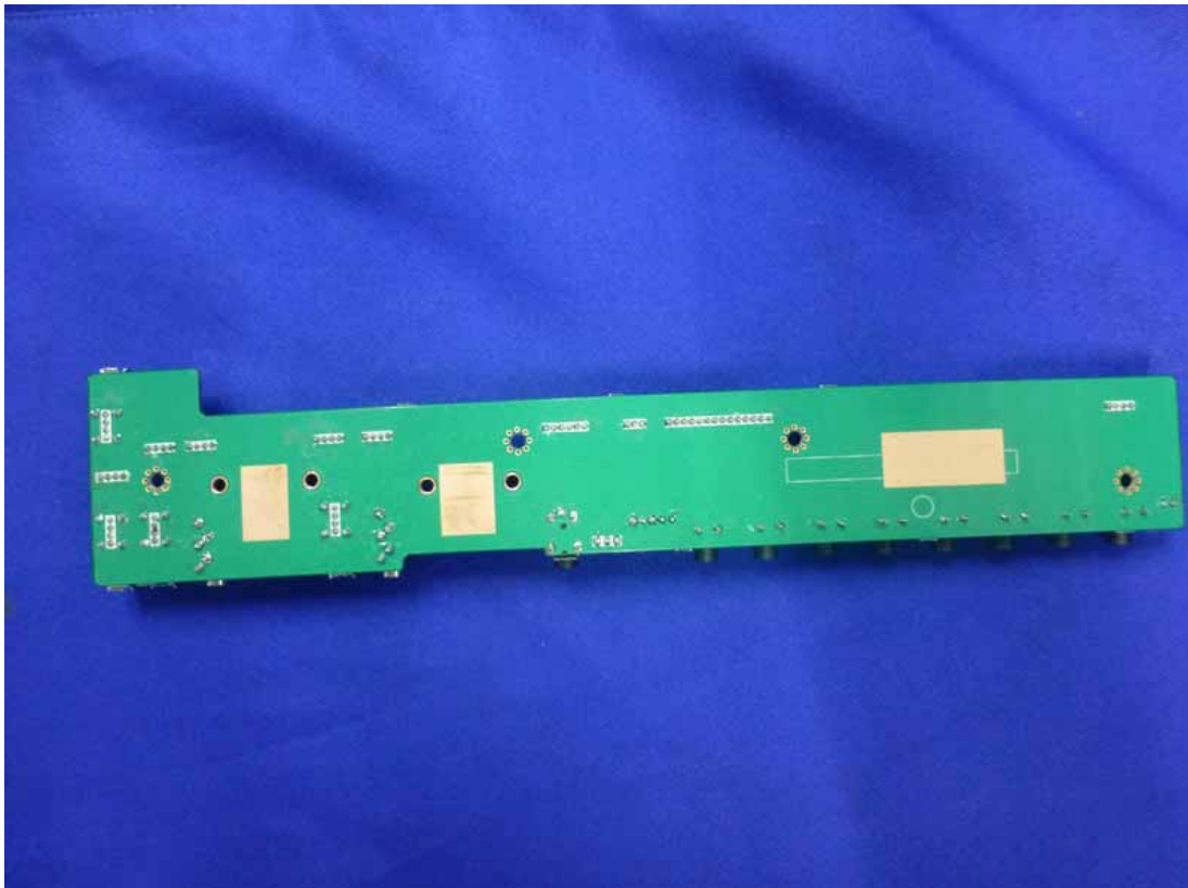
Figure 18 Backside of the Control Board
