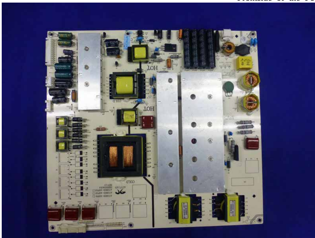
Figure 15 Frontside of the Power Board
