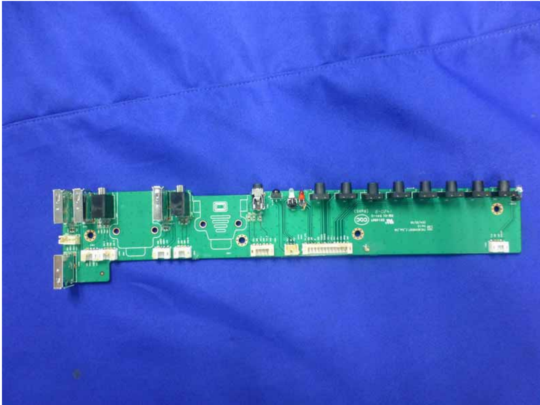
Figure 17 Front side of the Control Board
