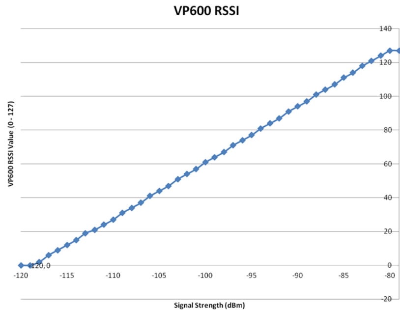
Figure 4.2 VP600 RSSI Curve
