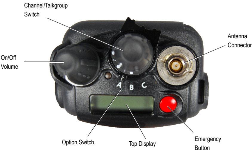
Figure 2.2 Top Panel Controls
