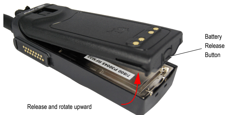
Figure 3.1 Battery Removal
