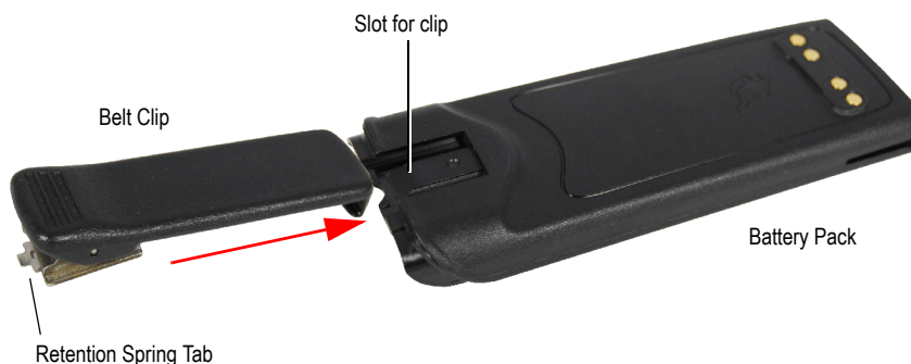
Figure 3.2 Belt clip Installation
